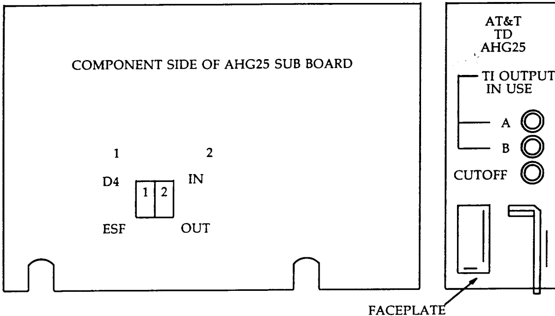
Figure 1. Location of Option Switches on AHG25 Timing Distributor Plug-In Unit
