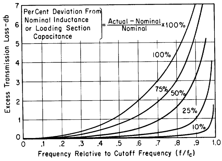
(b) EXCESS TRANSMISSION LOSS DUE TO LOADING COIL OR LOAD SPACING IRREGULARITIES
