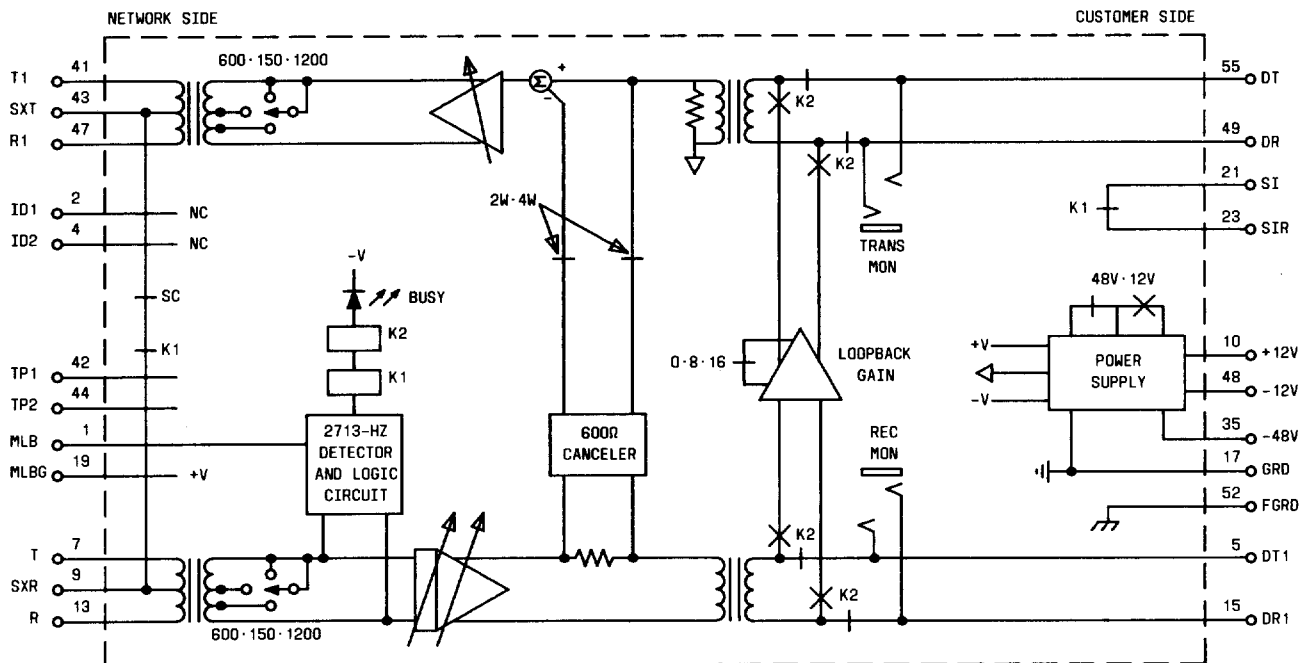
Fig. 1 — Block Diagram of BPT72
