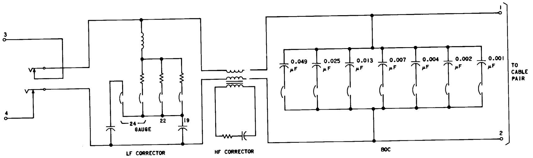
Fig. 2—837A Network—Schematic
