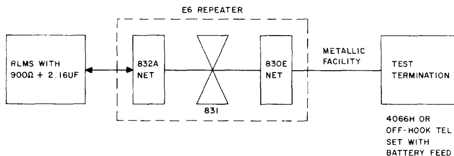
Fig. 2—Recommended Test Configuration
