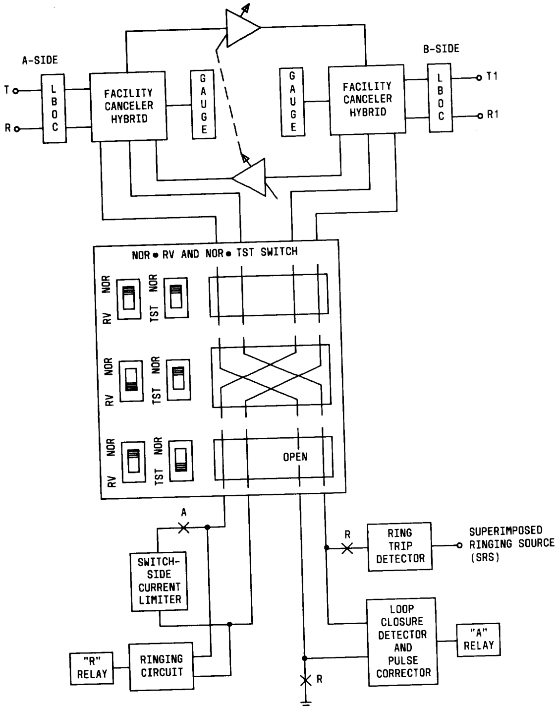
Fig. 2—Block Diagram of J99343GC Combined Function Unit
