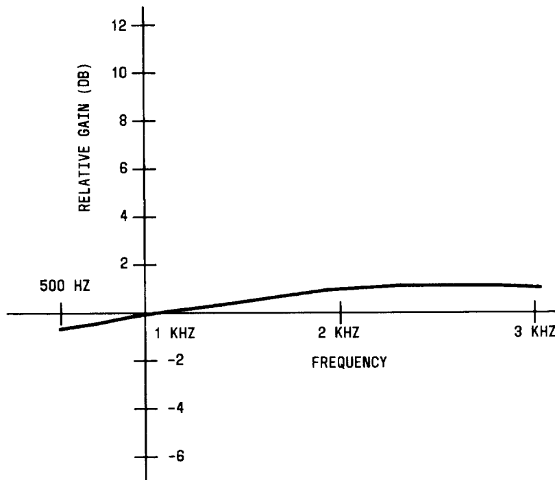
Fig. 3—Gain Frequency Response of J99343GC Combined Function Unit
