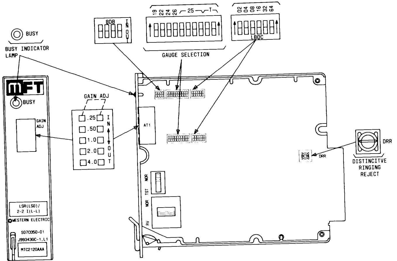
Fig. 1 — Pictorial of J99343GC Combined Function Unit
