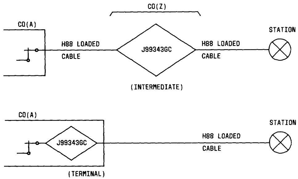
Fig. 6—Foreign Exchange Line Using J99343GC Combined Function Unit
