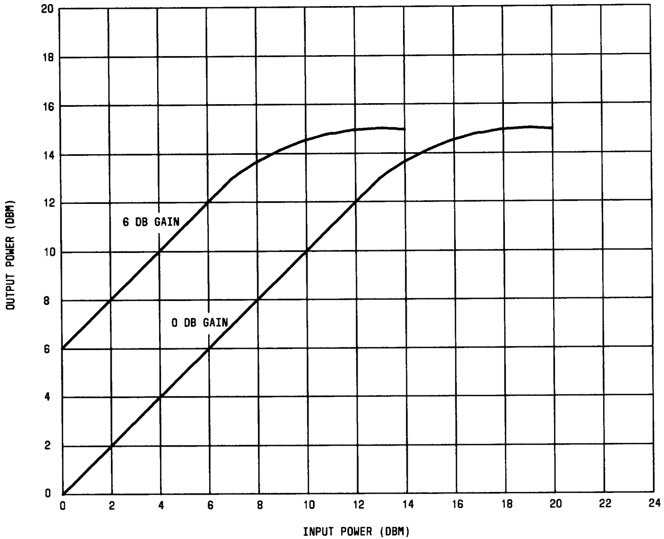
Fig. 5—Output Power Characteristic Curve
