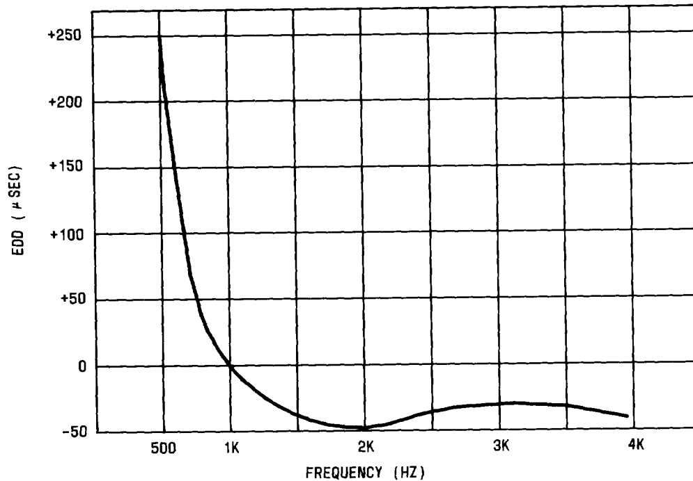
Fig. 4—Envelope Delay Distortion Curve
