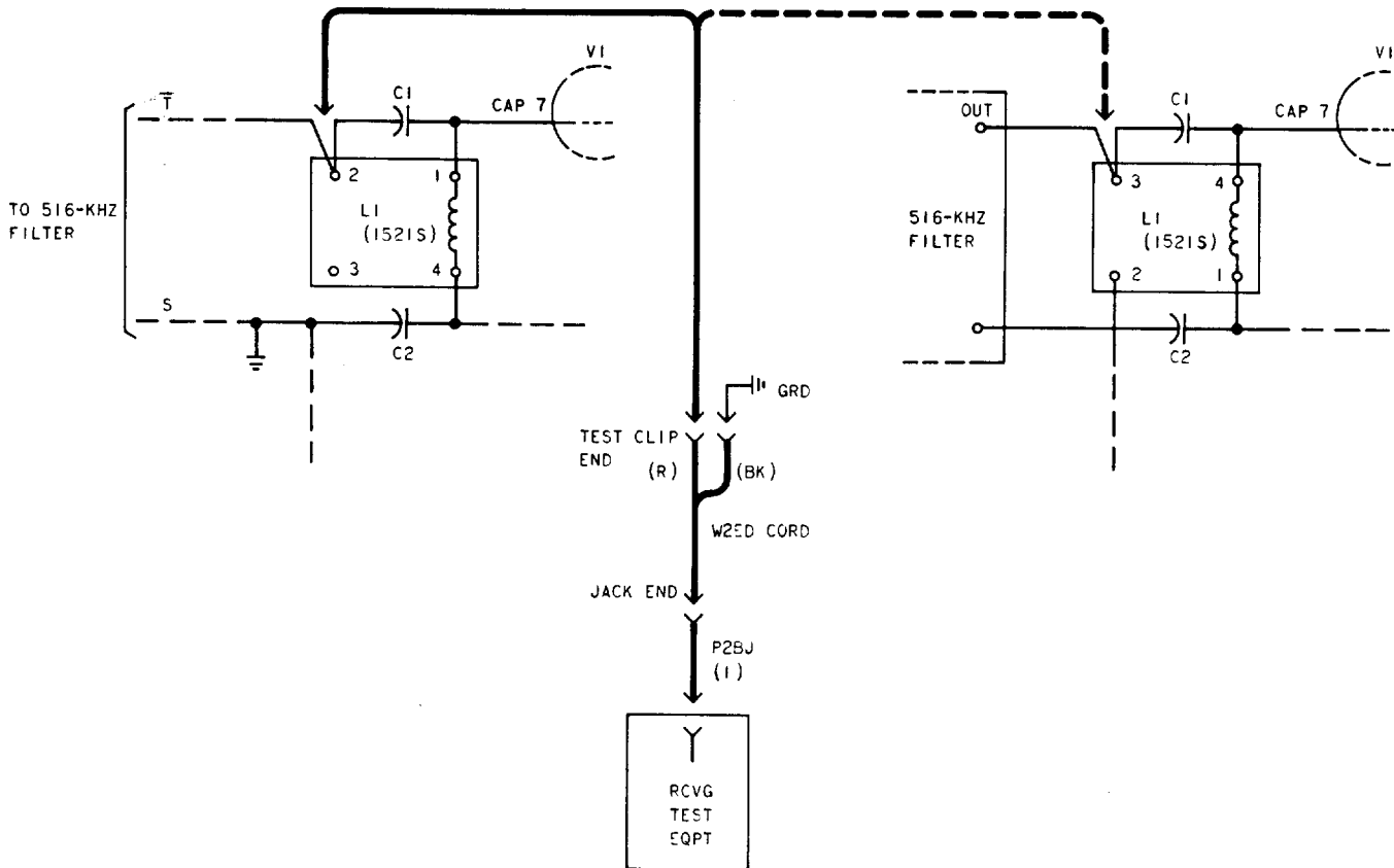
Fig. 3—Test Patch Using W2ED Cord
