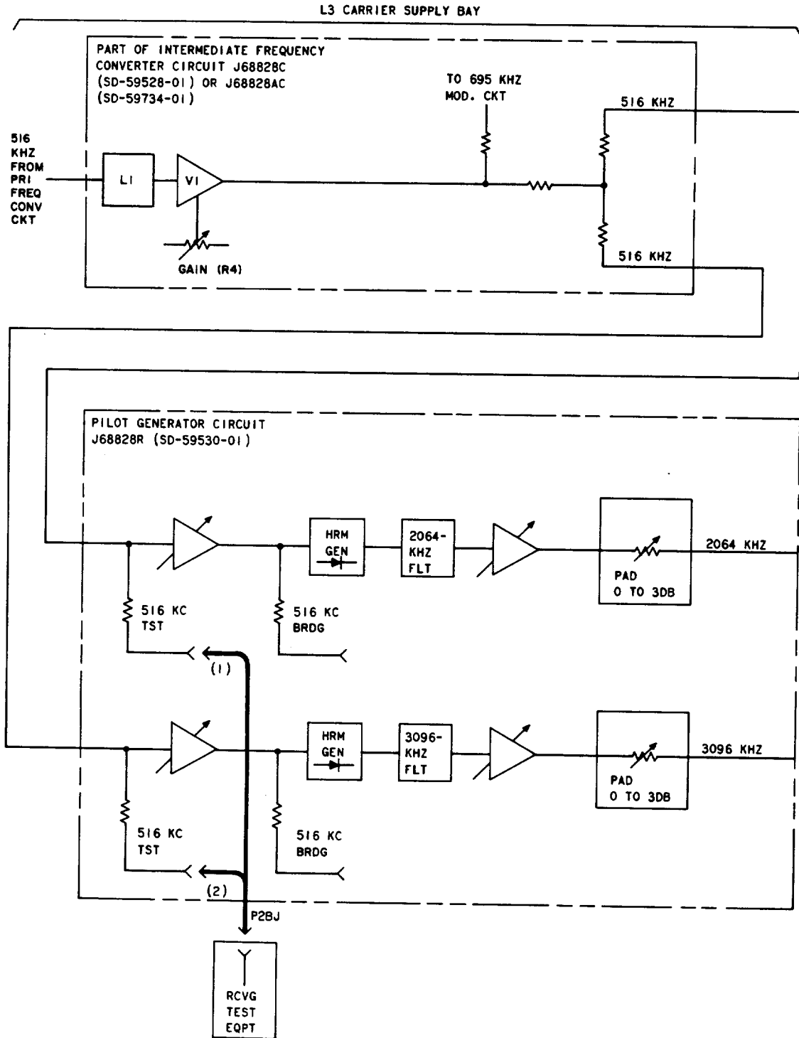
Fig. 2—Intermediate Frequency Converter Circuit—Measurement of the 516-kHz Output
