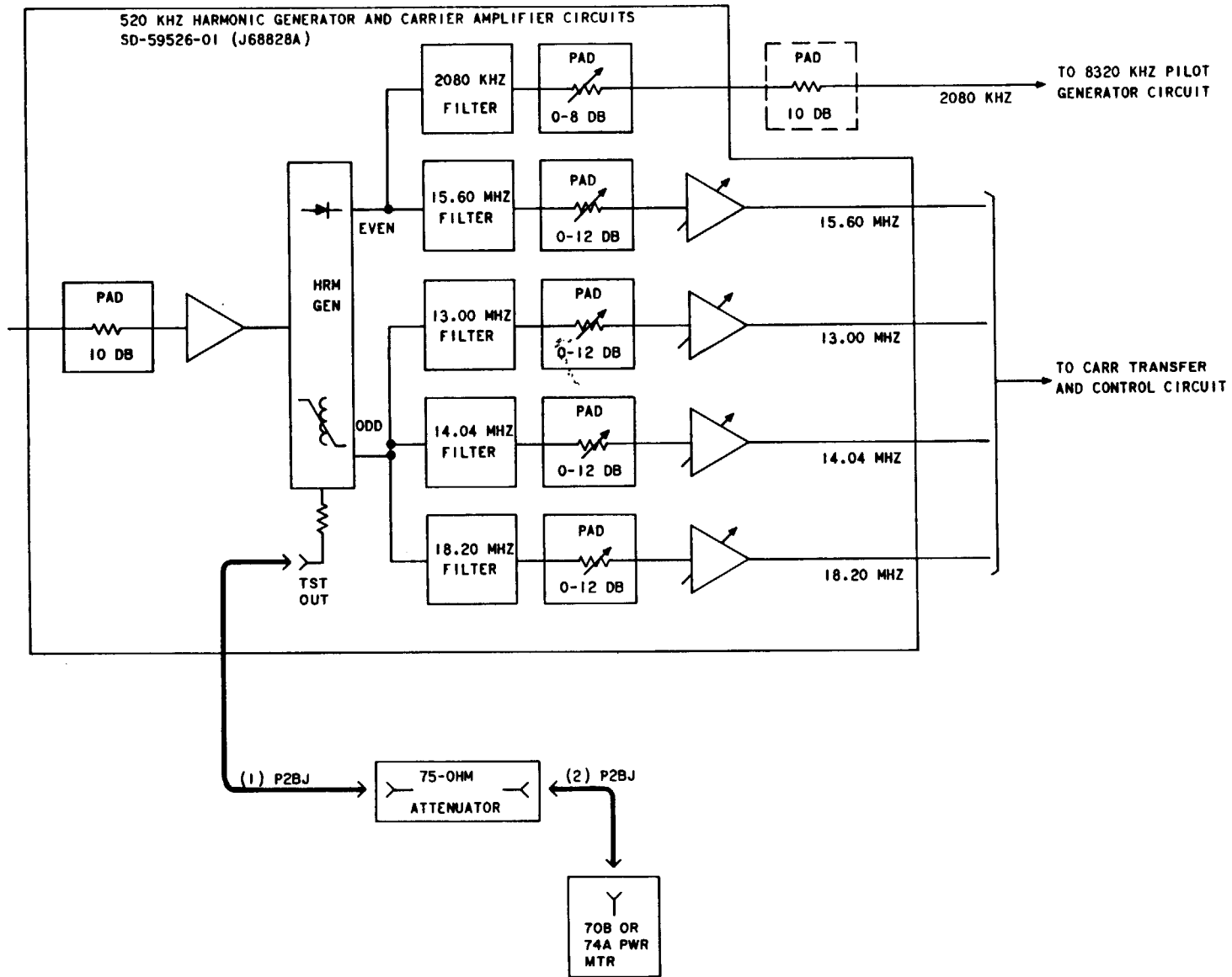
Fig. 2—Measurement of 520-kHz Harmonic Generator at TST OUT Jack
