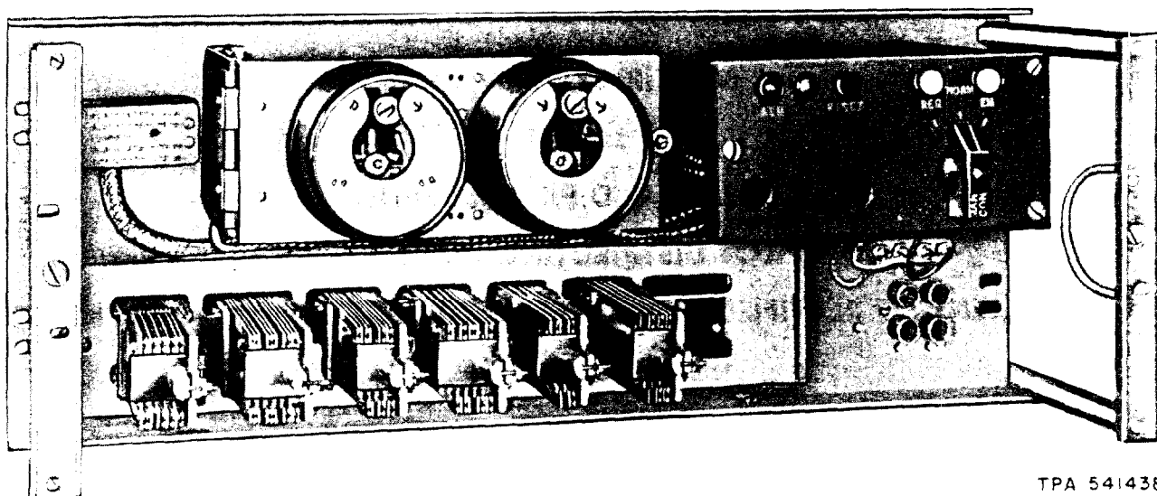
Fig. 1—Carrier and Pilot Transfer Control Panel J68828G
