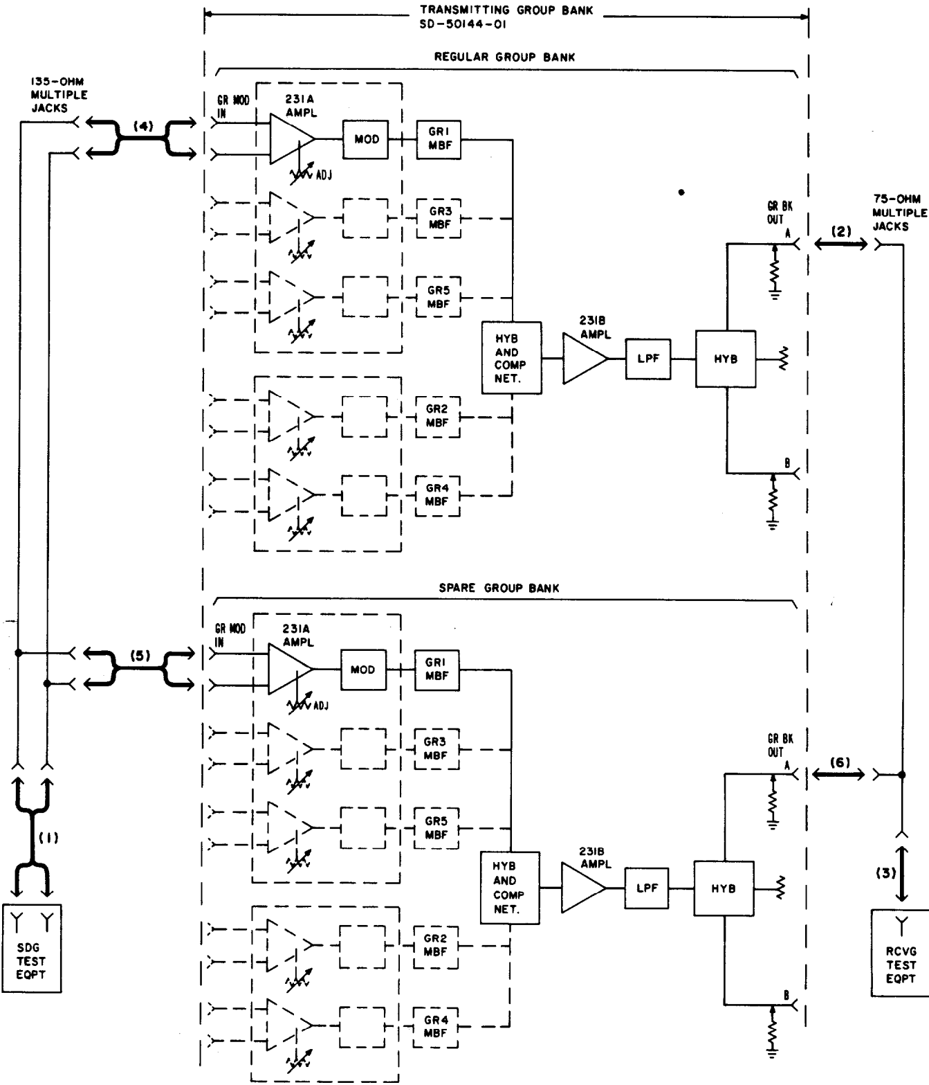
Fig. 2—Group Modulator—Group Turnover Test
