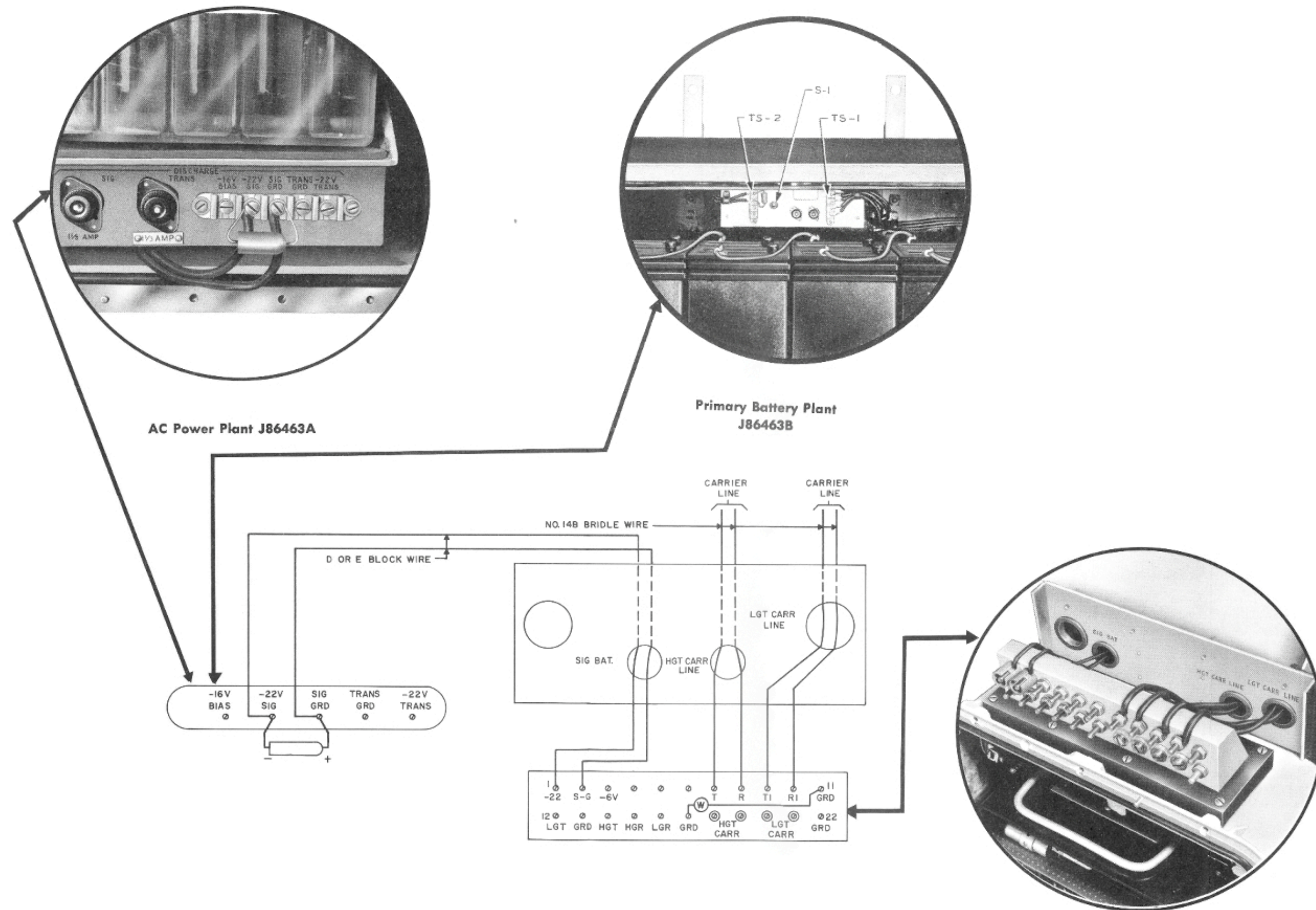
External Wiring and Line Connections
