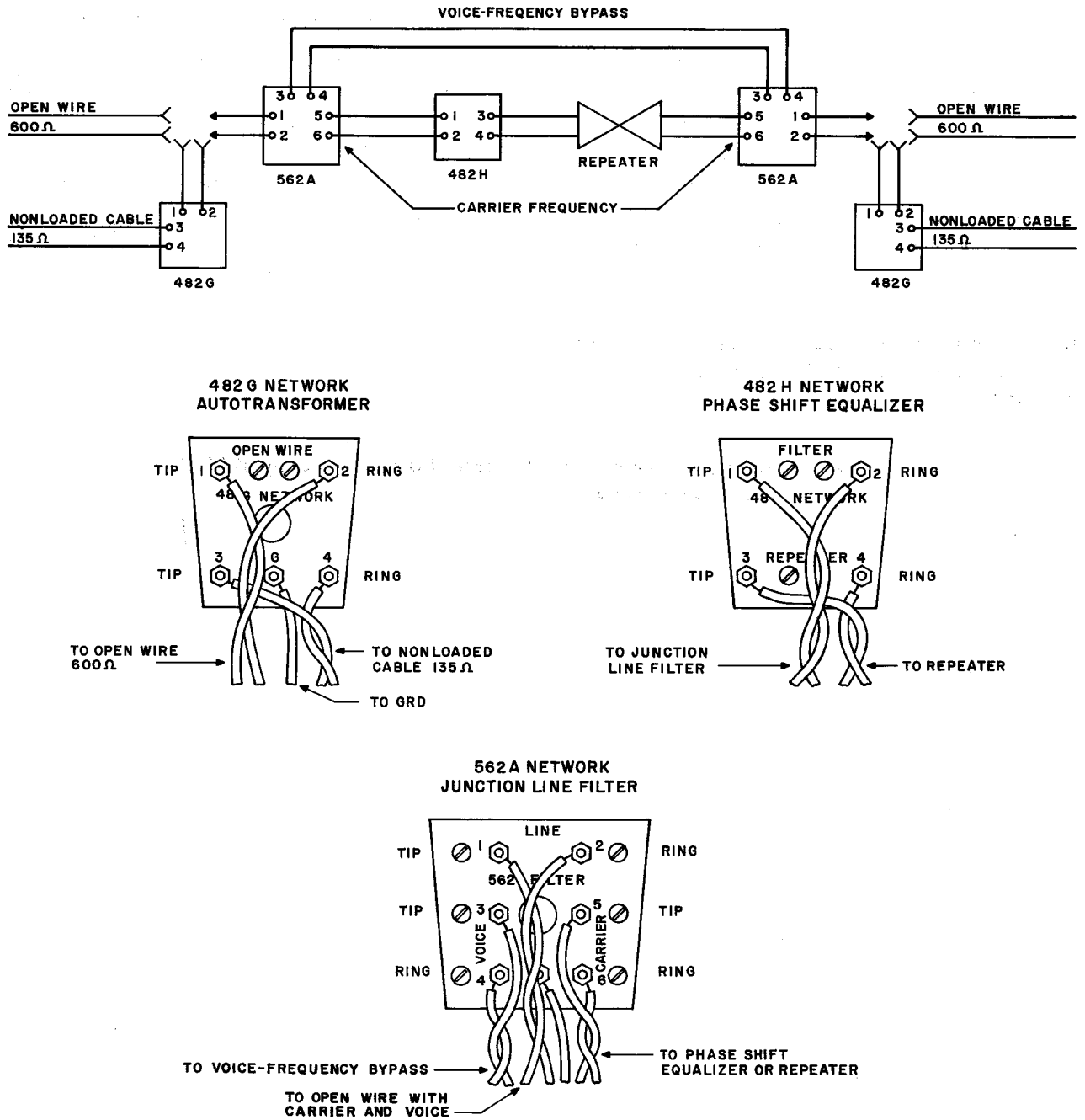
Fig. 1 – Network Application
