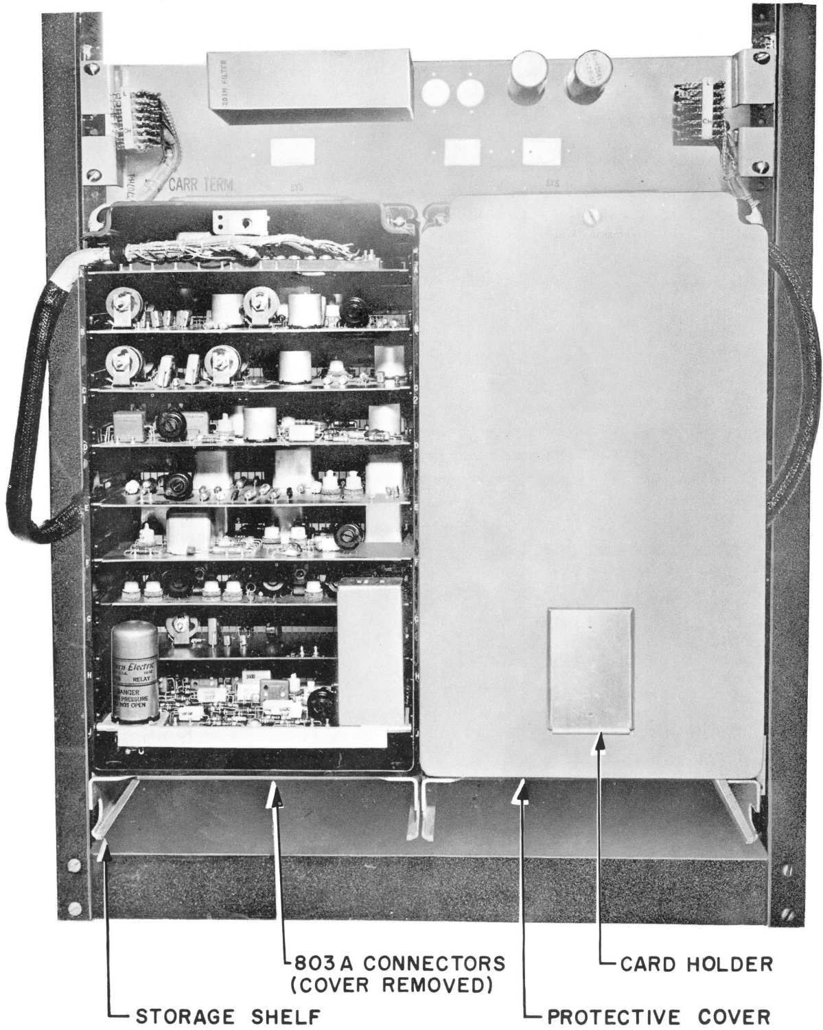
Fig. 1 - Central Office Terminal
