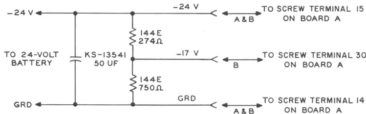
Fig. 5 — Battery Connections for Bench Adjustments
