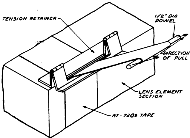
Fig. 2 - Tensioning Tape
