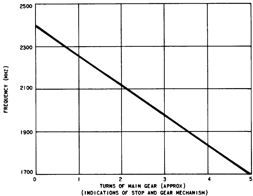
A - KLYSTRON TUNING MECHANISM ADJUSTMENT
