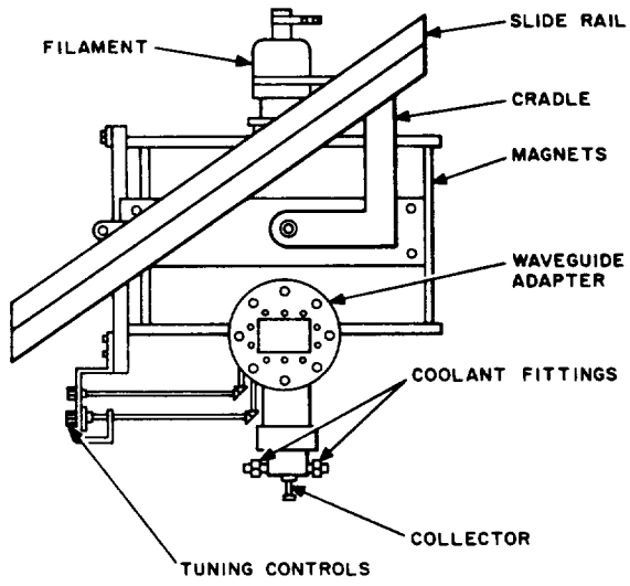
A-OPERATING POSITION
