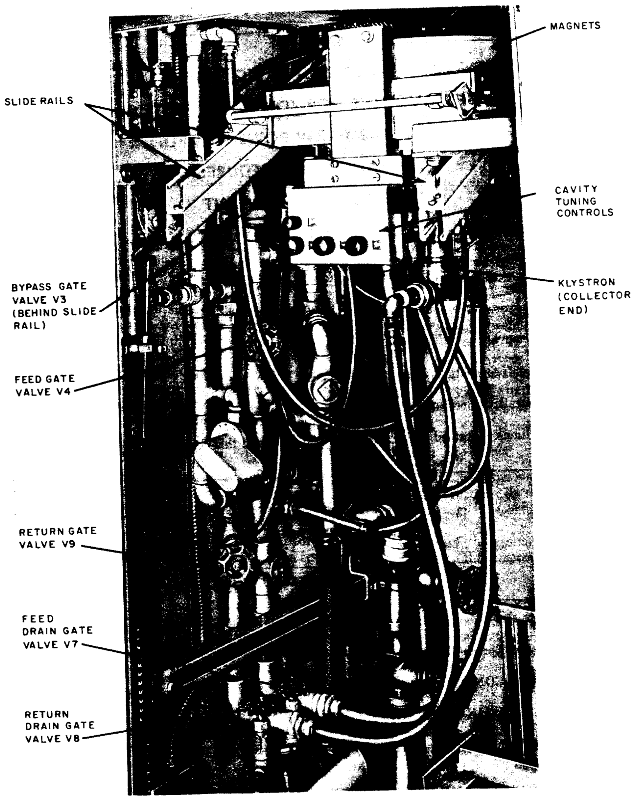
Fig. 1—Klystron Bay—Coolant Plumbing
