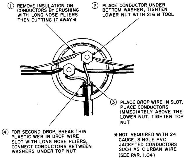
Fig. 12—Terminating Wire Leads
