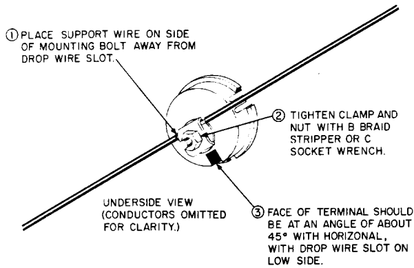
Fig. 11—Attaching Support Wire
