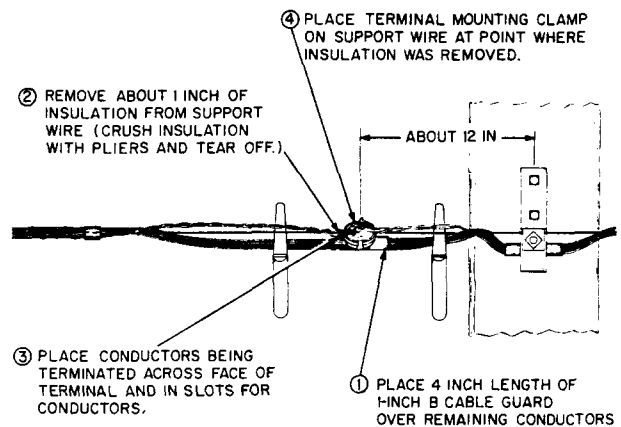
Fig. 10—Attaching 105A Wire Terminal
