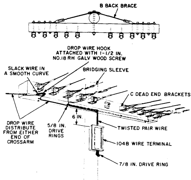
Fig. 4—For More Than Two Drops Use a 104B Wire Terminal Mounted on Pole
