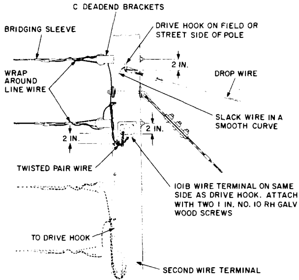
Fig. 6—Where Lines are Terminated on Deadend Brackets Attached to Face or Back of a Pole
