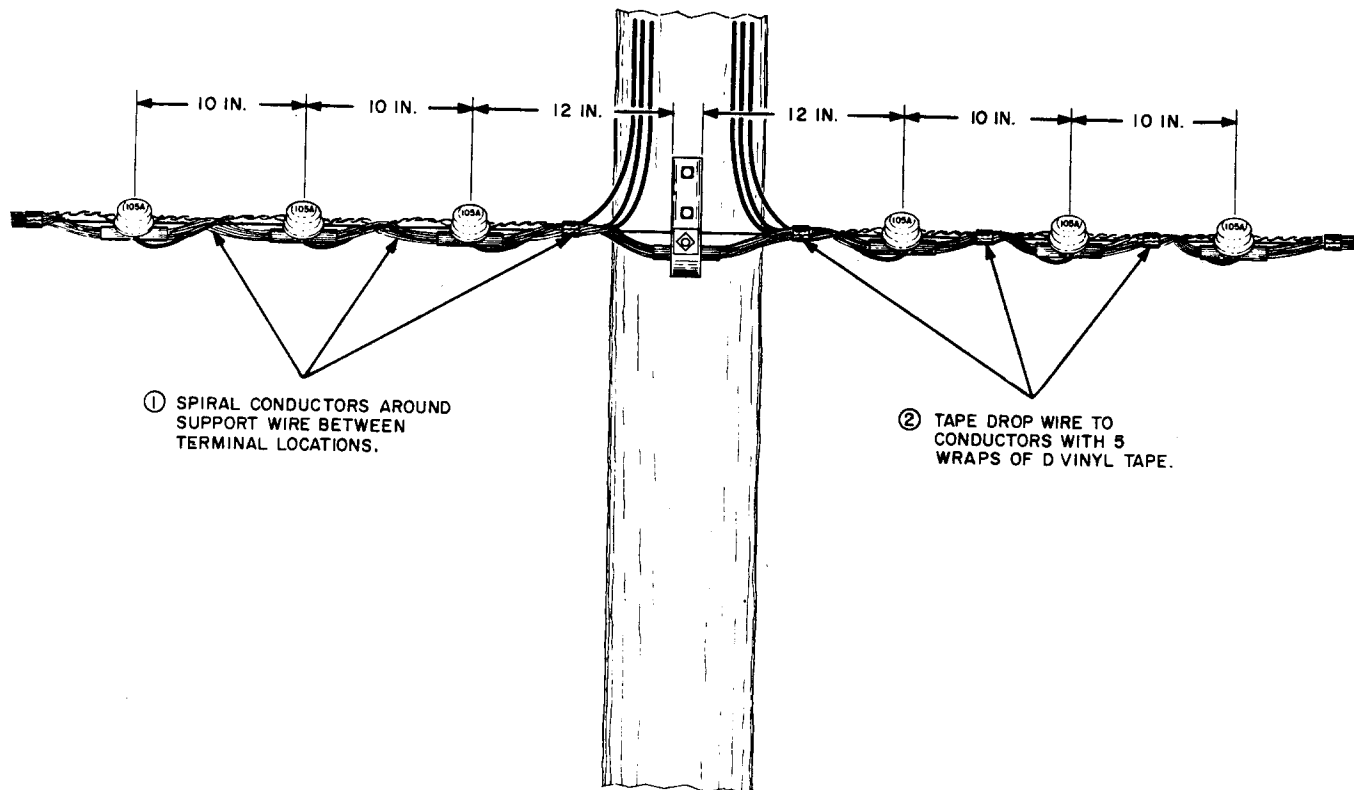
Fig. 14—Arrangement of Wire Terminals
