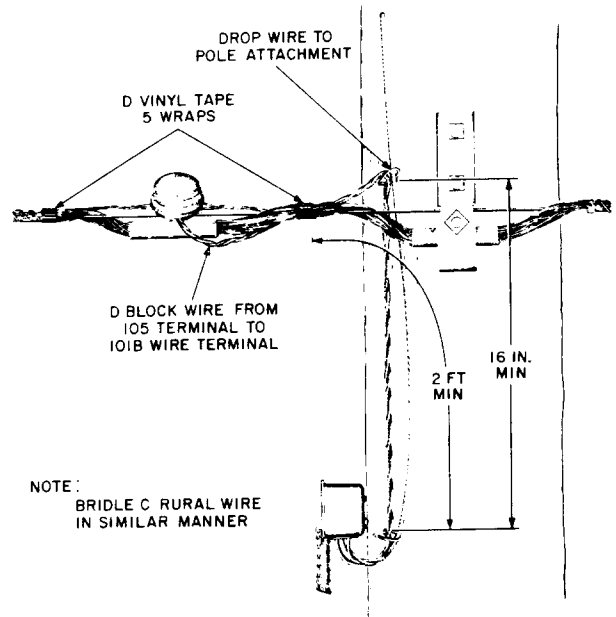
Fig. 13—Pole Attachment of Block and Rural Wire
