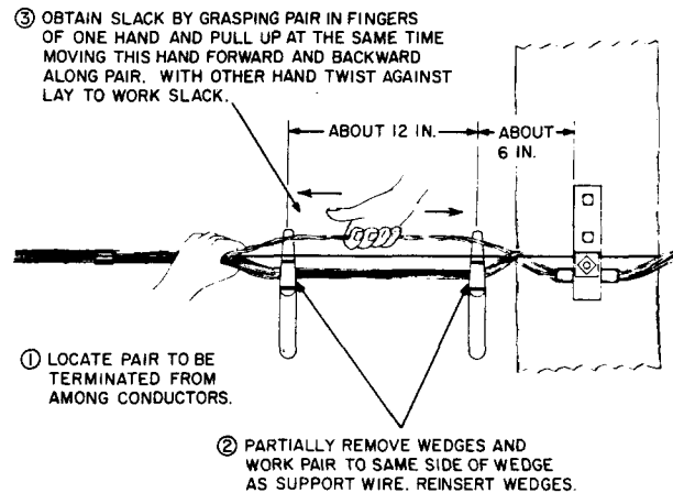
Fig. 9—Locating Wire Pair
