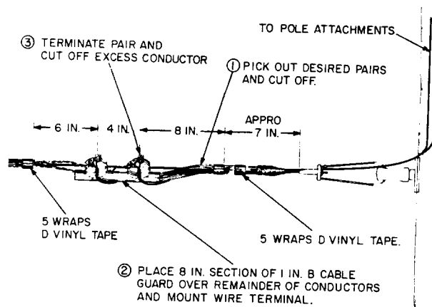
Fig. 15—Location of Wire Terminals at Dead-End Pole
