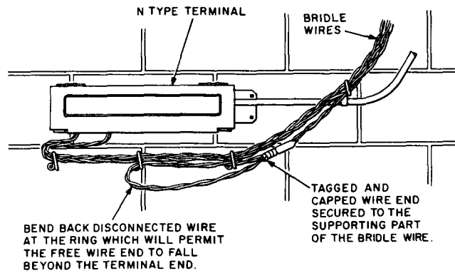
Fig. 6—N-Type Terminal Wall Mounted
