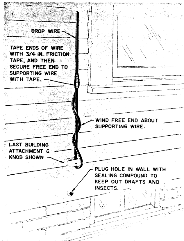
Fig. 1—Terminating Drop Wire When Protector is Removed
