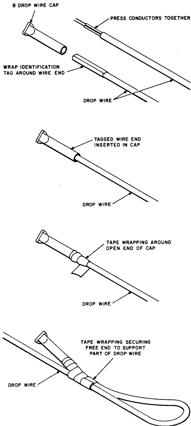
Fig. 3—Disposition of Disconnected Drop Wire
