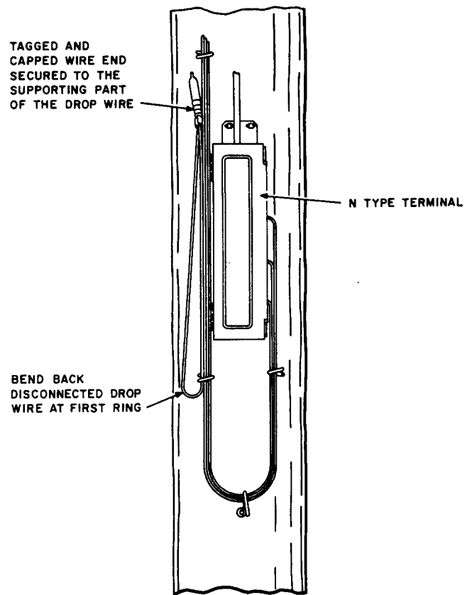
Fig. 4—N-Type Terminal, Pole Mounted
