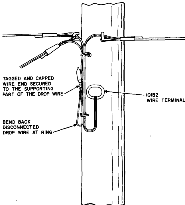
Fig. 7—101-Type Wire Terminal, Pole Mounted
