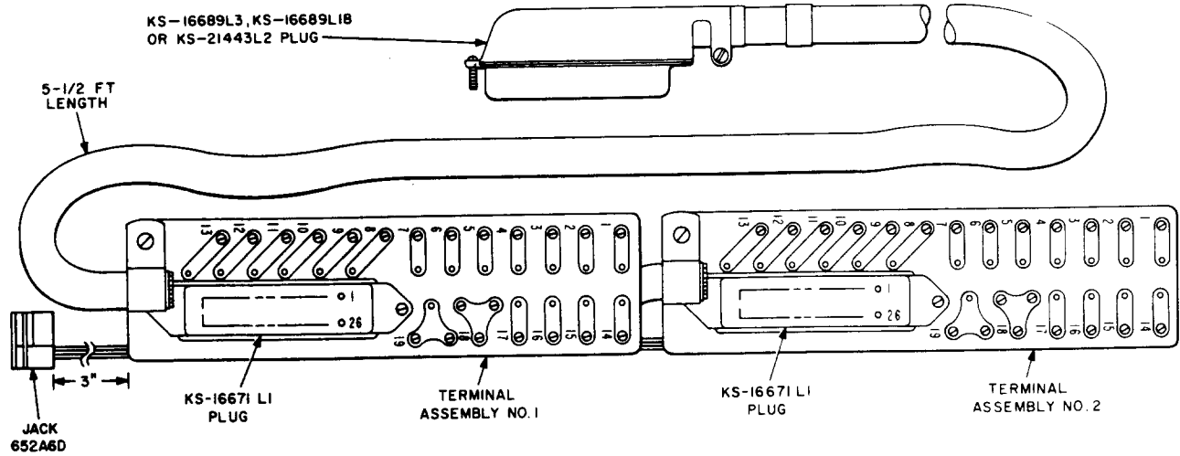
Fig. 4—B25G Connector Cable—View of Terminal Strip, Local Wiring Side
