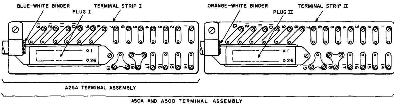
Fig. 2—View of Terminal Strip, Local Wiring Side
