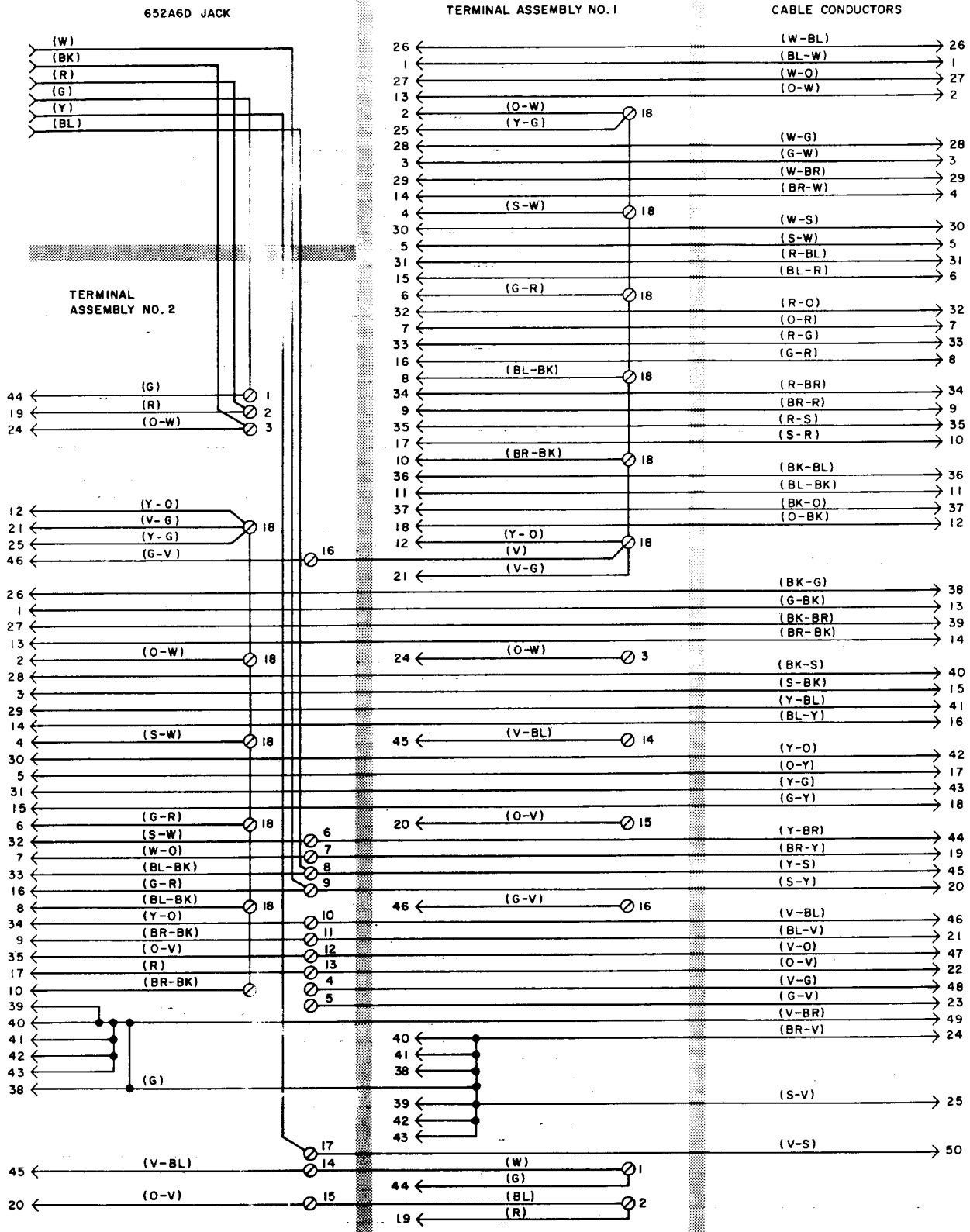
Fig. 11—B25G Connector Cable, Connections
