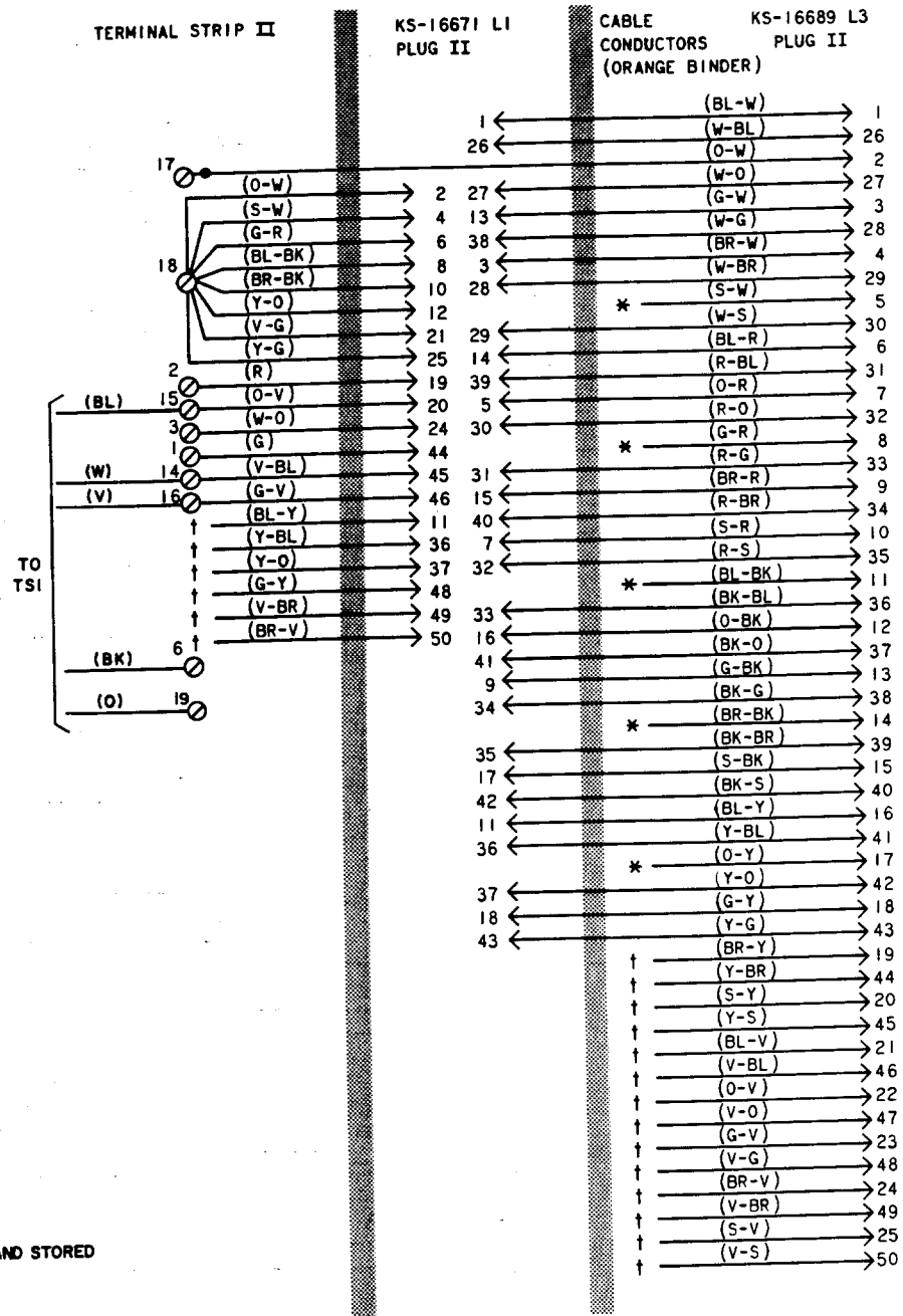
Fig. 12—B50B (O Binder) Connector Cable, Connections (Sheet 2 of 2)
