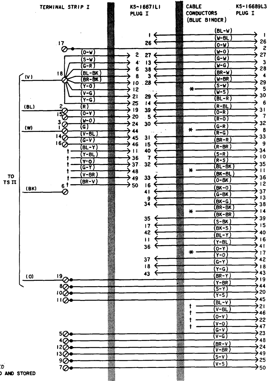
Fig. 12—B50B (BL Binder) Connector Cable, Connections (Sheet 1 of 2)
