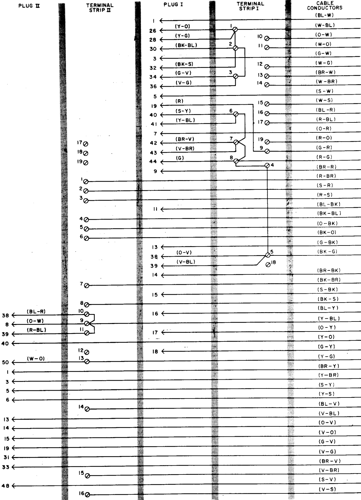
Fig. 8—A25E Connector Cable, Connections
