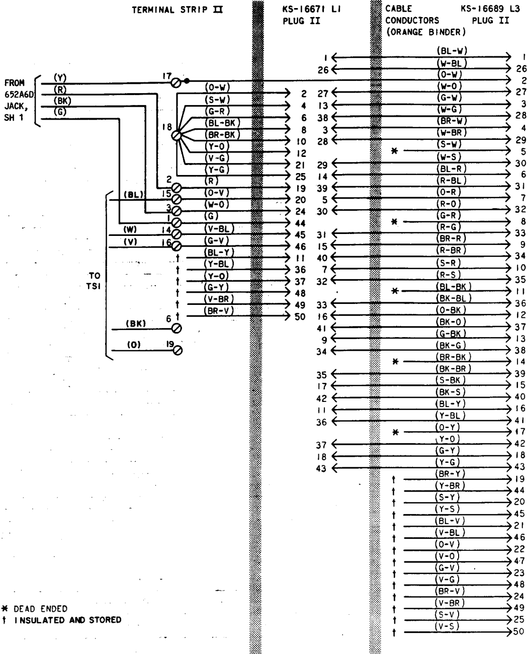
Fig. 13—B50C (O Binder) Connector Cable, Connections (Sheet 2 of 2)
