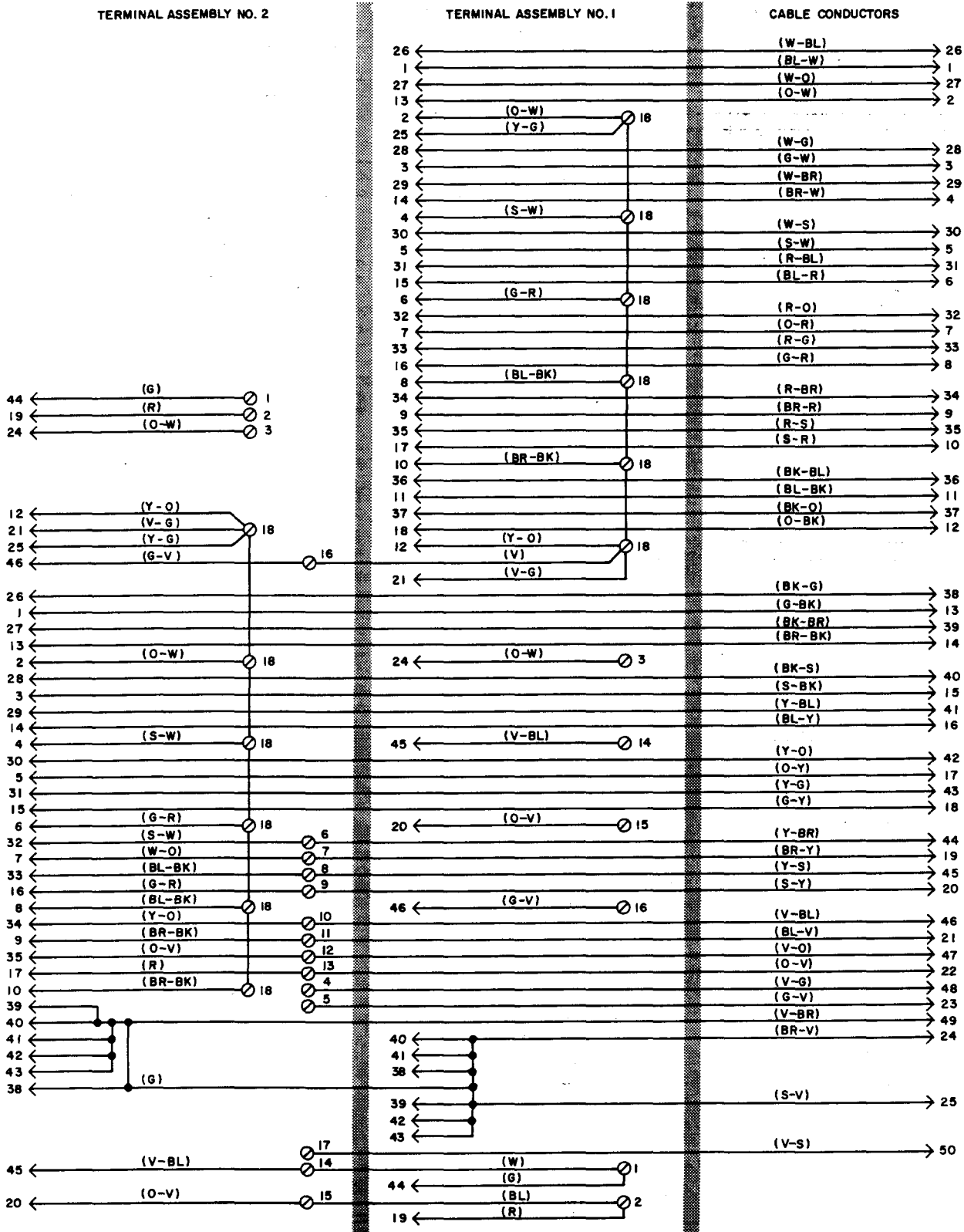
Fig. 10—B25C Connector Cable, Connections
