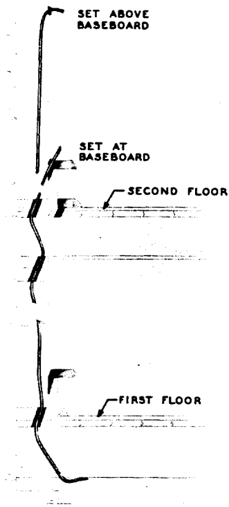
Fig. 3 – Fishing Outside Walls
