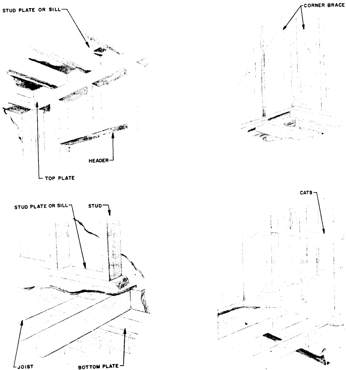
Fig. 5 – Wall Obstructions
