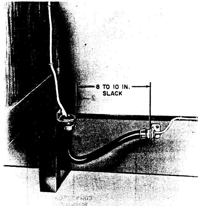
Fig. 1—Wiring to Desk-Station Tubing
