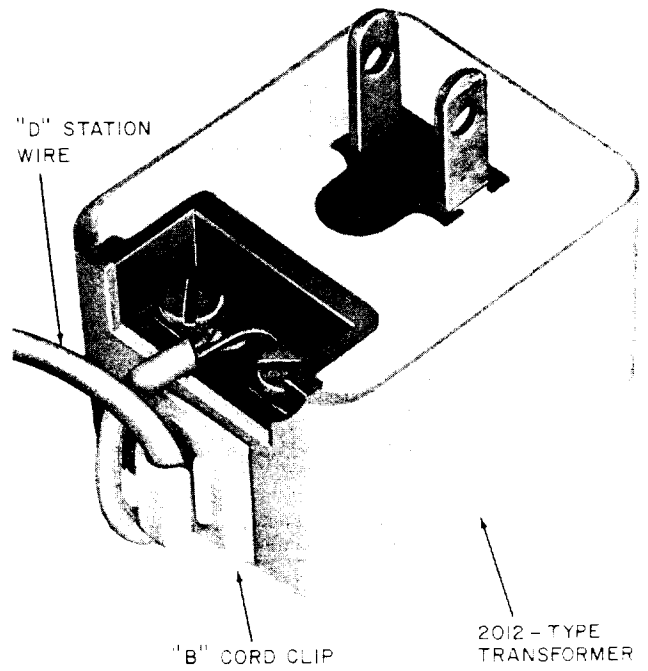
Fig. 13—Cord Clip Used to Secure Station Wire to 2012-Type Transformer
