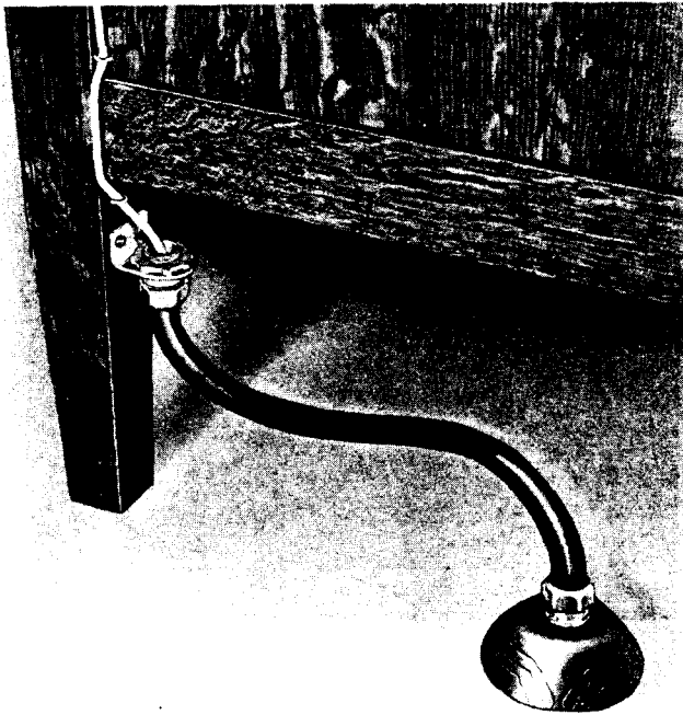
Fig. 4—Use of Station Tubing and 750-Type Service Fitting—No Underfloor Duct or Conduit System
