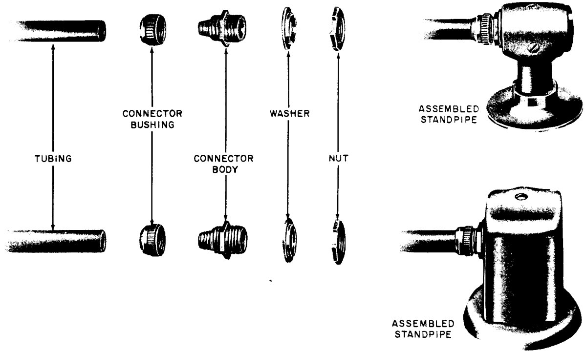
Fig. 3—Assembly of Station Tubing Fittings to Standpipes That Are Part of a Permanent Underfloor Duct or Conduit System
