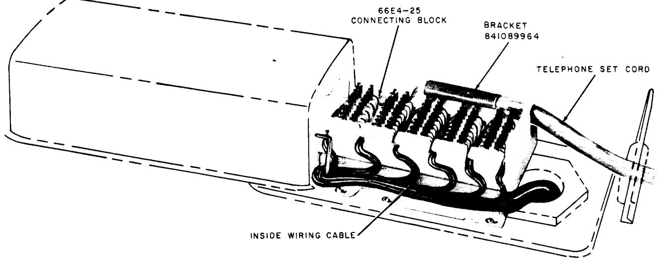
Fig. 5—66E4-25 Connecting Block Installed in Commercial Fitting
