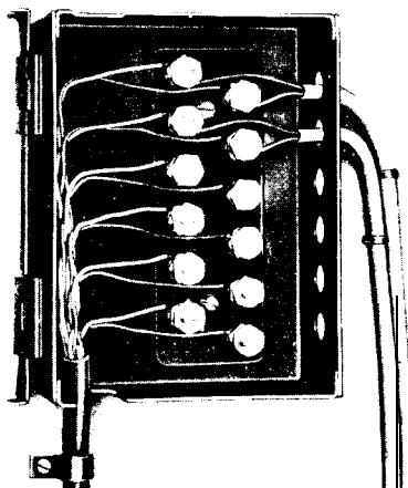
Fig. 3 - Station Wiring of HS-type Terminal
