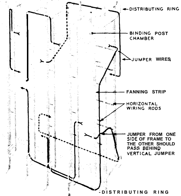
Fig. 9 — Cross-connection Arrangement on a Frame-type Terminal
