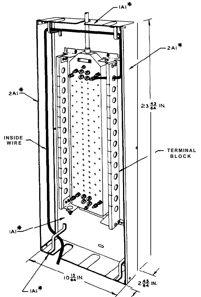
Fig. 14 -Station Wiring in Fuseless-type Protected Terminals
