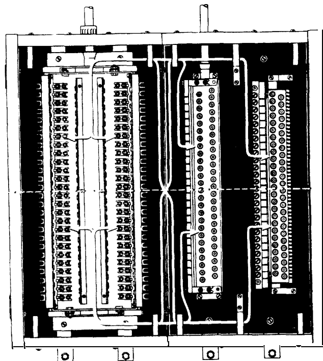
Fig. 10 — Typical Wiring Arrangement in LA-type Terminal
