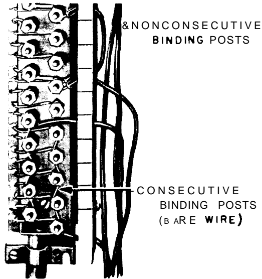
Fig. 8 — Use of Wire in Strapping Binding Posts
