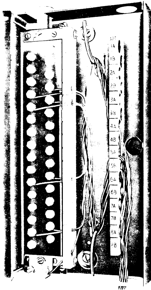
Fig. 2 -Station Wiring of GE-type Terminal
