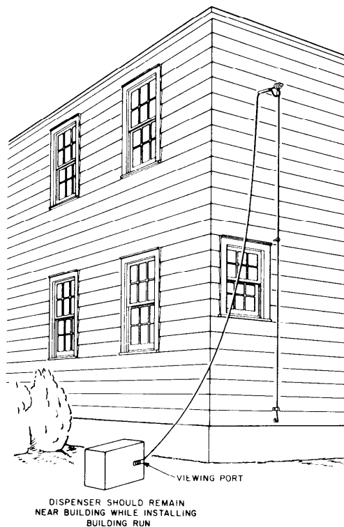
Fig. 3 - Drop Wire Attached to Building
