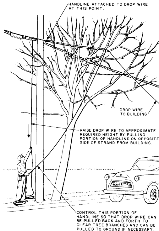
Fig. 11 - Raising Drop Wire
