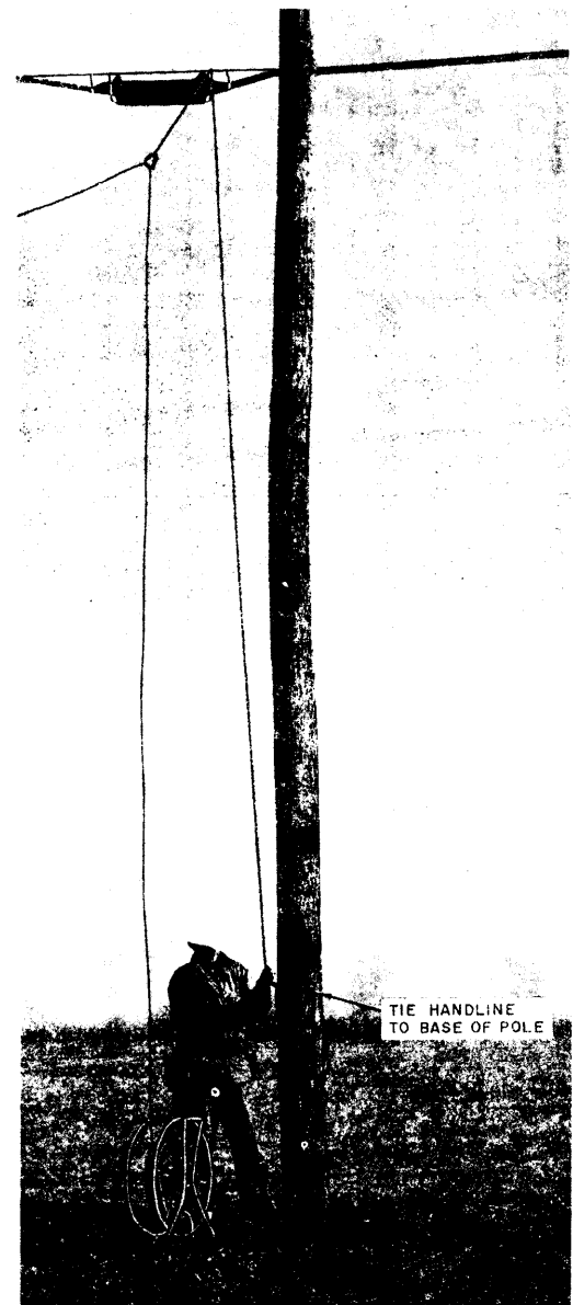
Fig. 16 - Drop Wire Raised to Approximate Height - Reel Method
