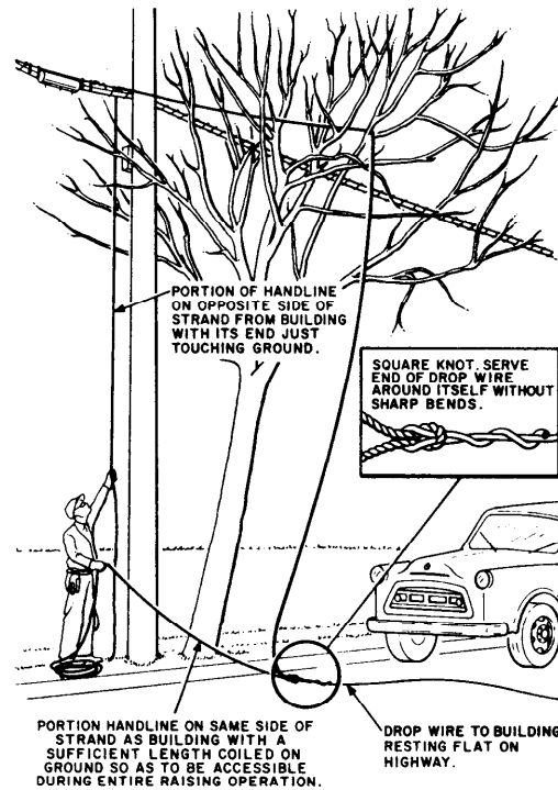
Fig. 10 - Drop Wire Tied to Handline
