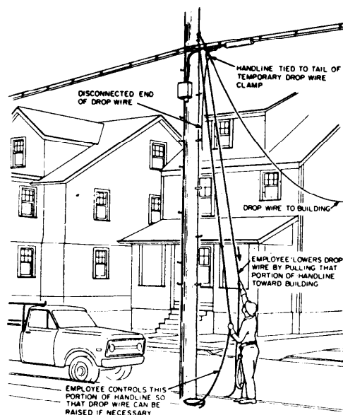
Fig. 12 - Lowering Drop Wire
