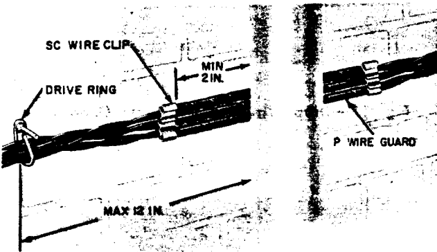
Fig. 7—Block Wires Crossing Behind Pipe
