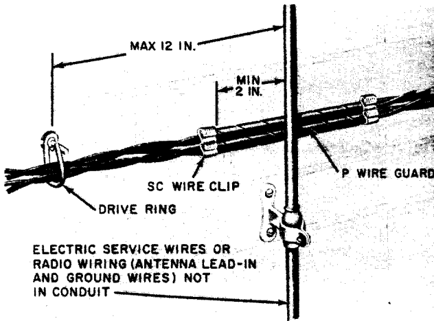
Fig. 12—Block Wire Crossing Behind Foreign Wire
