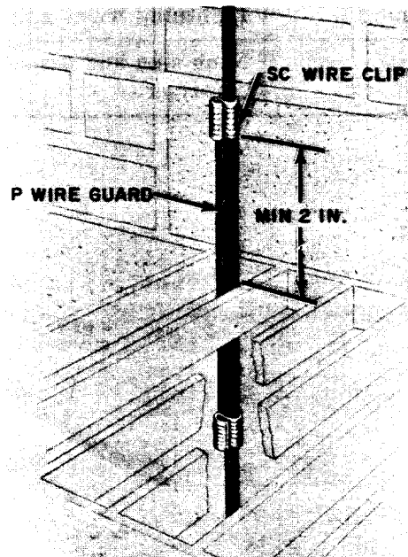
Fig. 5—Protecting Wire Run Through Stationary Metal Grating
