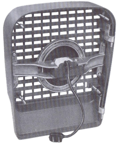
Fig. 18—KS-16301, List 6 Horn
