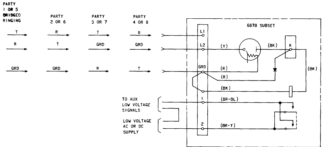
Fig. 26—Noncontinuous Low Voltage Auxiliary Signal
