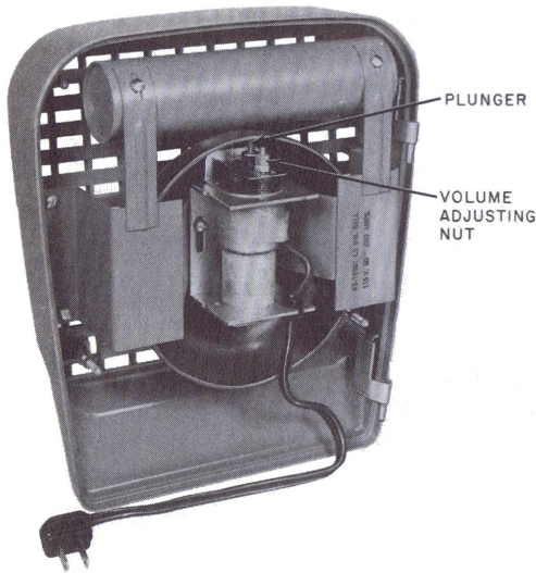
Fig. 9—KS-16301, List 3 Bell
