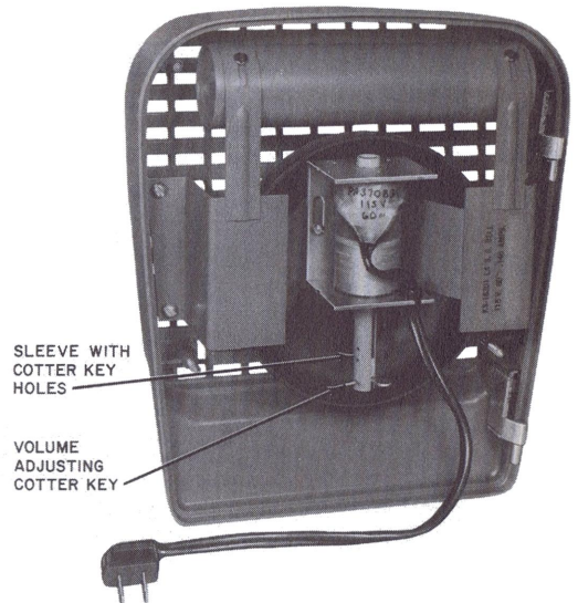
Fig. 10—KS-16301, List 4 Bell
