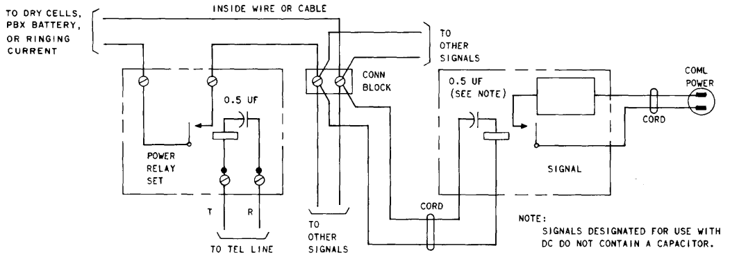
Fig. 22—Multiple Signal
