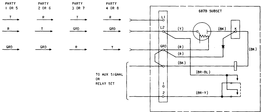
Fig. 25—Auxiliary Signals on Party Line
