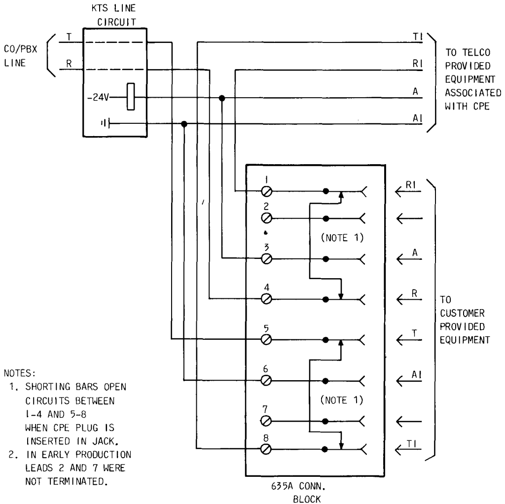
Fig. 4—Connections for USOC RJ34X
