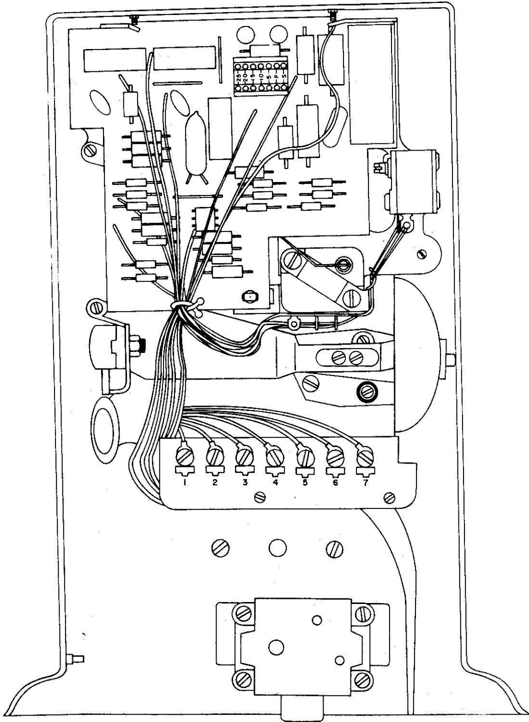
Figure 1 Multislot Coin Telephone Set Totalizer.
