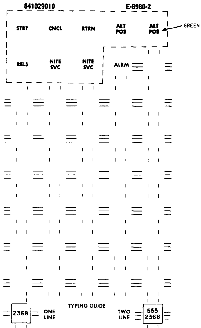
Fig. 16—841029010 (E-6980-2) Designation Tabs
