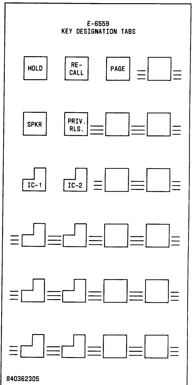
Fig. 11—840362305 (E-6559) Designation Tabs
