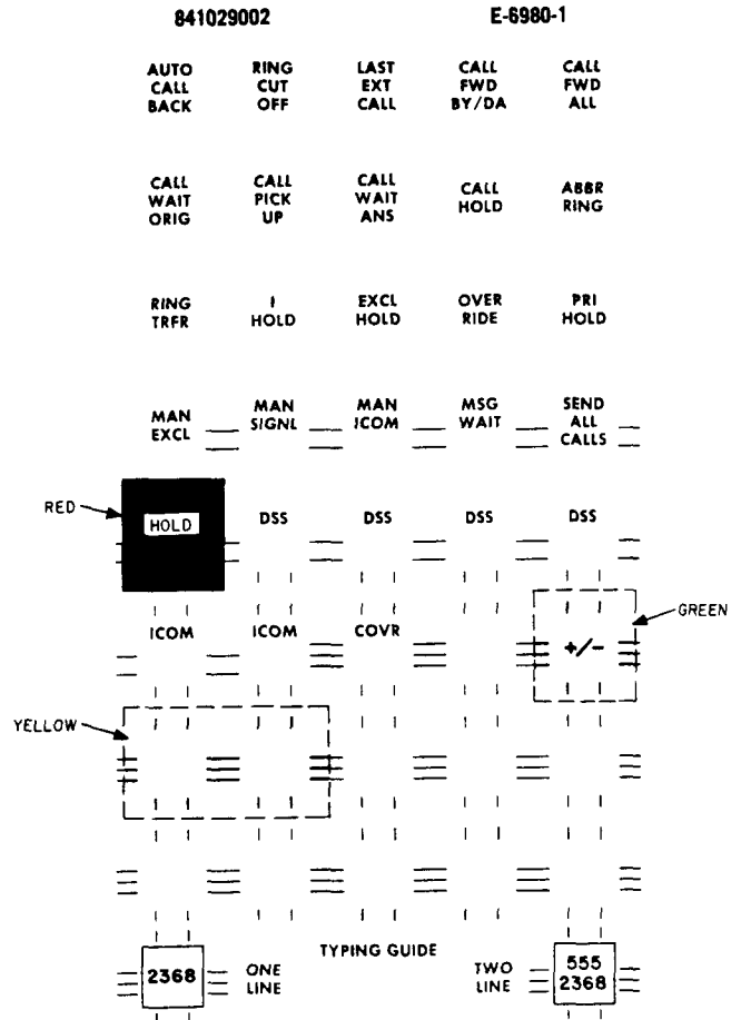
Fig. 15—841029002 (E-6980-1) Designation Tabs
