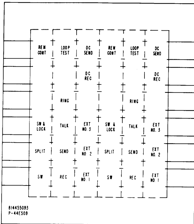
Fig. 10—814455093 (P-44E509) Designation Strip
