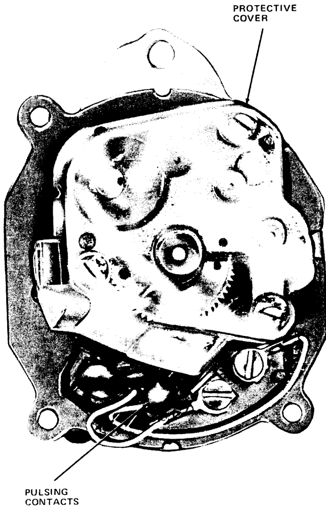
Fig. 2—10AL Dial, Rear View
