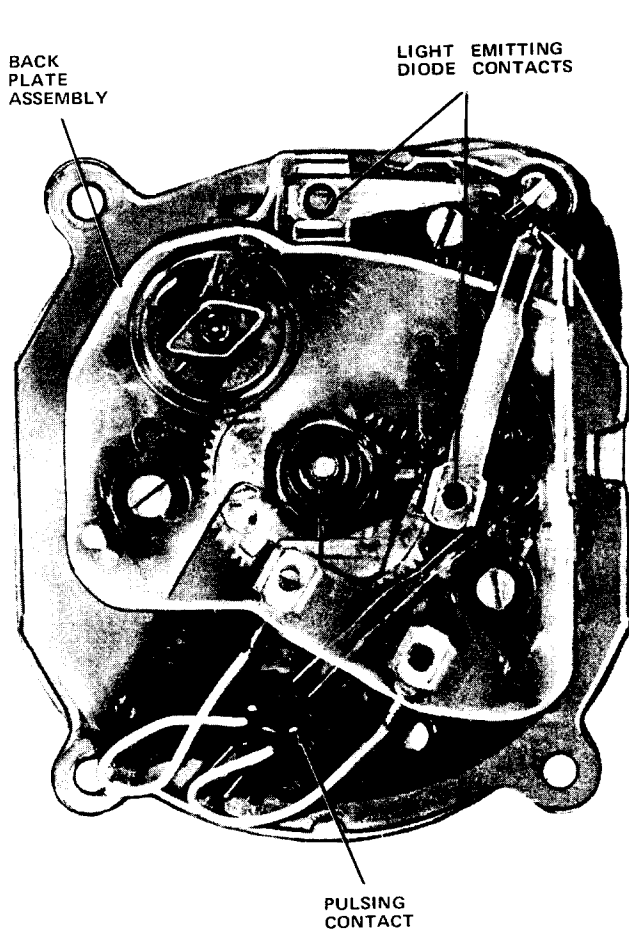
Fig. 4—10D Dial, Rear View
