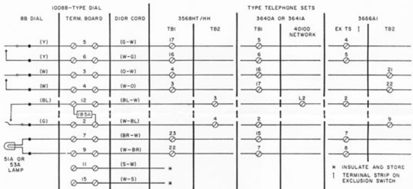
Fig. 3 — 1008B Dial, Connections
