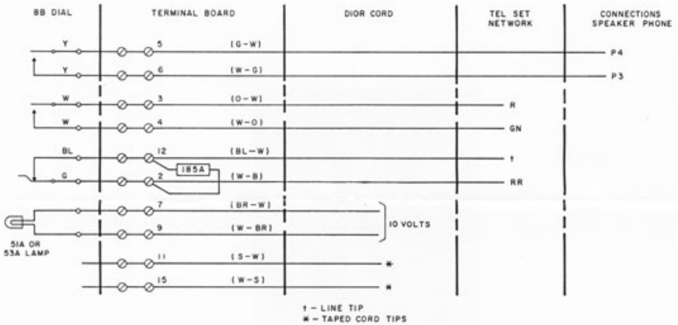
Fig. 2 — 1008B Dial Schematic and Connecting Diagram
