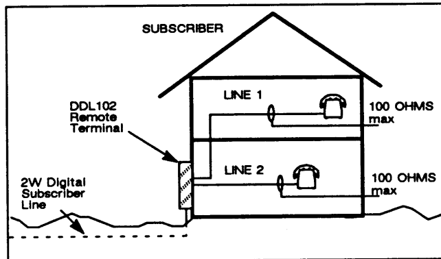
Figure 1. Typical DDL102 DuaLine Plus RT Installation
