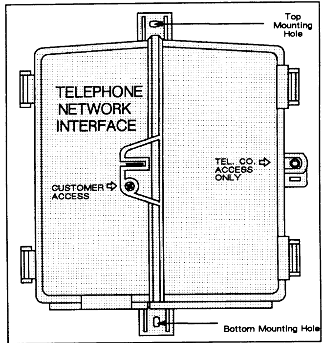
Figure 2. DDL102 DuaLine Plus Remote Terminal in the Secured Position (Closed)
