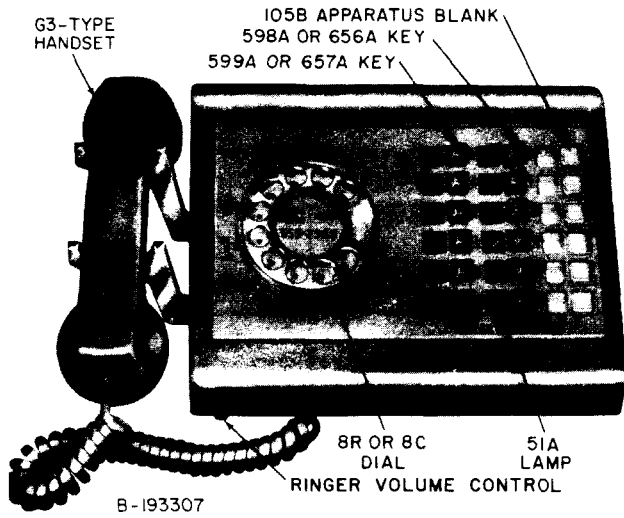
Fig. 2—Typical Telephone Set Using 590- or 650-Series Keys
