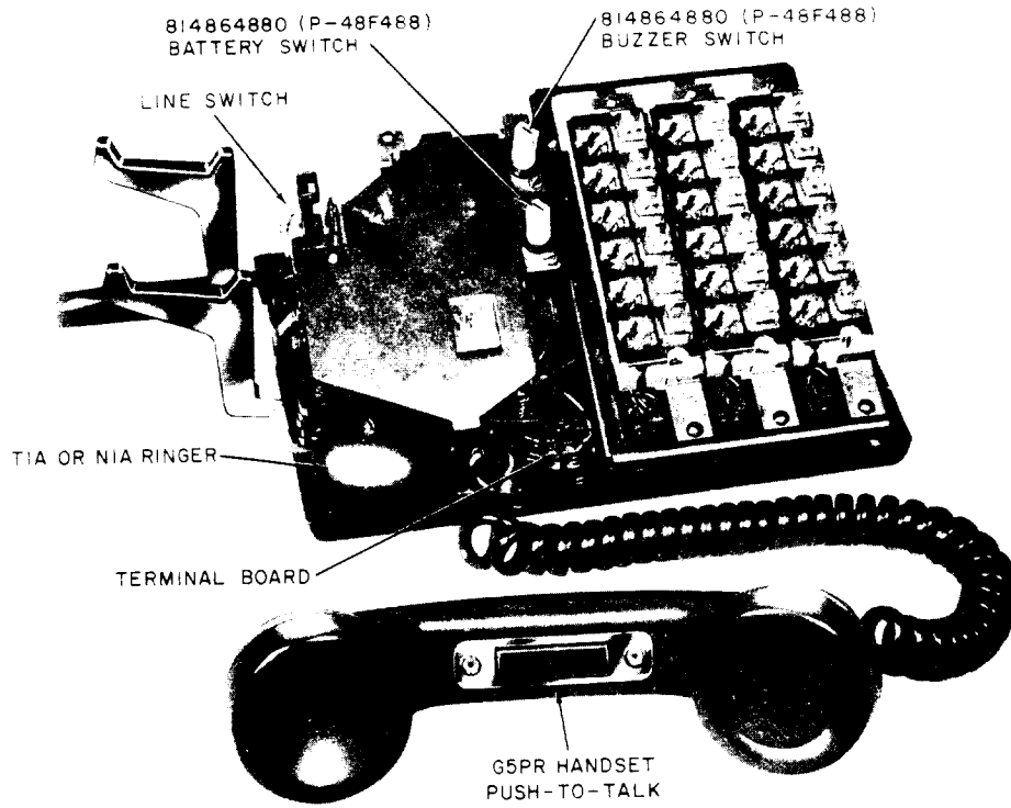
Fig. 9—625A1 (MD) Telephone Set, Interior View
