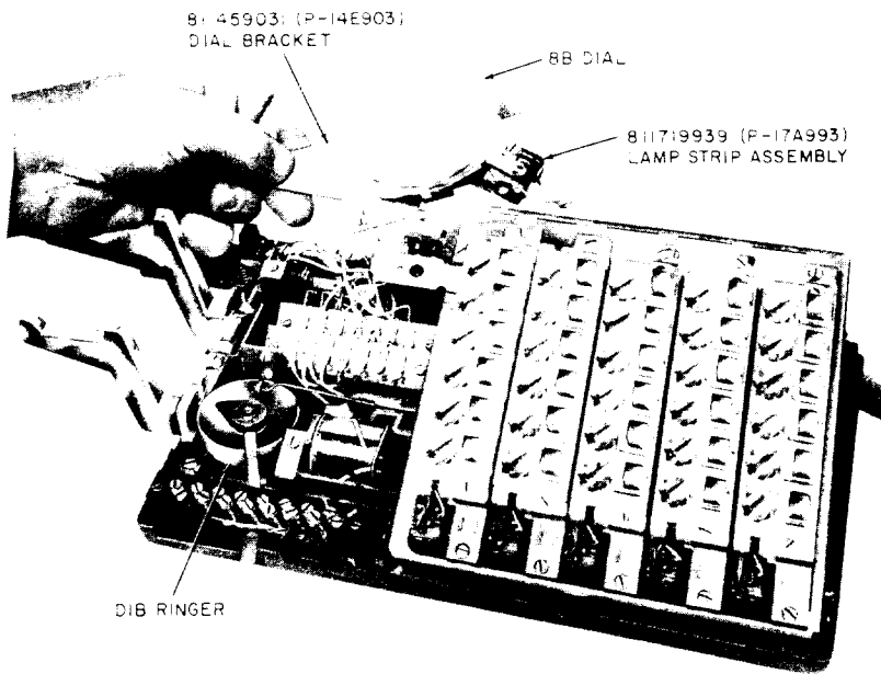
Fig. 4—617A15 (MD) Telephone Set, Interior View
