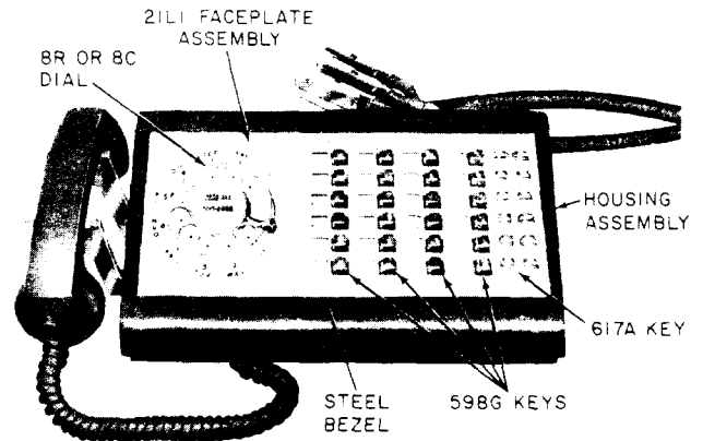
Fig. 1—609-Type (MD) Telephone Set
