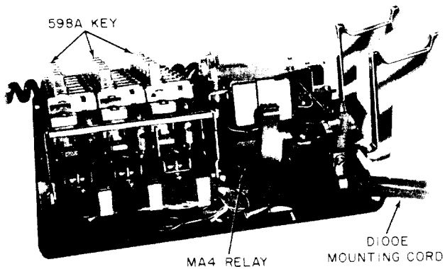
Fig. 10—625A1 (MD) Telephone Set, Rear View
