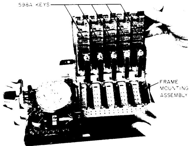
Fig. 7—598A Keys and Frame Mounting Assembly of 617-type (MD) Telephone Set
