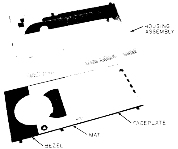
Fig. 11—Housing, Faceplate, Bezel, and Mat of 617-Type (MD) Telephone Set
