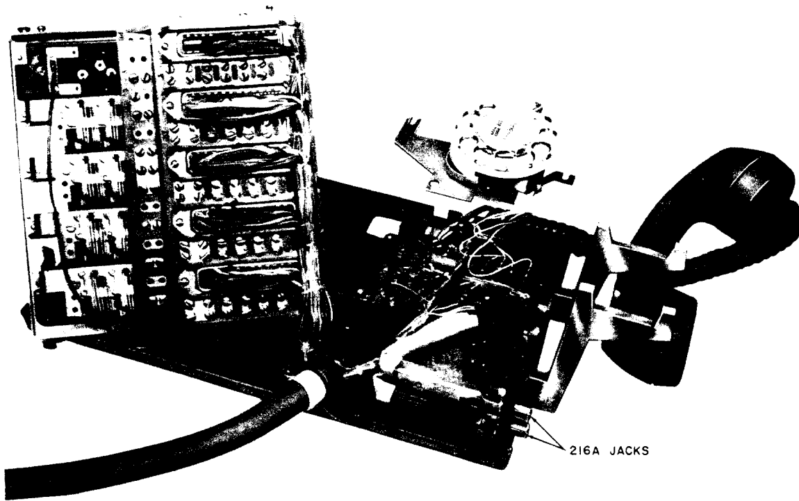
Fig. 2—609A1 (MD) Telephone Set Housing Removed, Key Frame and Dial Lifted
