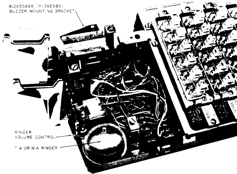
Fig. 6—617B15 (MD) Telephone Set, Interior View
