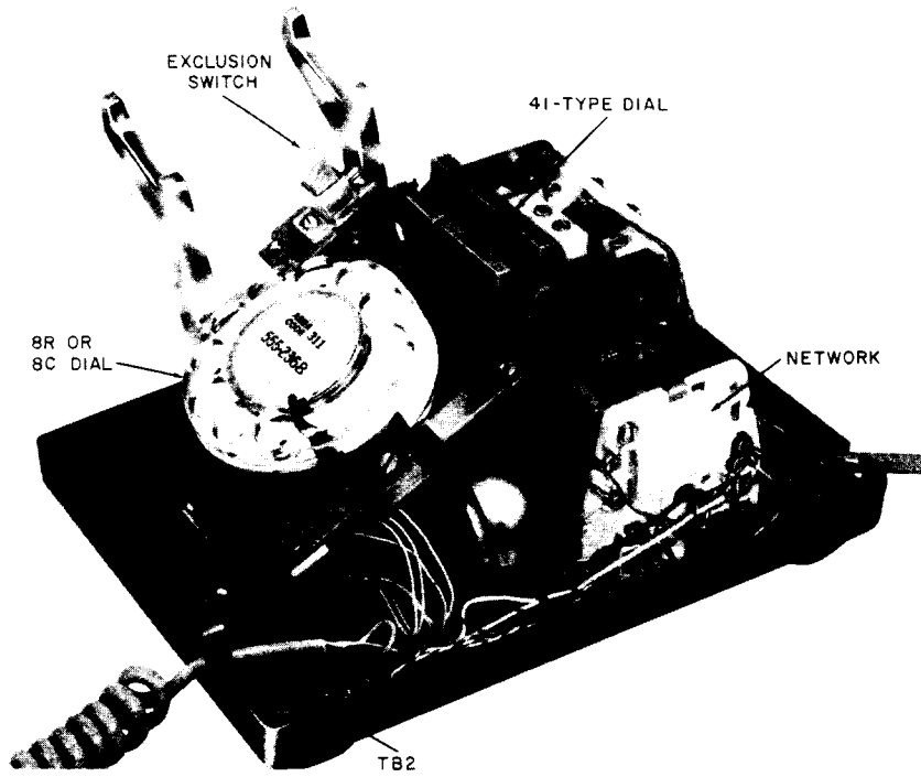
Fig. 3—660-Type Telephone Set, Housing Removed
