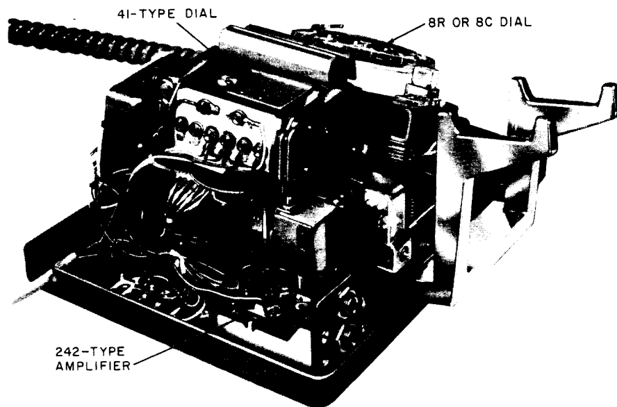
Fig. 4—663-Type Telephone Set, Housing Removed
