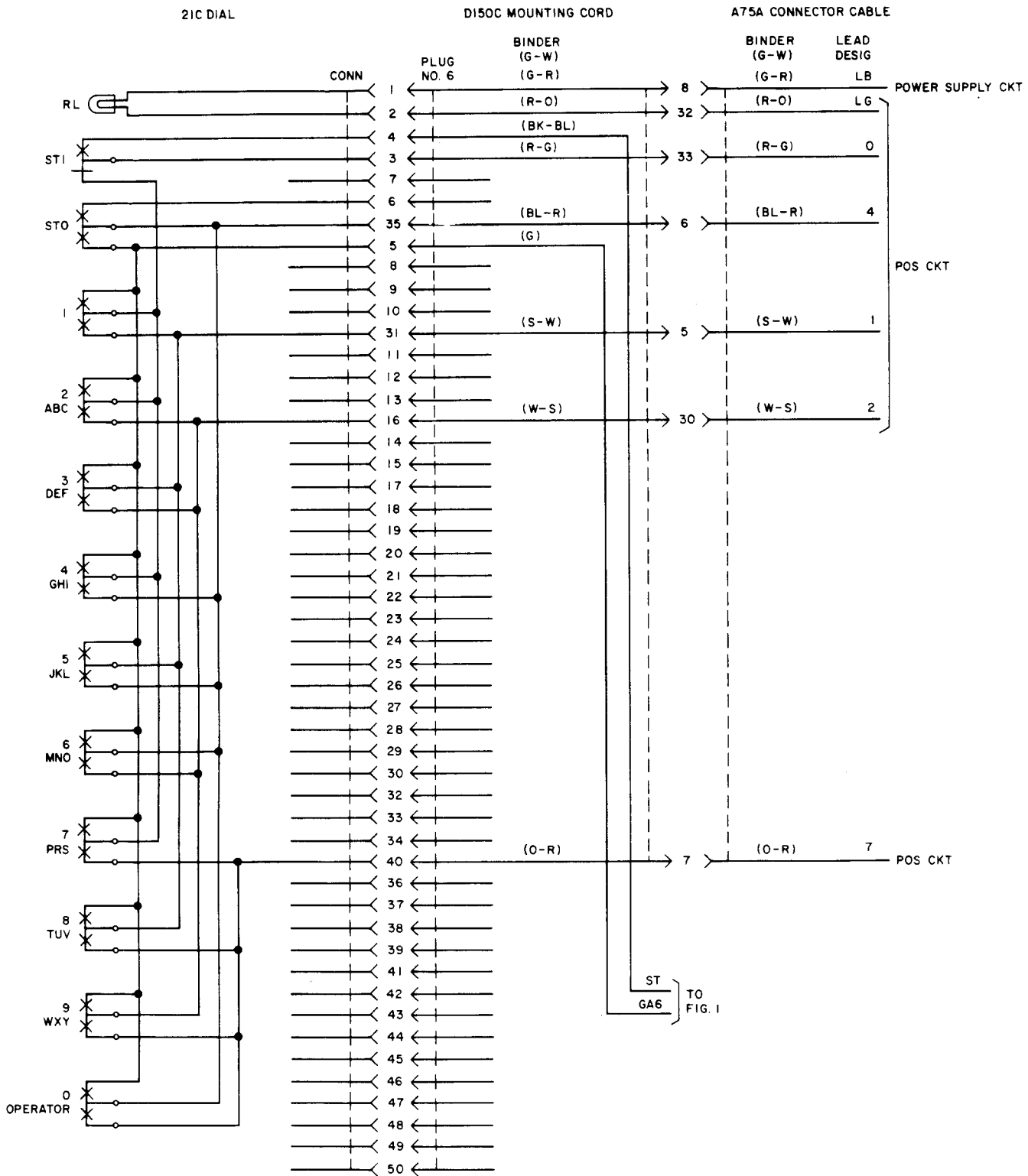
Fig. 3—Pushbutton Dial
