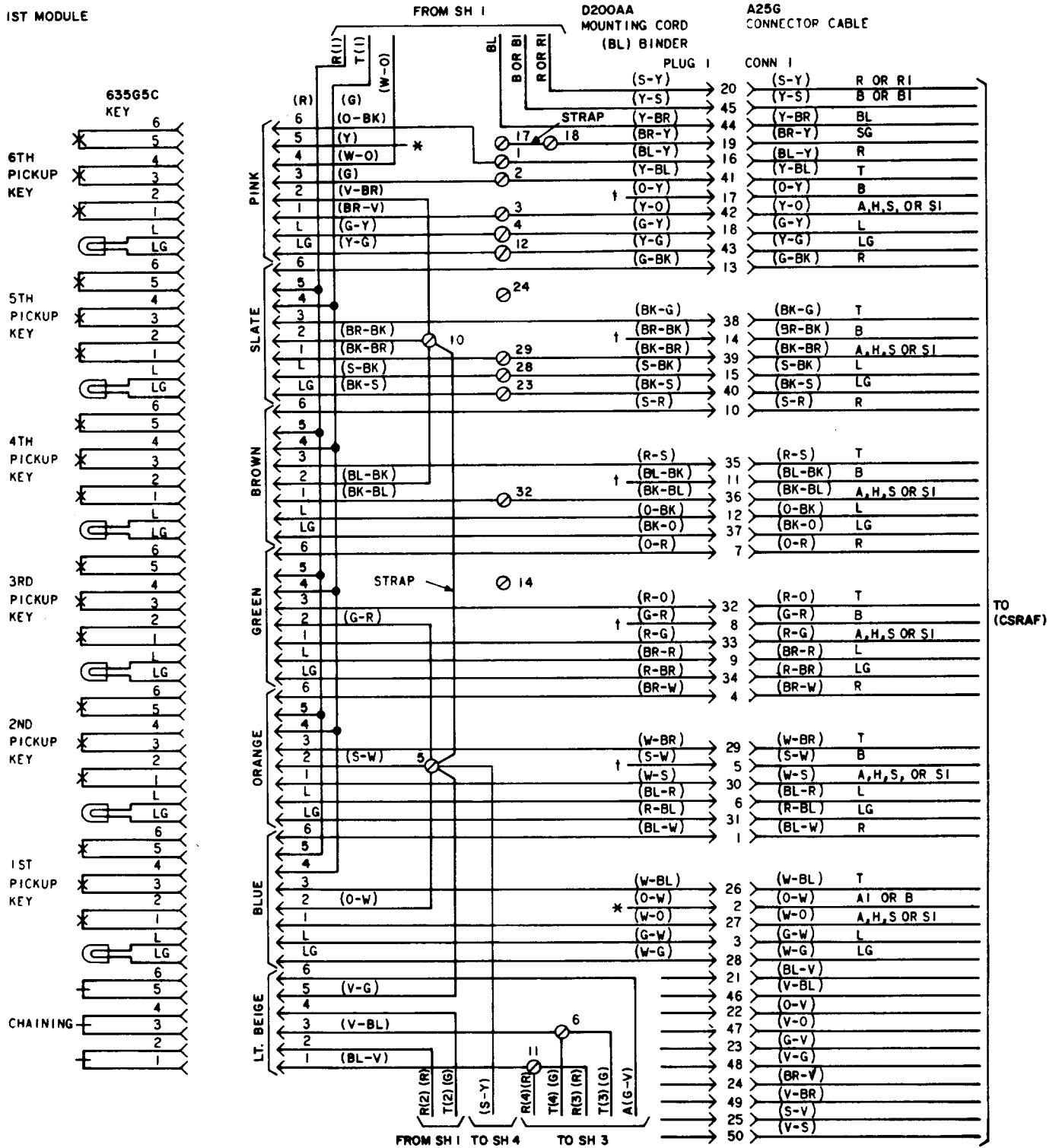
Fig. 1—637EA13 (MD) and 637EAM13 Telephone Set, Connections (Sheet 2 of 6)
