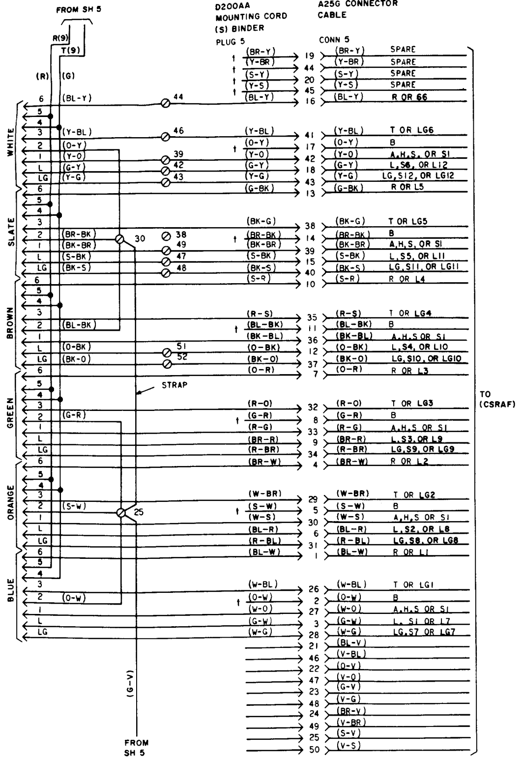
Fig. 1—637EA13 (MD) and 637EAM13 Telephone Set, Connectors (Sheet 6 of 6)
