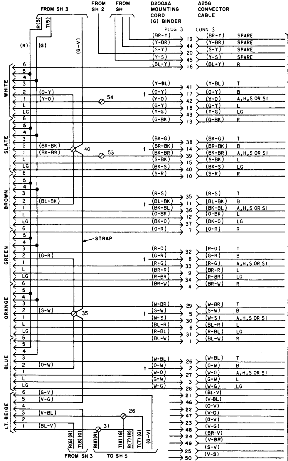
Fig. 1—637EA13 (MD) and 637EAM13 Telephone Set, Connections (Sheet 4 of 6)
