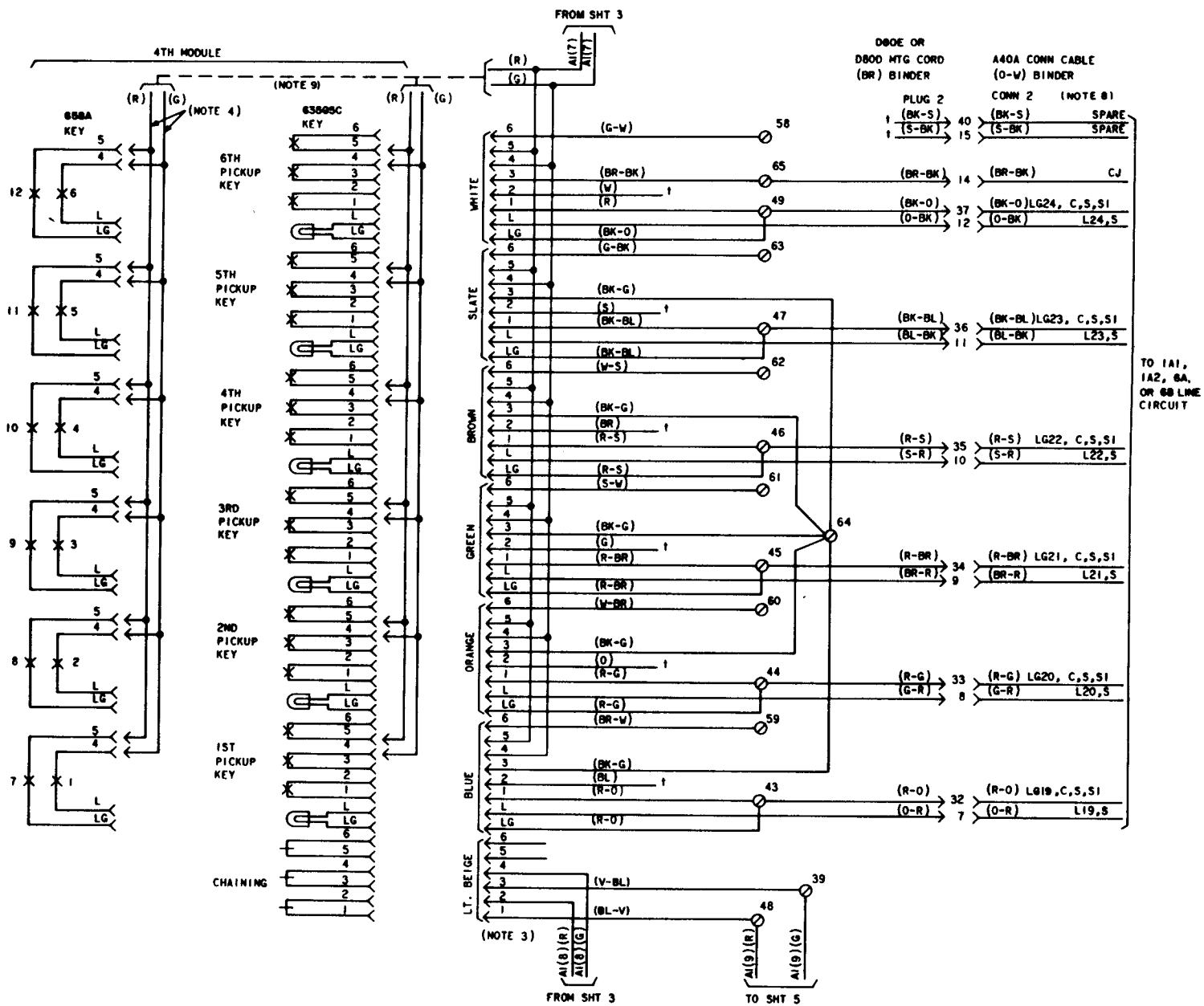
Fig. 5—2639-Type Telephone Set Module and Connector Cable Arrangements (Sheet 4 of 5)†
