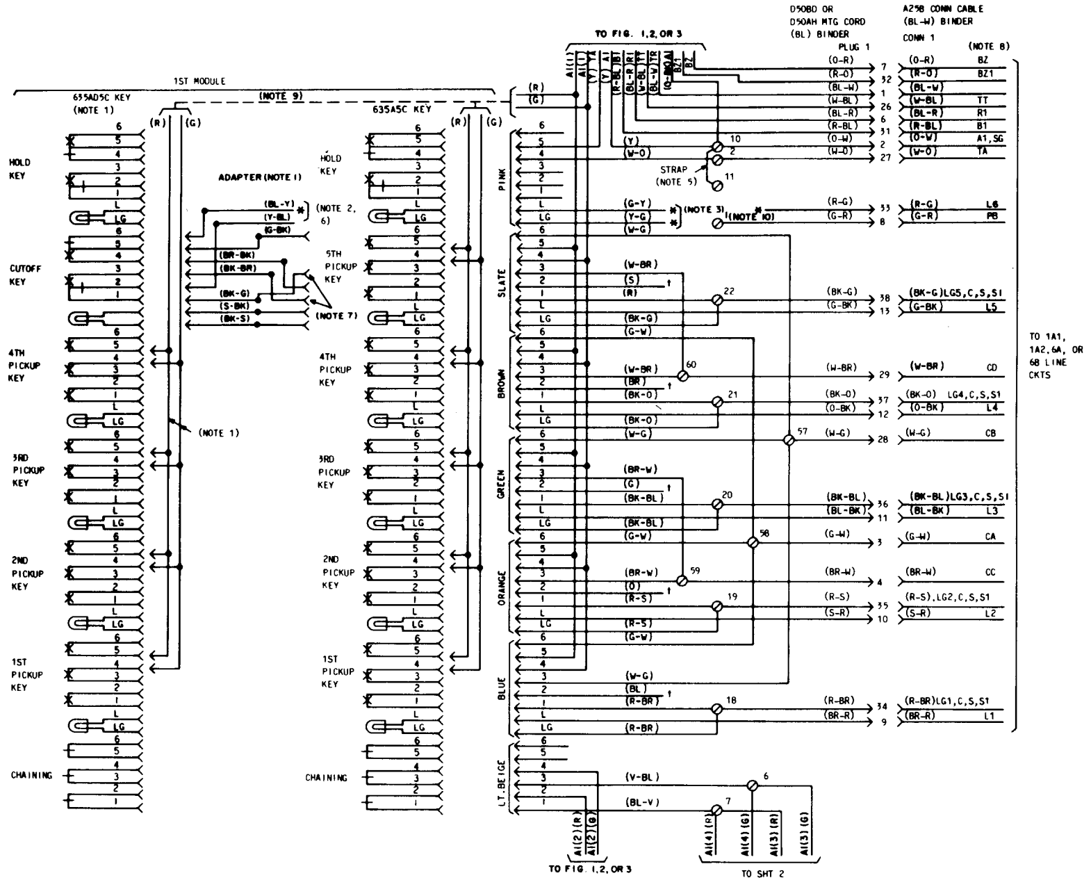
Fig. 4—2638-Type Telephone Set Module and Connector Cable Arrangements (Sheet 1 of 3)
