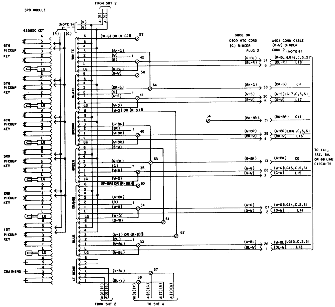
Fig. 5—2639-Type Telephone Set Module and Connector Cable Arrangements (Sheet 3 of 5)
