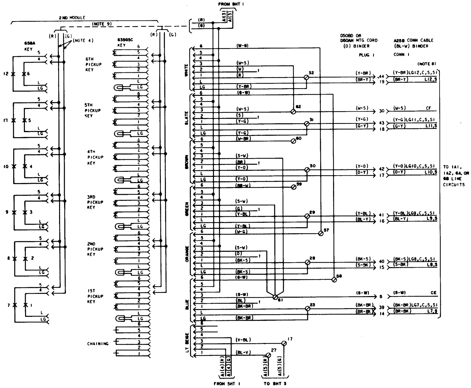
Fig. 4—2638-Type Telephone Set Module and Connector Cable Arrangements (Sheet 2 of 3)
