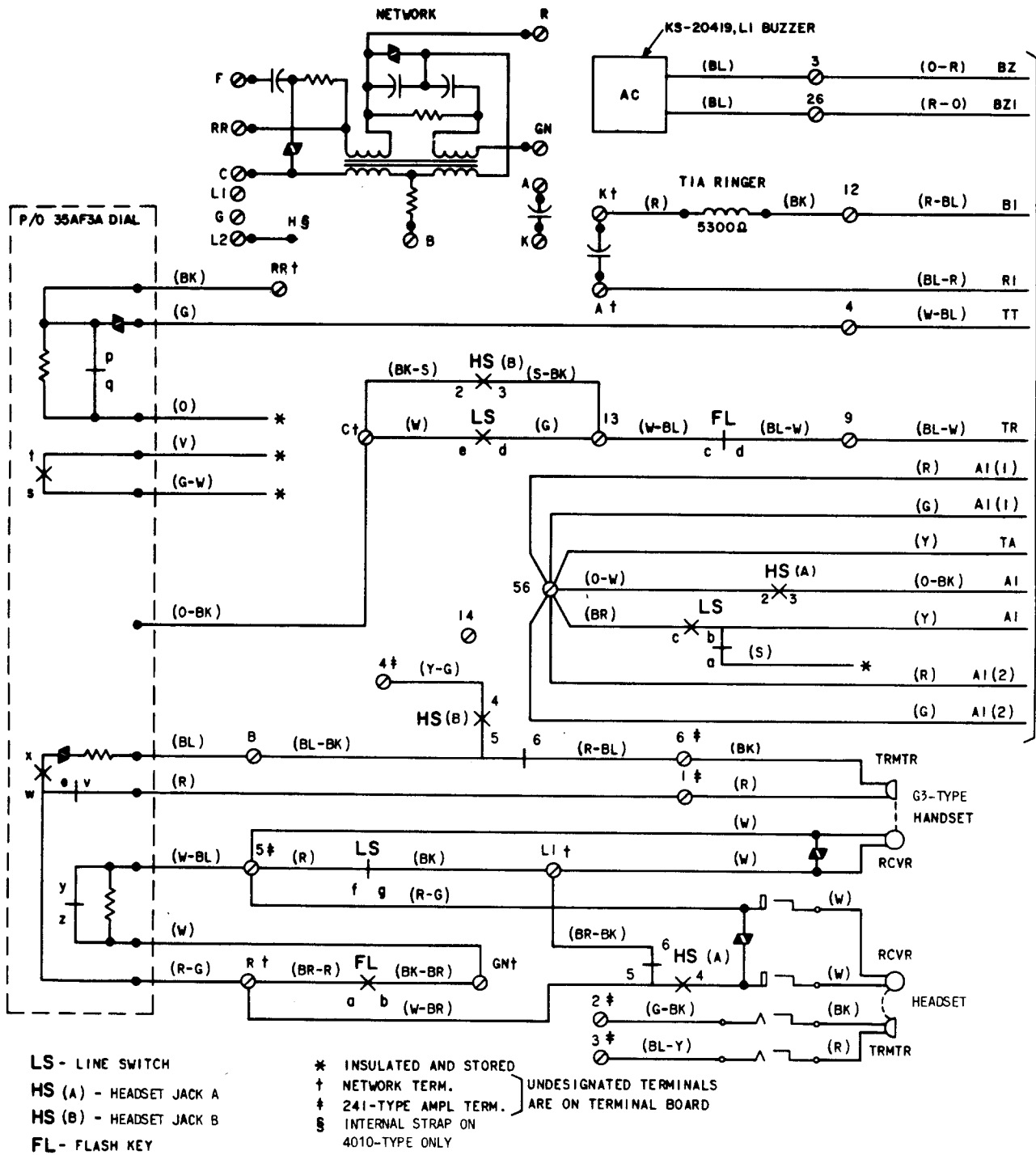
Fig. 1—2638CA and 2639DA Telephone Set, Connections
