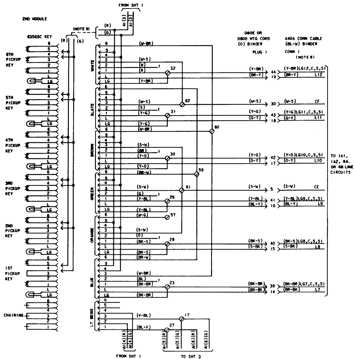
Fig. 5—2639-Type Telephone Set Module and Connector Cable Arrangements (Sheet 2 of 5)
