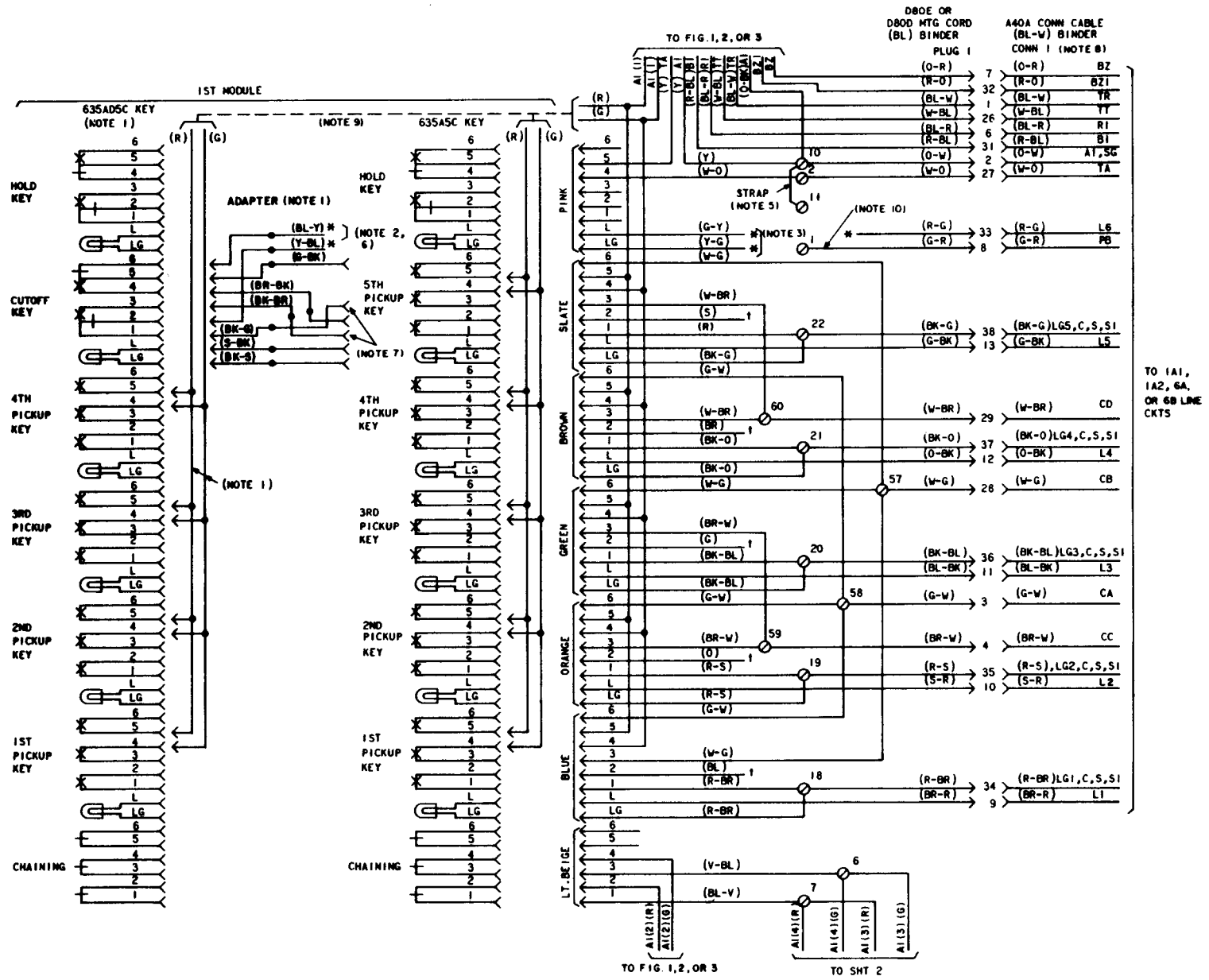
Fig. 5—2639-Type Telephone Set Module and Connector Cable Arrangements (Sheet 1 of 5)
