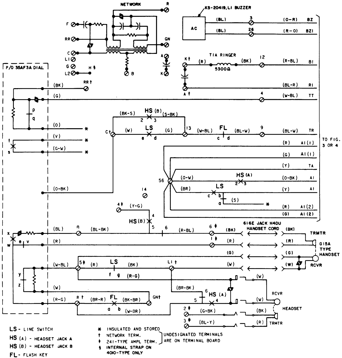
Fig. 2—2638CAM and 2639DAM Telephone Set, Connections
