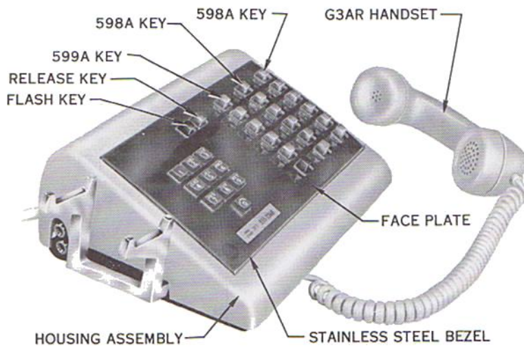
Fig. 6 — 1638-Type Telephone Set with Jacks (Concentrator Use)
