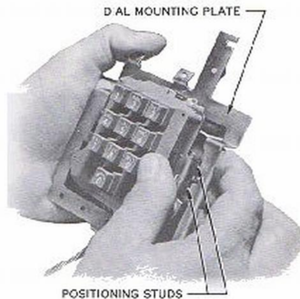
Fig. 26 — Placing Dial on Dial Mounting Plate
