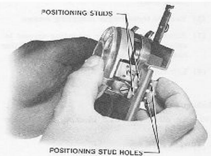
Fig. 29 – Placing Rotary Dial in Dial Mounting Plate
