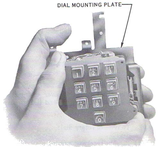
Fig. 24 - Lifting Dial From Dial Mounting Plate
