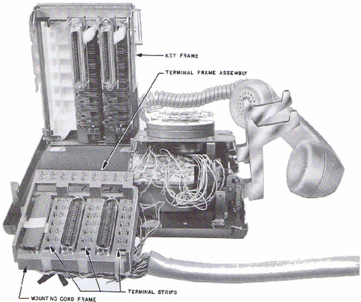
Fig. 20— 630-Type Telephone Set Showing Removal of Cord Frame
