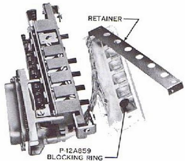
Fig. 31 – Method of Placing Blocking Ring
