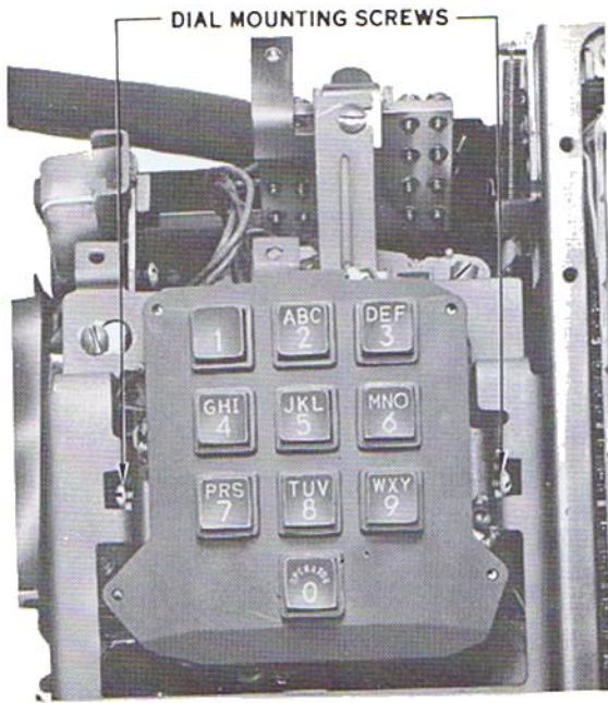
Fig. 21 - 1630-Type Telephone Set, Dial Mounting Screws
