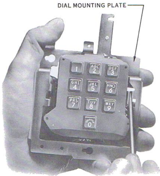
Fig. 22 - Removing TOUCH-TONE Dial From Dial Mounting Plate
