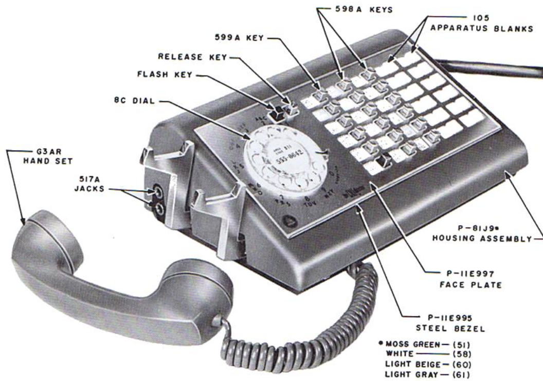
Fig. 14 - 639-Type Telephone Set
