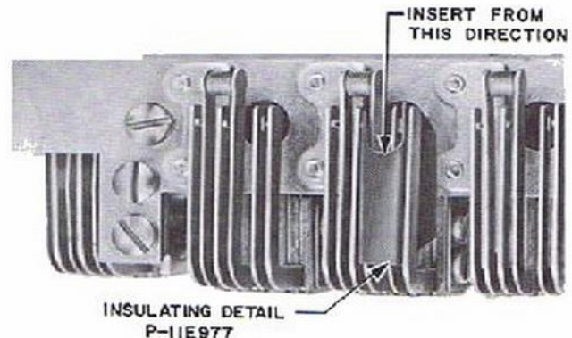
Fig. 32 – Part of 590 Series Key with P-11E977 Insulating Detail when Converted for Signaling
