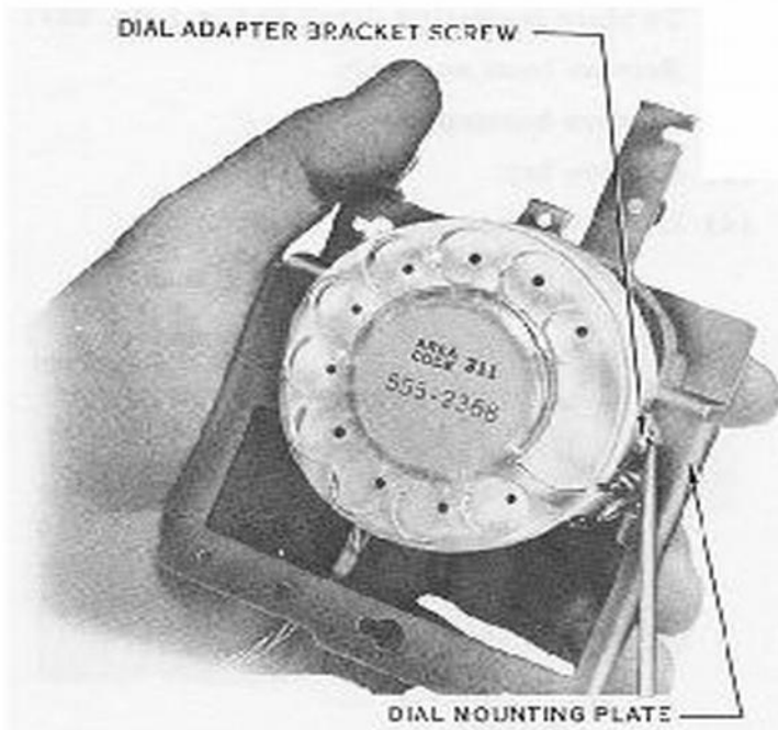
Fig. 27 – Holding Dial and Dial Mounting Bracket
