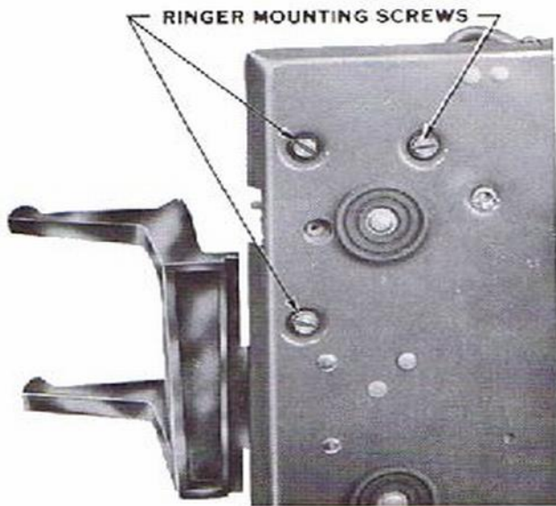
Fig. 30 – Method of Removing Ringer
