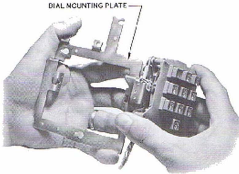
Fig. 25 — Holding Dial and Dial Bracket for Dial Replacement
