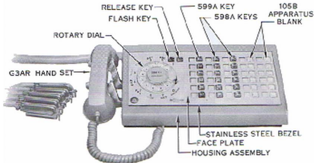
Fig. 1 — 637-Type Telephone Set with Jacks (All Purpose)
