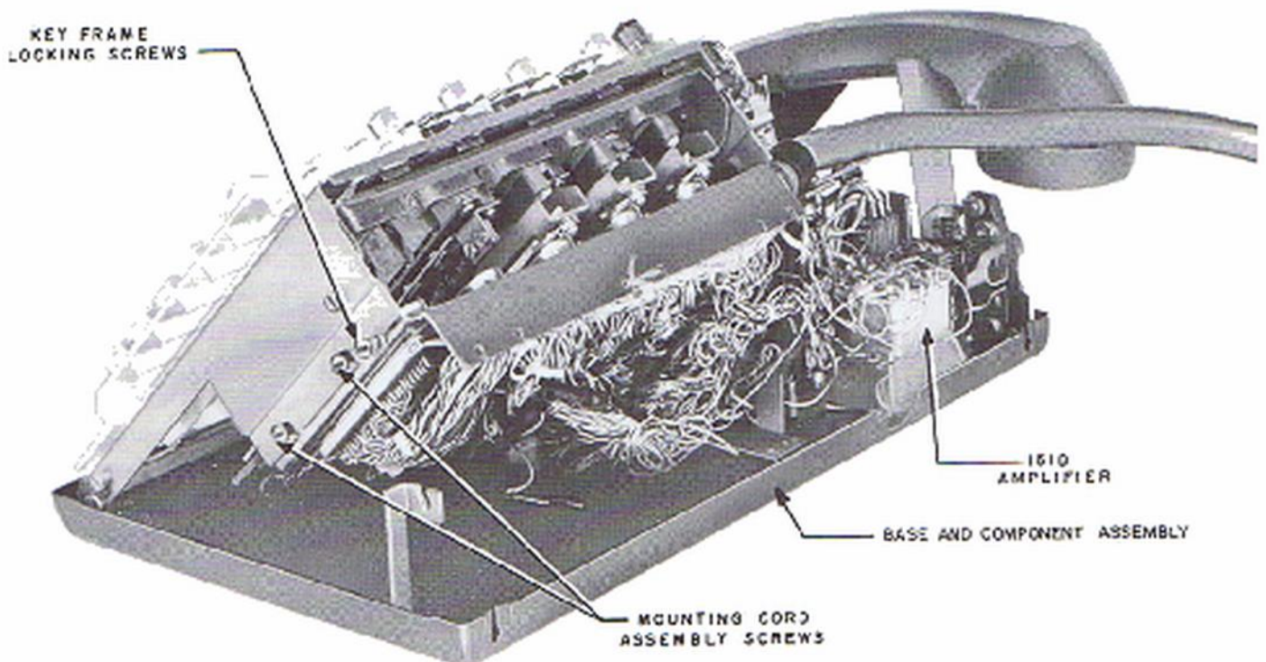
Fig. 19 — 639-Type Telephone Set, Key Frame Lifted, Rear View
