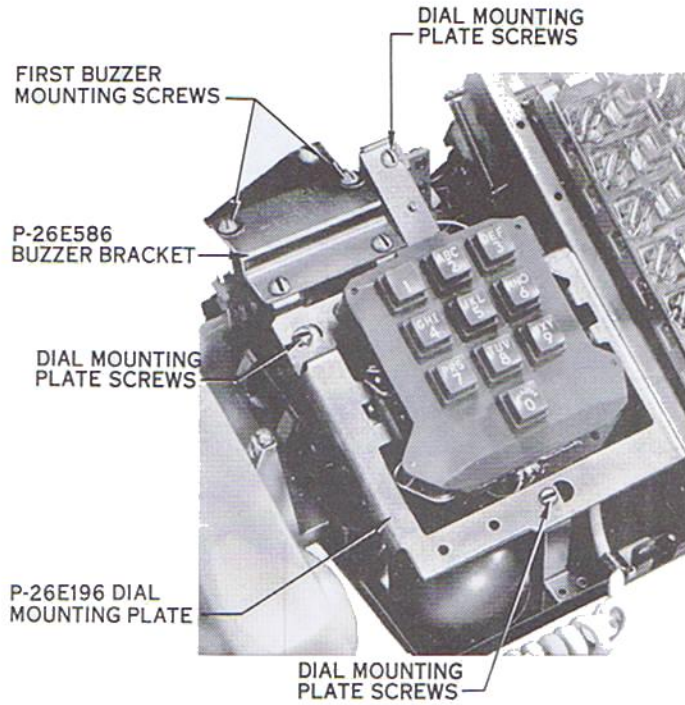
Fig. 11 - 1630-Type Telephone Set
