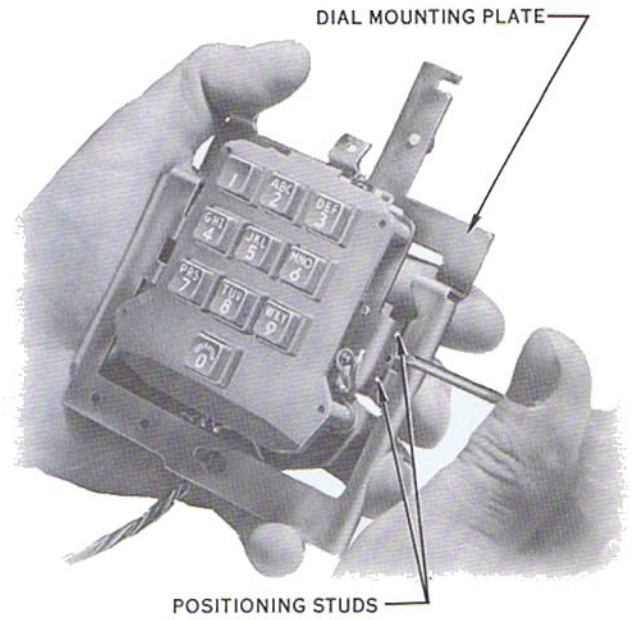
Fig. 23 - Removing Dial From Dial Mounting Plate
