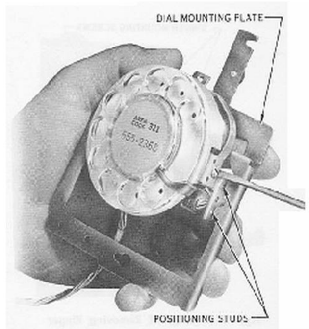
Fig. 28 – Removing Dial from Dial Mounting Plate
