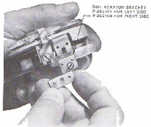
Fig. 10 — Placing Dial Adapter Brackets
