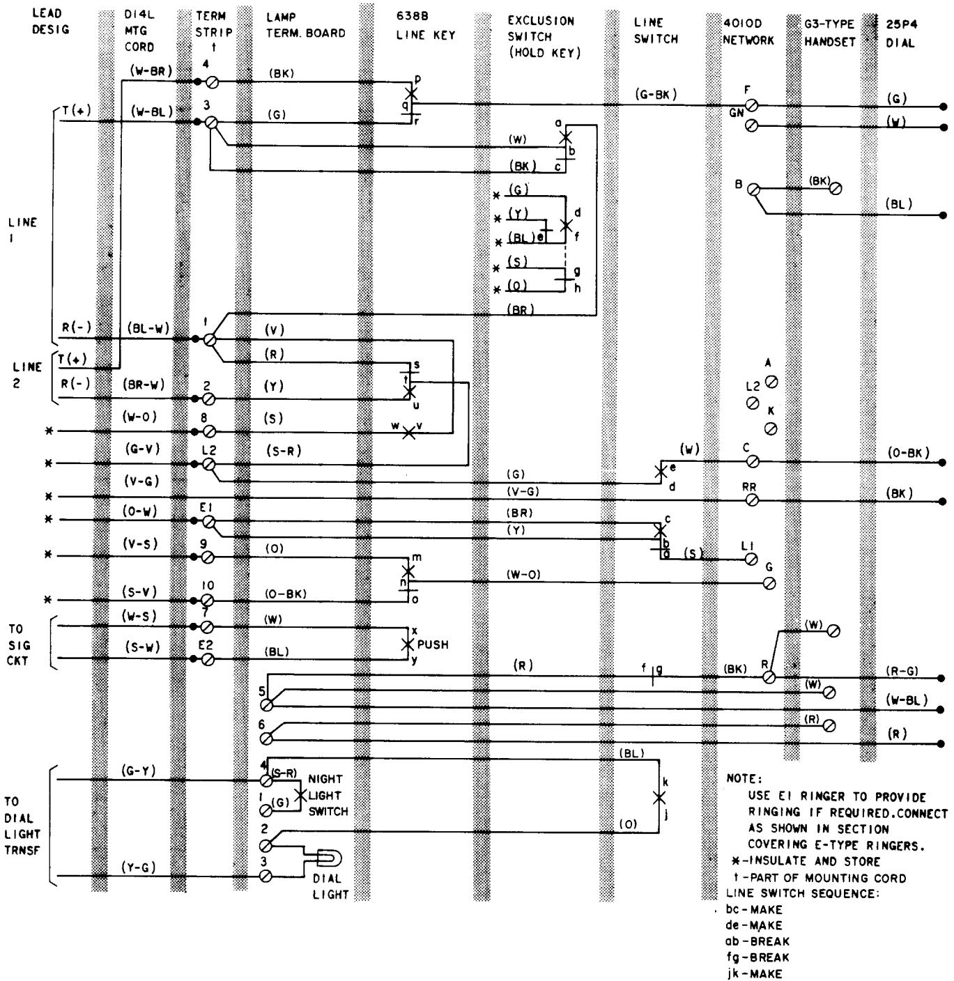
Fig. 1—1712B (MD) Telephone Set Connections Using 25P4 (MD) Dial and 4010D Network—Wired for 2-Line Pickup, Hold on Line 1, and Signaling
