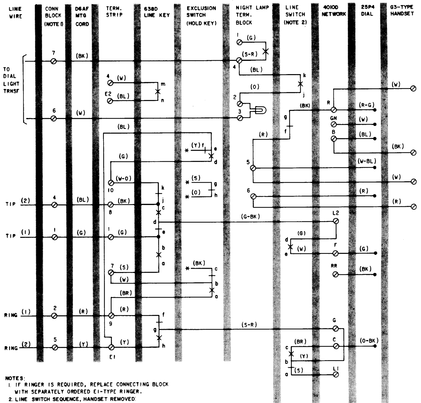
◆Fig. 2—1713B Telephone Set Connections With 25P4 Dial◆
