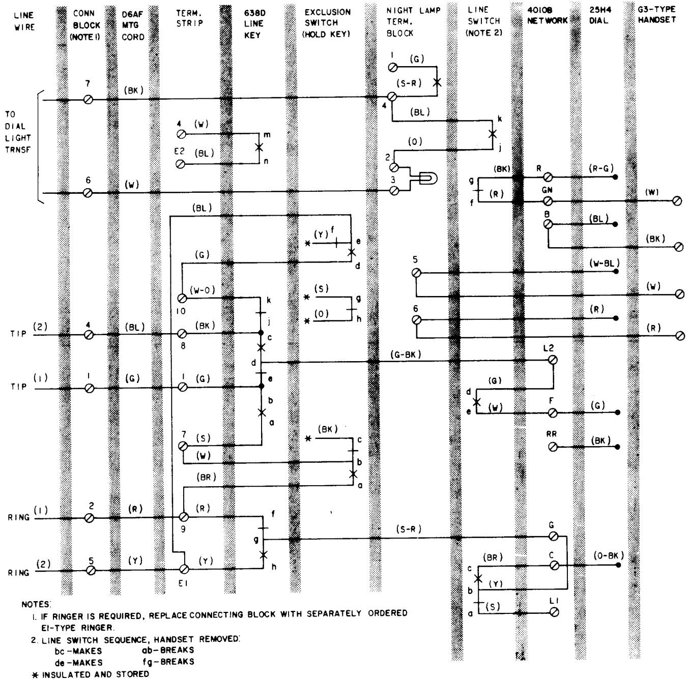
Fig. 1—1713B Telephone Set Connections With 25H4 Dial
