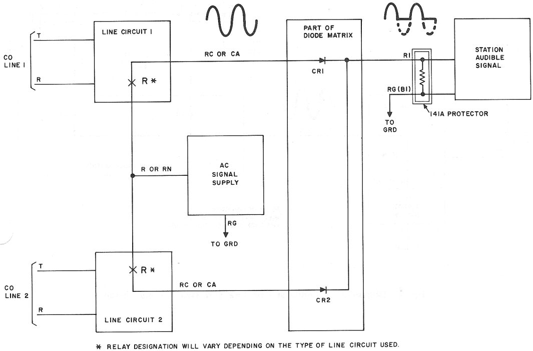
Fig. 1—Simplified Schematic of Two Lines and One Audible Signal
