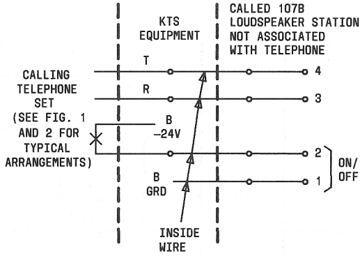
Fig. 3—Example of Standalone Voice-Signaling Arrangement
