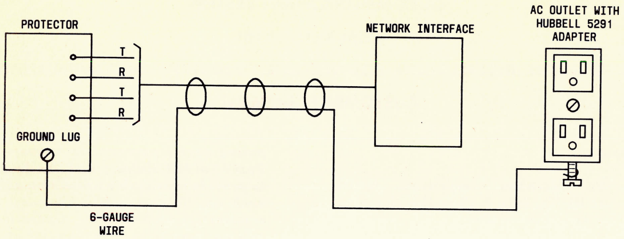
Fig. 9A—Typical Arrangement of Coupled Bonding Conductor
