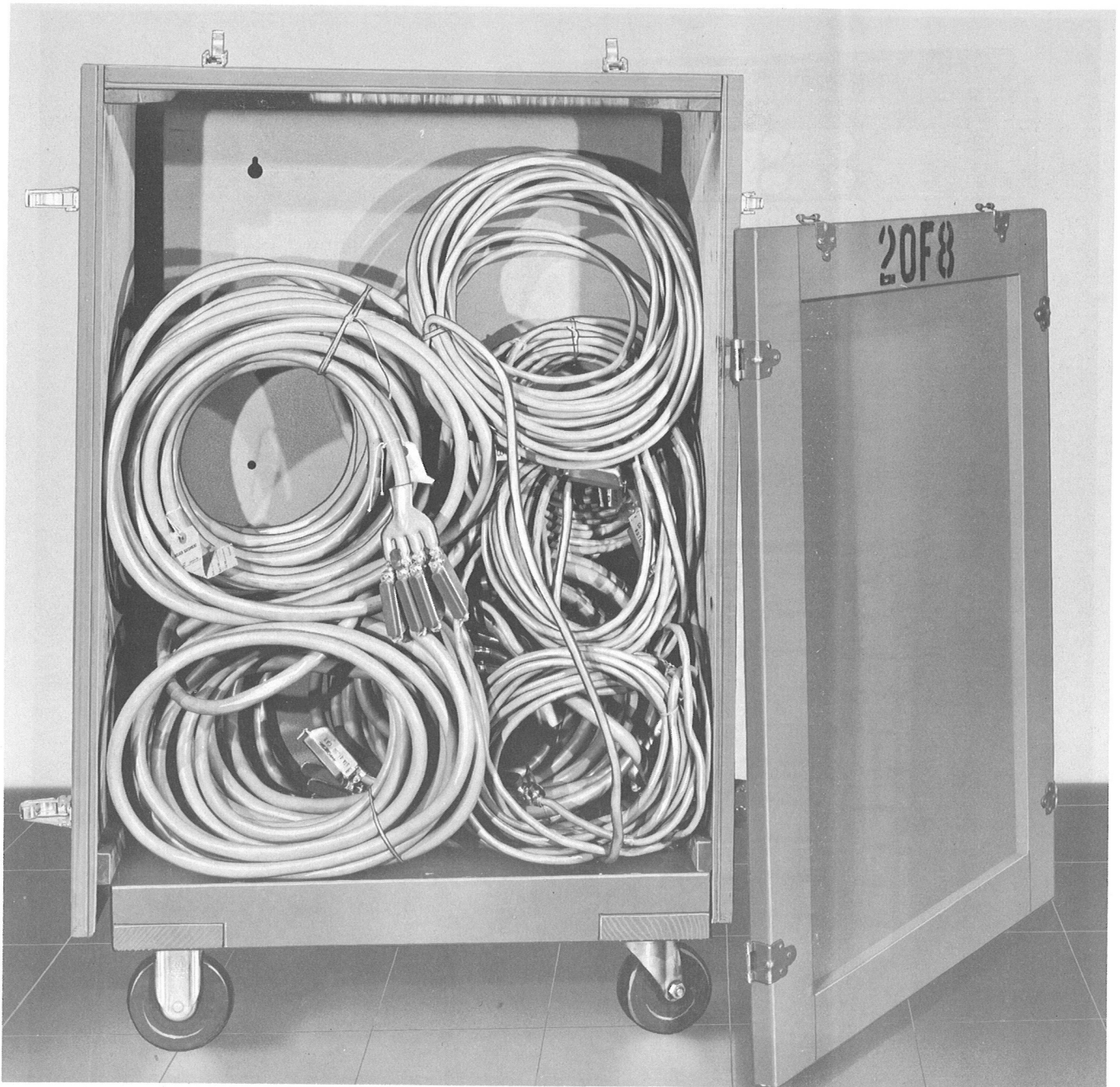
Fig. 8—Cabinet No. 2 Showing Cable Storage
