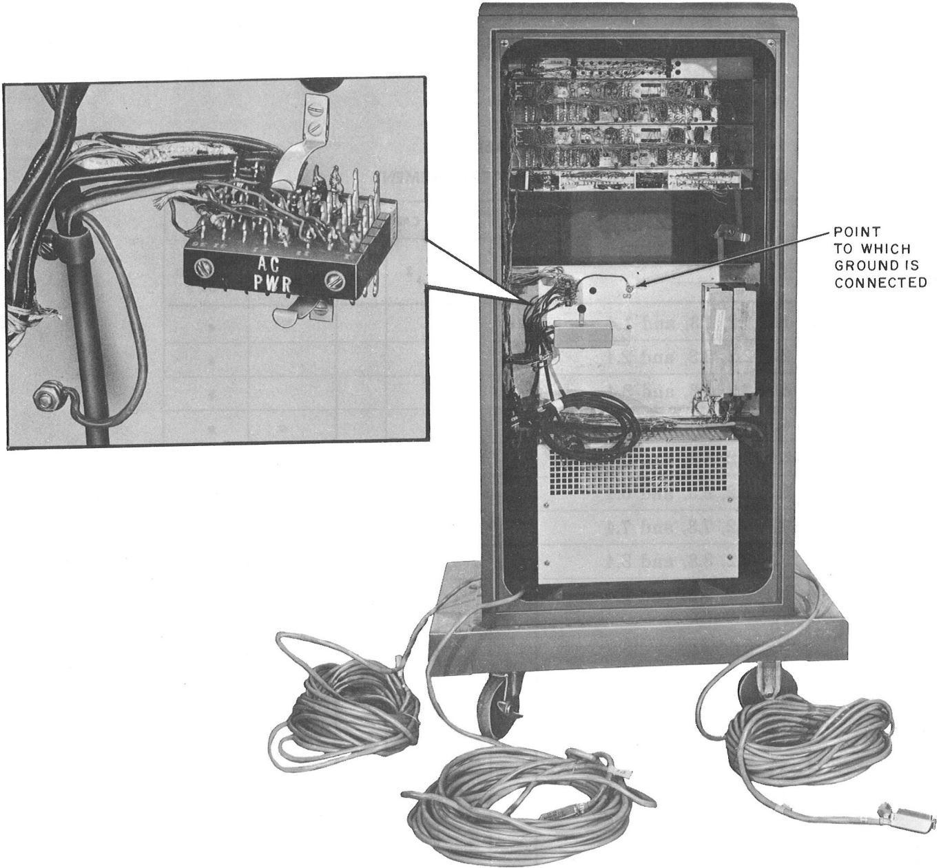
Fig. 13—Cabinet No. 4 Showing Power and Ground Connections
