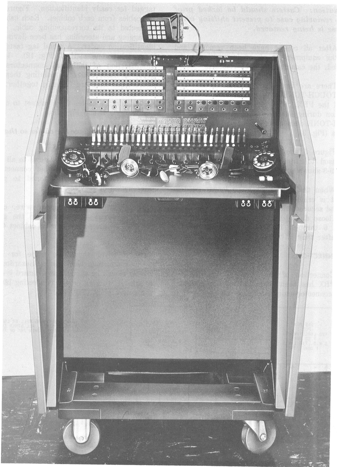
Fig. 4—Position 1 in Case with Cover Removed
