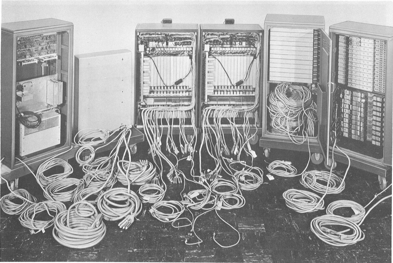
Fig. 11—Complete Equipment Assembly Showing Cables
