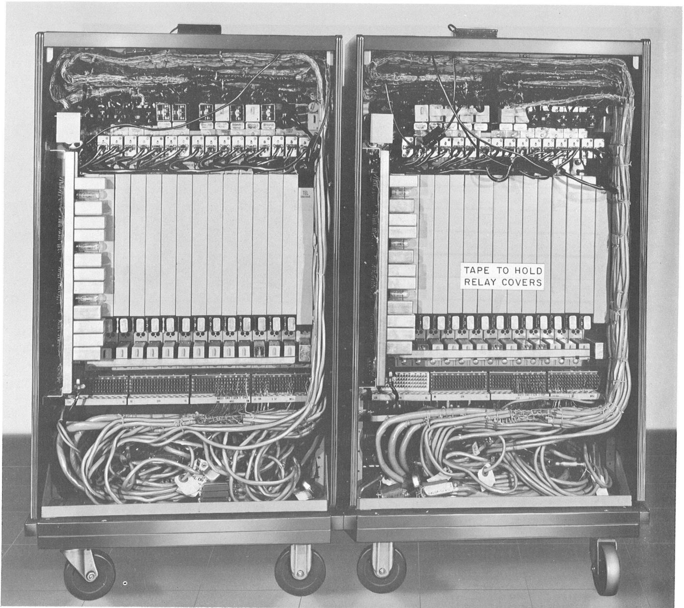
Fig. 6—555 PBX Positions, Rear View
