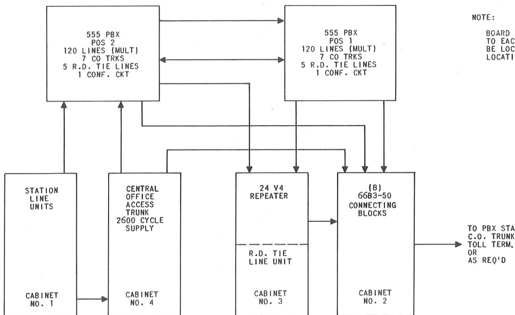
Fig. 5—Block Diagram for Specially Modified 555 PBX
