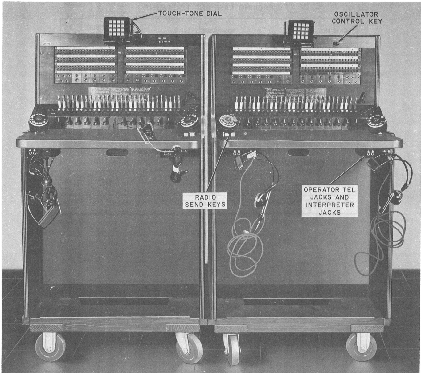
Fig. 3—555 Switchboard Positions 1 and 2
