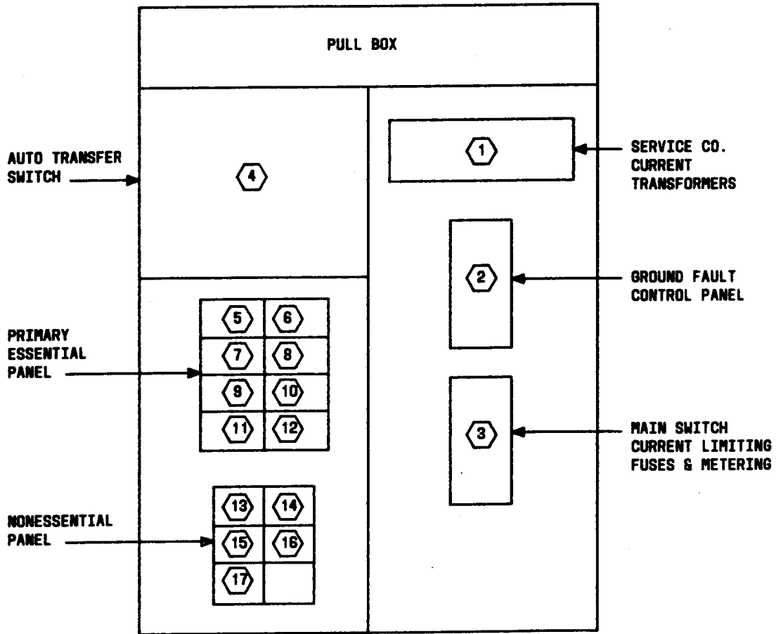
Fig. 1 — Main Switchboard Elevation
