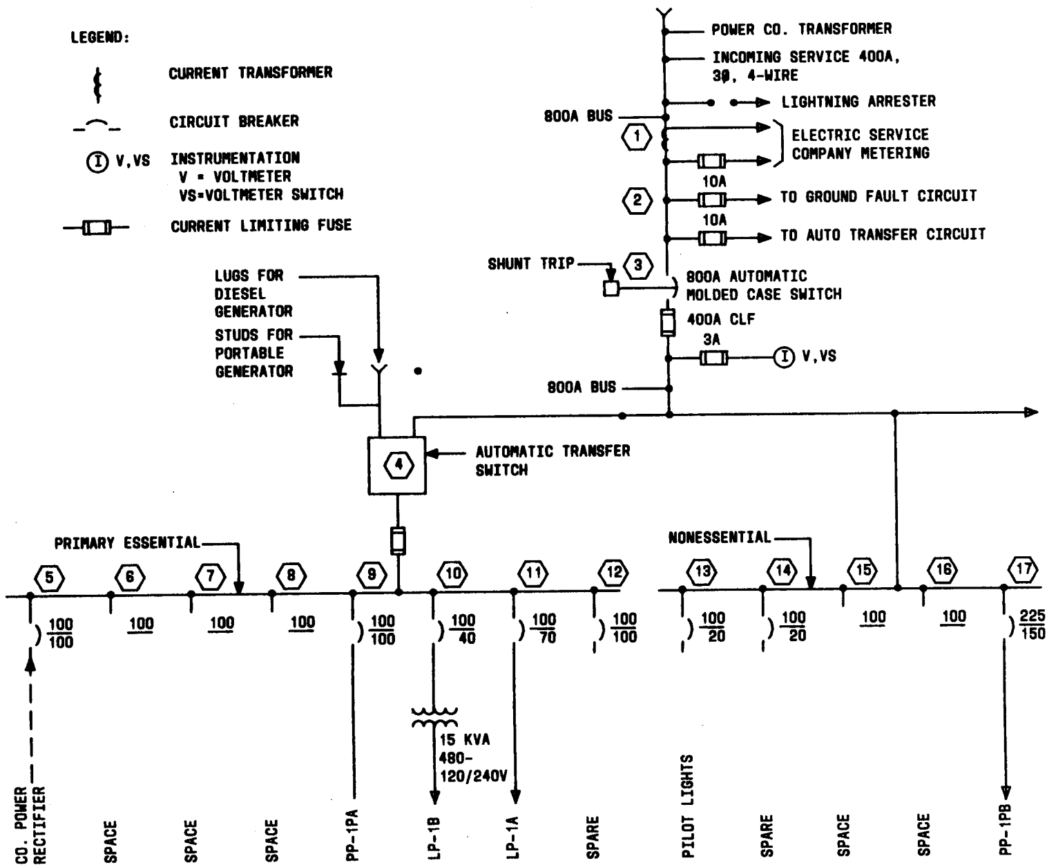
Fig. 2—One-Line Diagram
