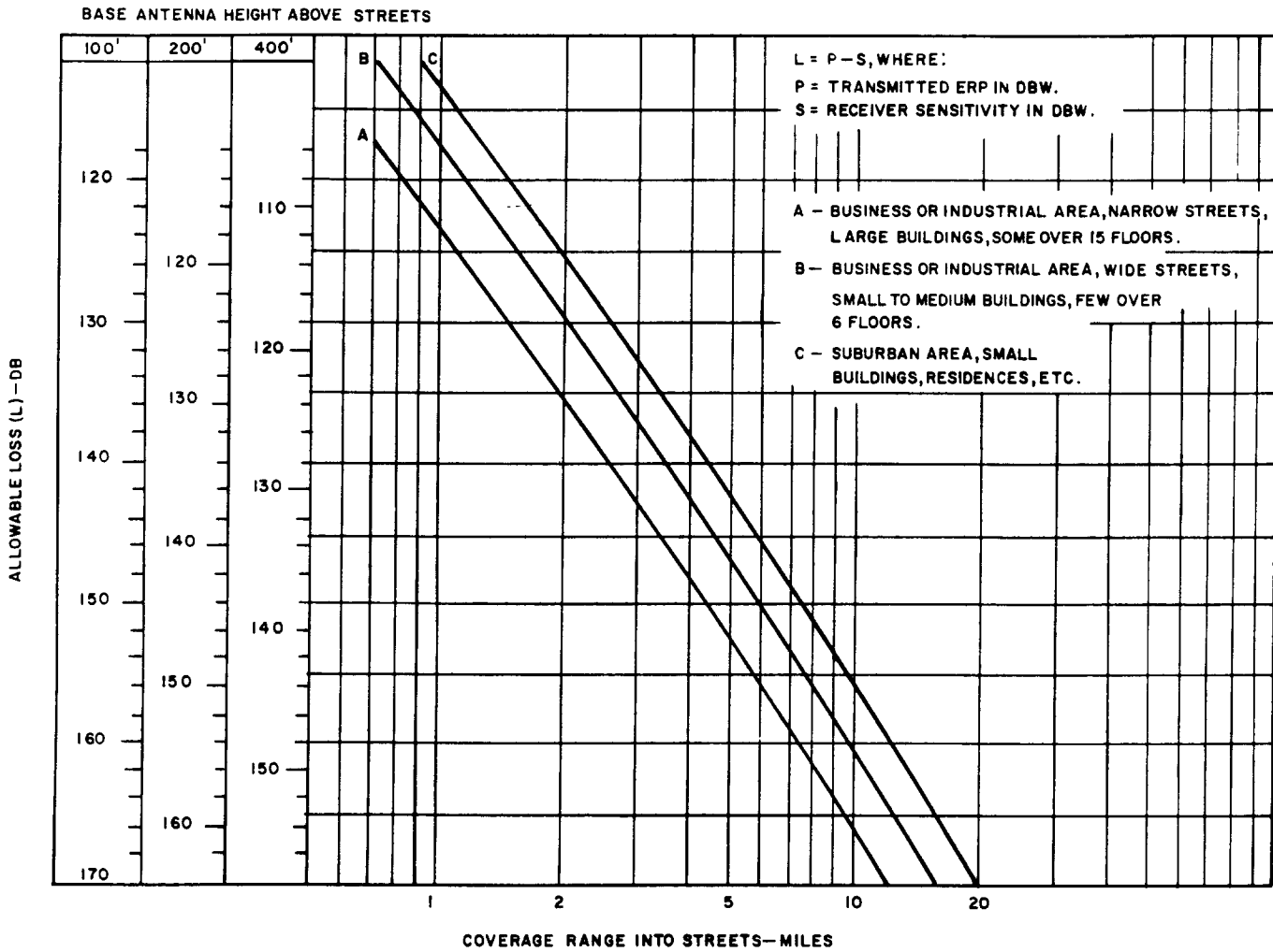
Fig. 6—Peripheral Area Coverage on Streets—150-MHz BELLBOY
