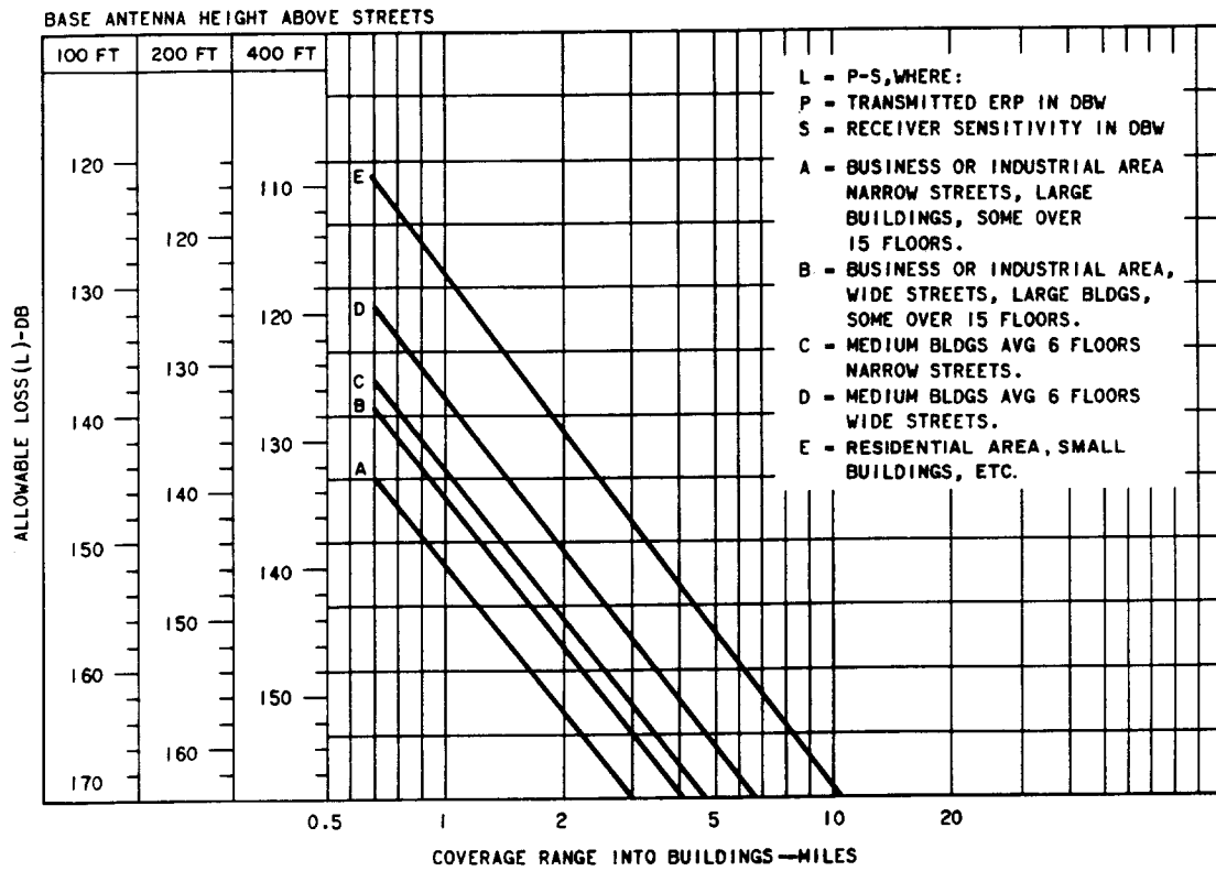
Fig. 5—Primary Service Area Coverage Within Buildings—150-MHz BELLBOY
