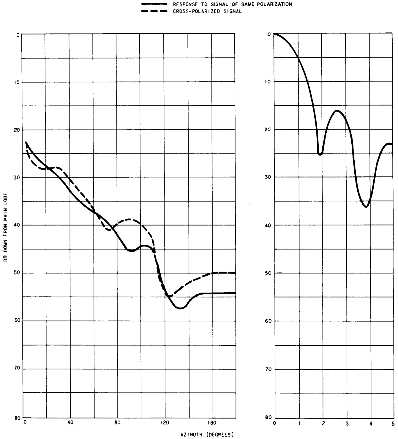
Fig. 1—Smoothed Horizontal Directivity—6 GHz
