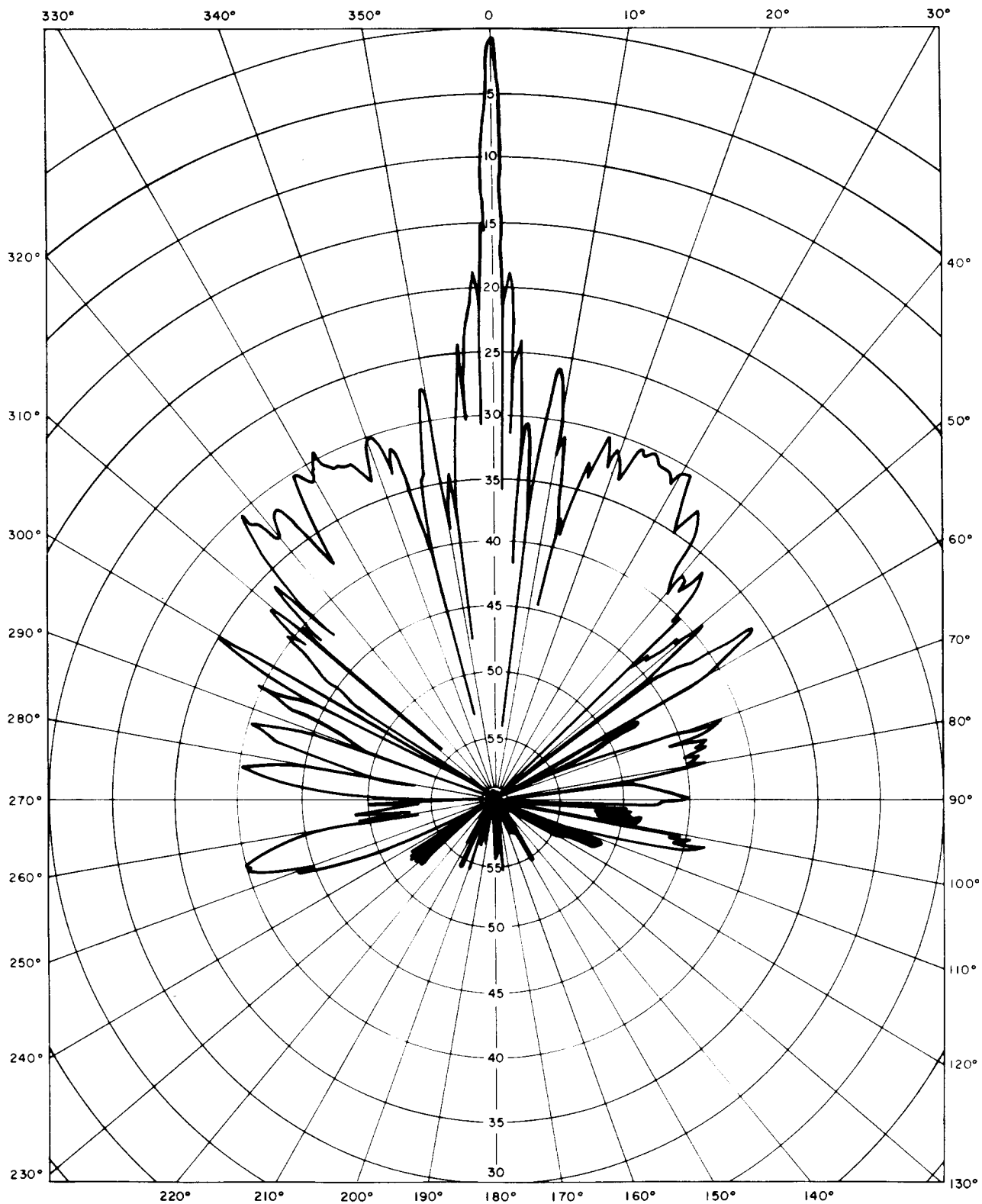
Fig. 3—Radiation Pattern for 6.175 GHz Horizontally Polarized Signal
