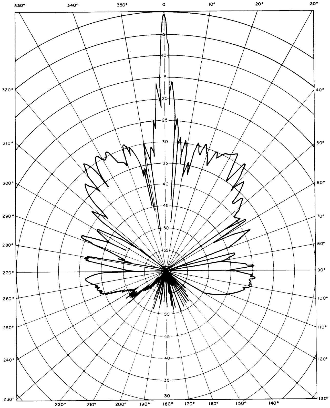
Fig. 4—Radiation Pattern for 6.175 GHz Vertically Polarized Signal
