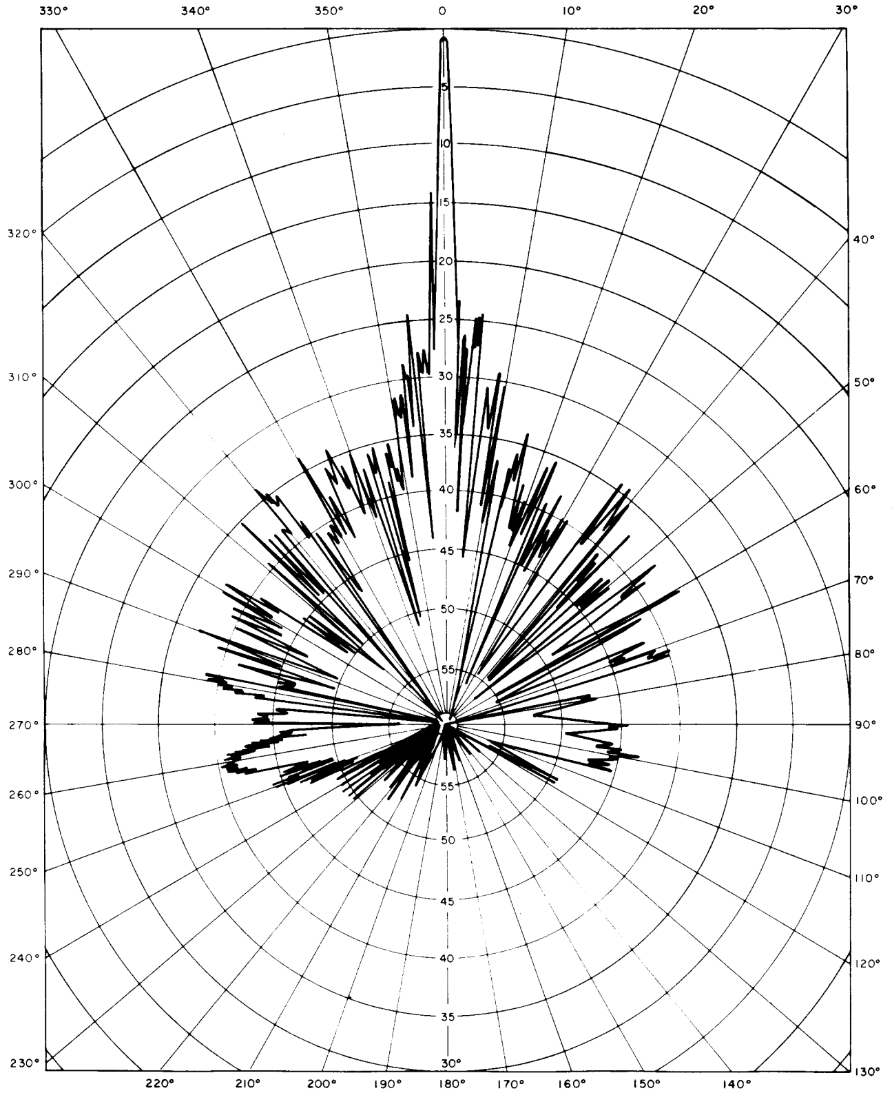
Fig. 5—Radiation Pattern for 11.2 GHz Horizontally Polarized Signal
