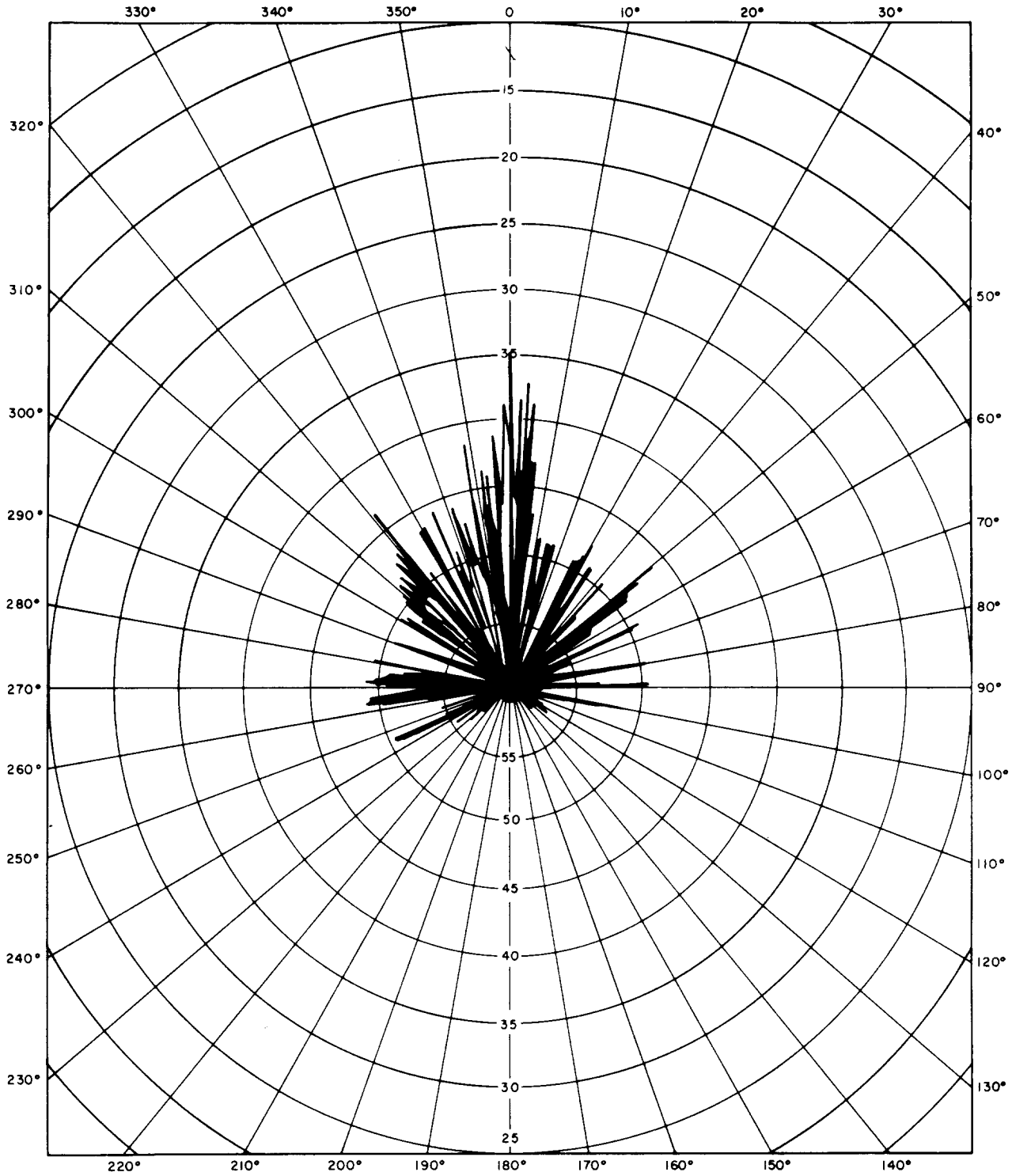
Fig. 8—Response to a Cross-Polarized 11.2 GHz Signal
