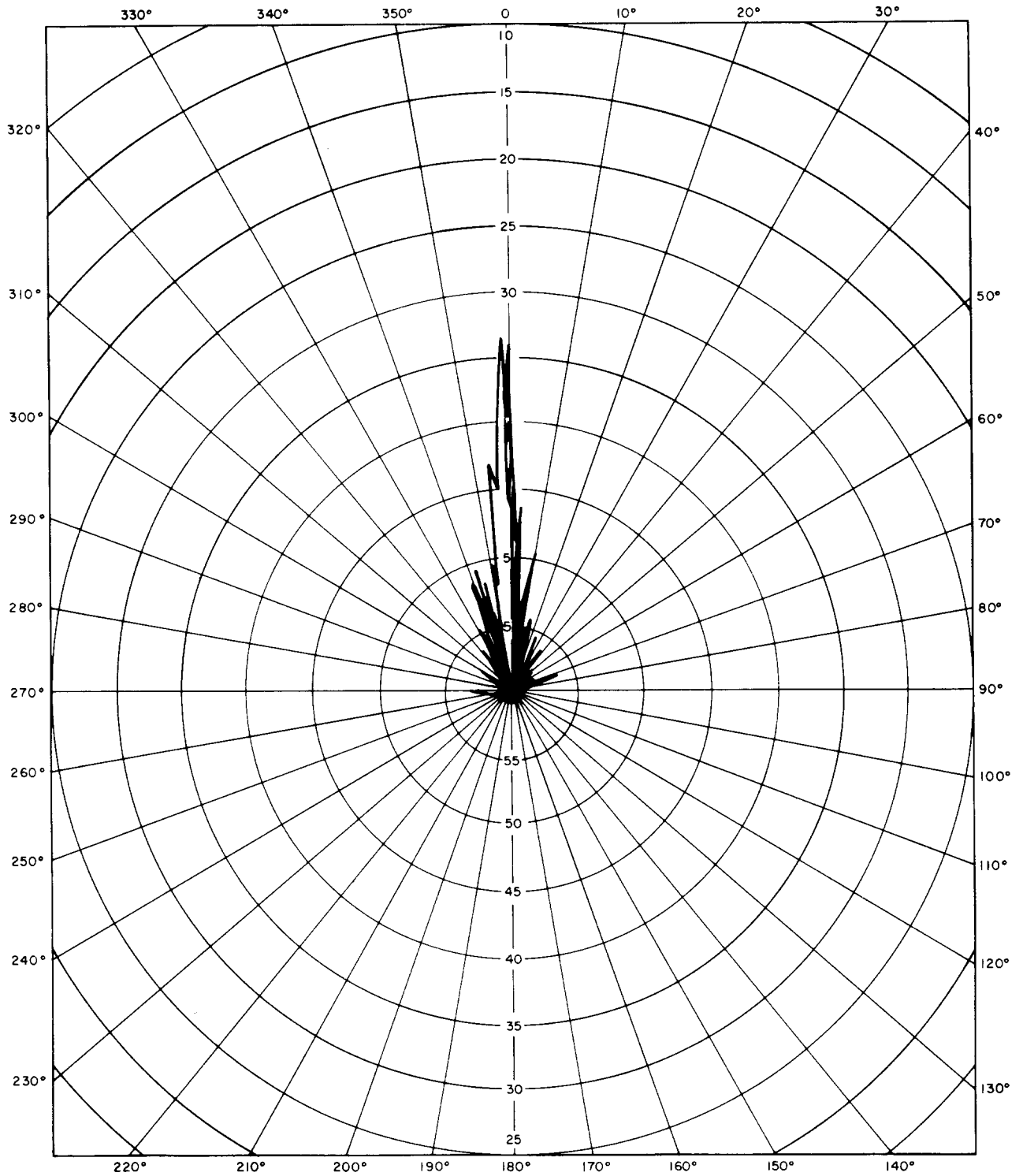
Fig. 7—Response to a Cross-Polarized 6.175 GHz Signal
