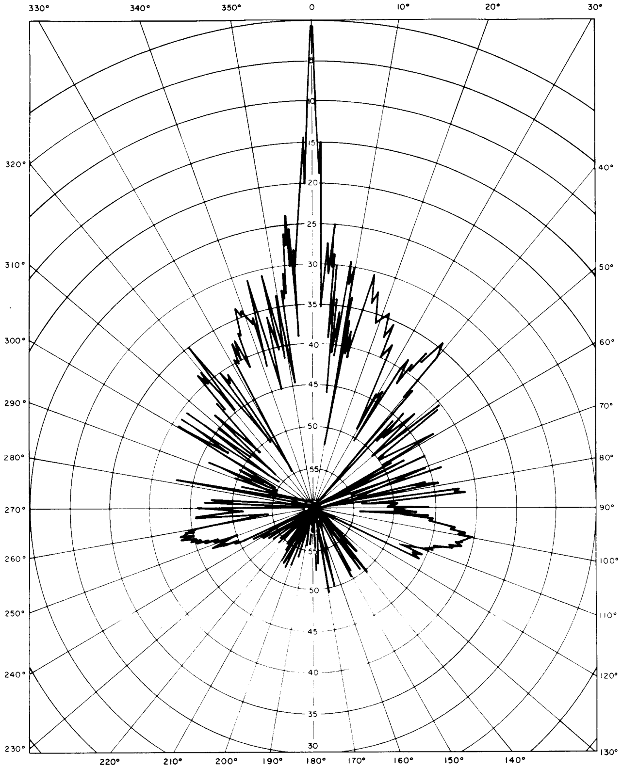
Fig. 6—Radiation Pattern for 11.2 GHz Vertically Polarized Signal
