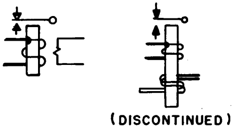
(c) Relay with noninductive winding and transfer contacts
