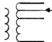
(7) Load-ratio control transformer with taps
