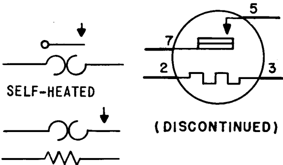
(l) Thermostat-type relay
