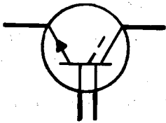
(o) N-P-I-N transistor with ohmic connection to the intrinsic region
