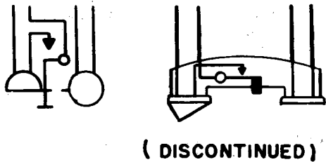
(c) 4-conductor handset with push-to-talk switch
