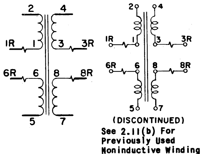
(13) Repeating coil with taps
