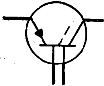
(o) N-P-I-N transistor with ohmic connection to the intrinsic region
