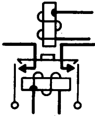
(g) Mechanically locking and electrically releasing relay
