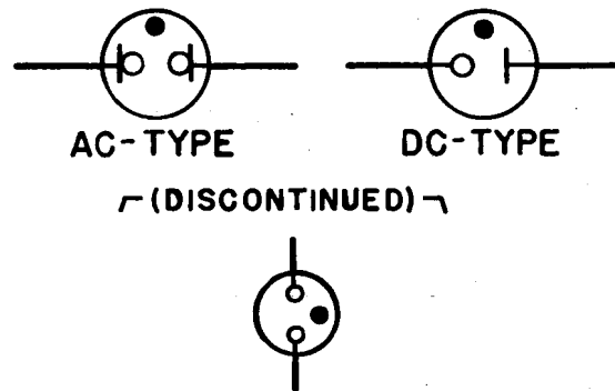
(e) Glow-type lamp
