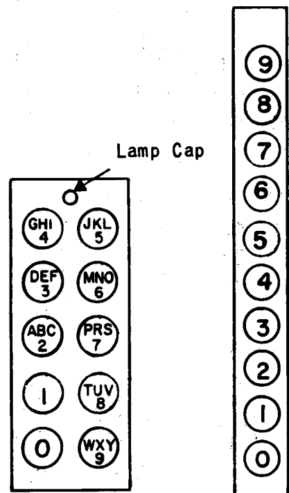
(b) Push-button-type keytop diagrams (See note)
