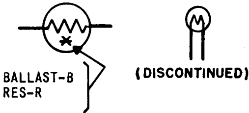
(b) Double-filament ballast or resistance lamp
