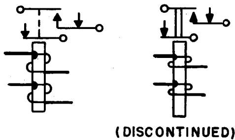
(b) Double-wound relay with break and make-before-break contacts
