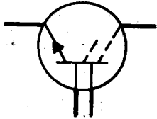
(q) N-P-I-P transistor with ohmic connection to the intrinsic region
