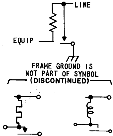
(b) Protector-type heat coil
