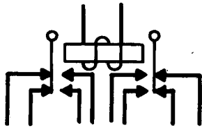
(k) Thermal delay relay (Also see 4.59)
