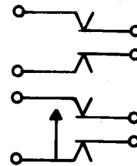
(10) Spring-type jack and plug (engaged)
