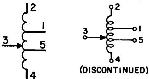
(3) Application (Variable tap-type autotransformer)
