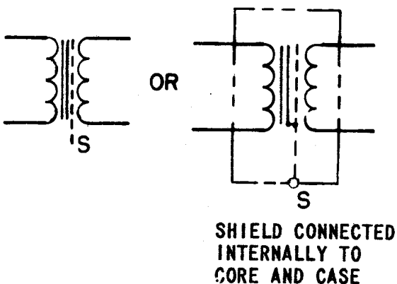
(2) With magnetic core and shield
