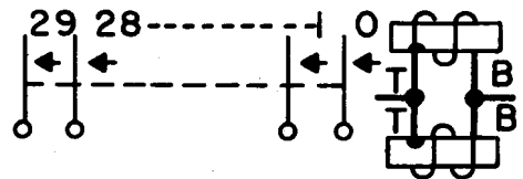
(1) Nonsplit multicontact relay
