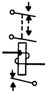
(e) Relay in normally operated position
