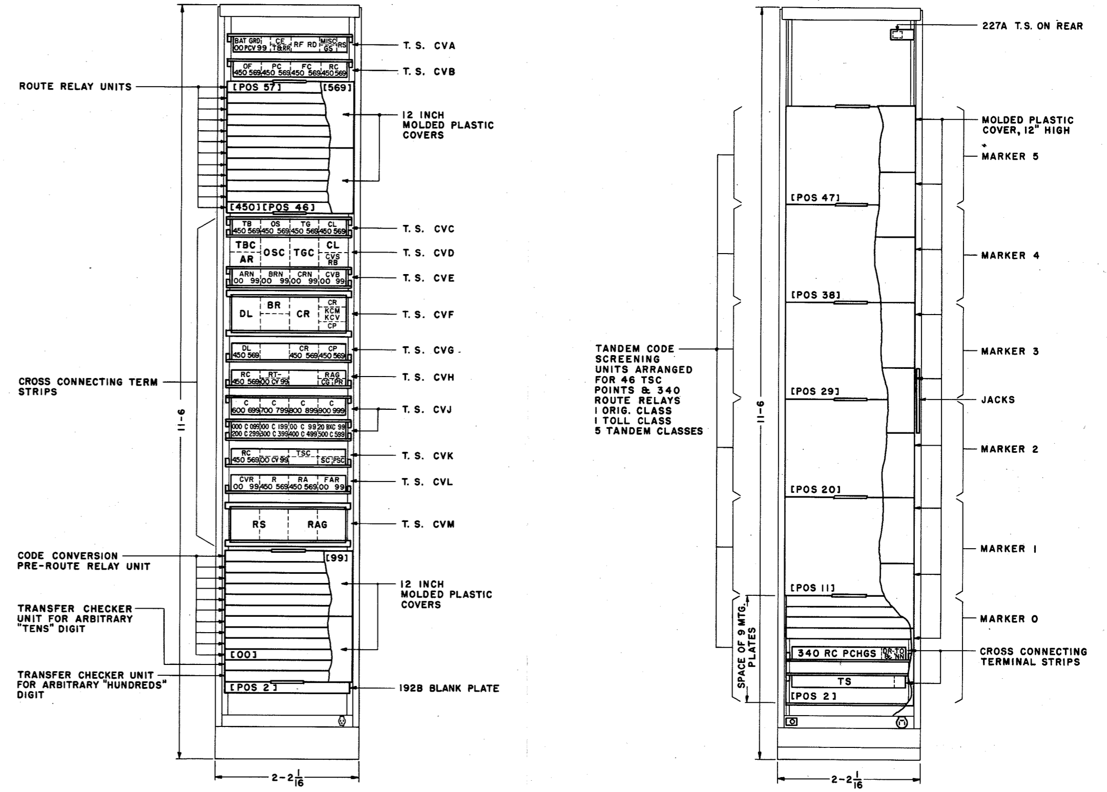
CODE CONVERSION AND ROUTE RELAY FRAME
