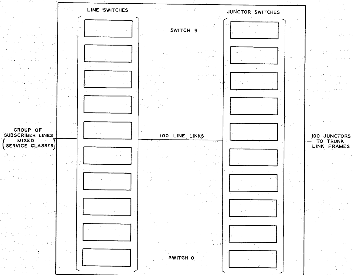
Fig. 3 - Line Link Frame
