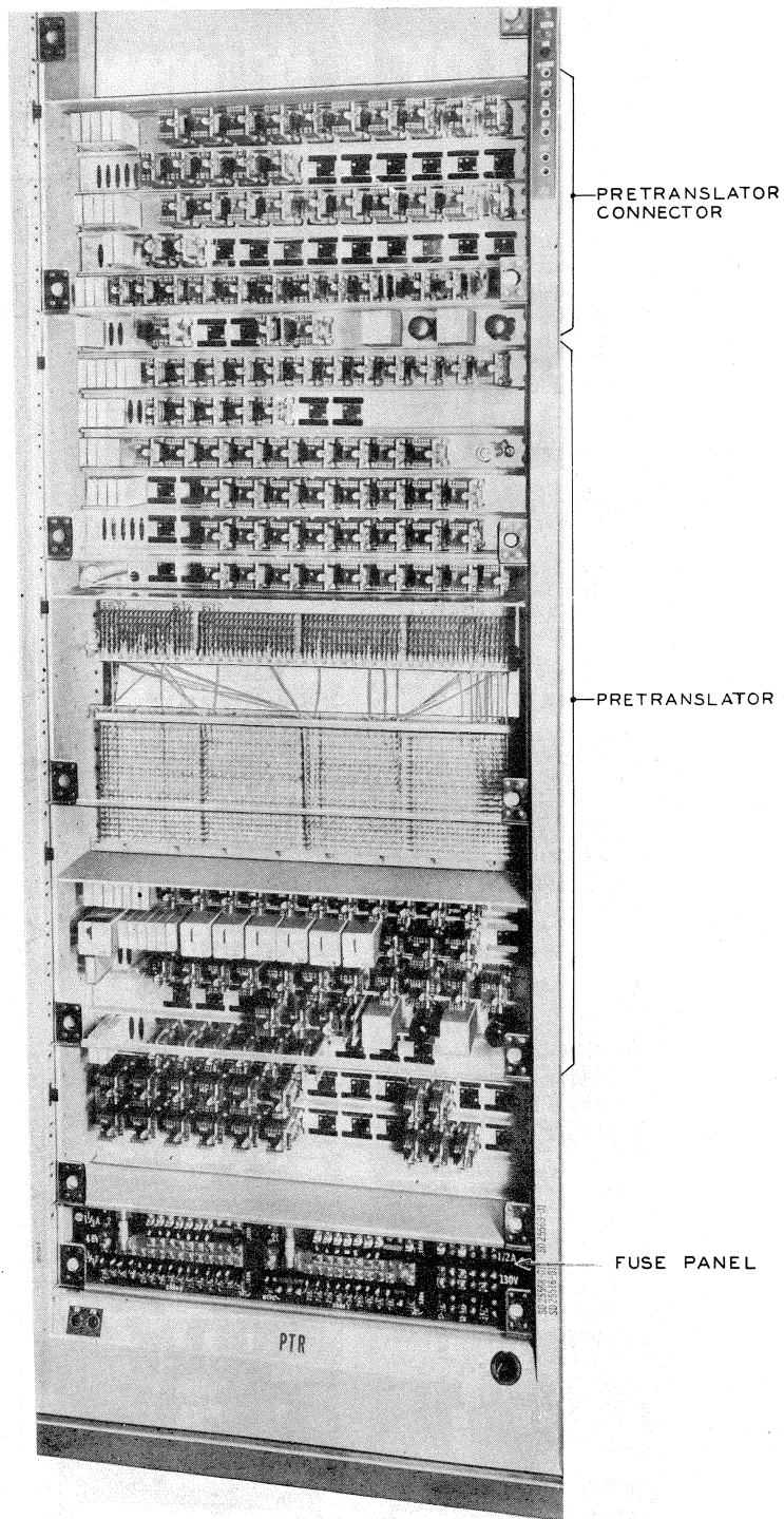
FIG. 21 PRETRANSLATOR AND PRETRANSLATOR CONNECTOR FRAME
