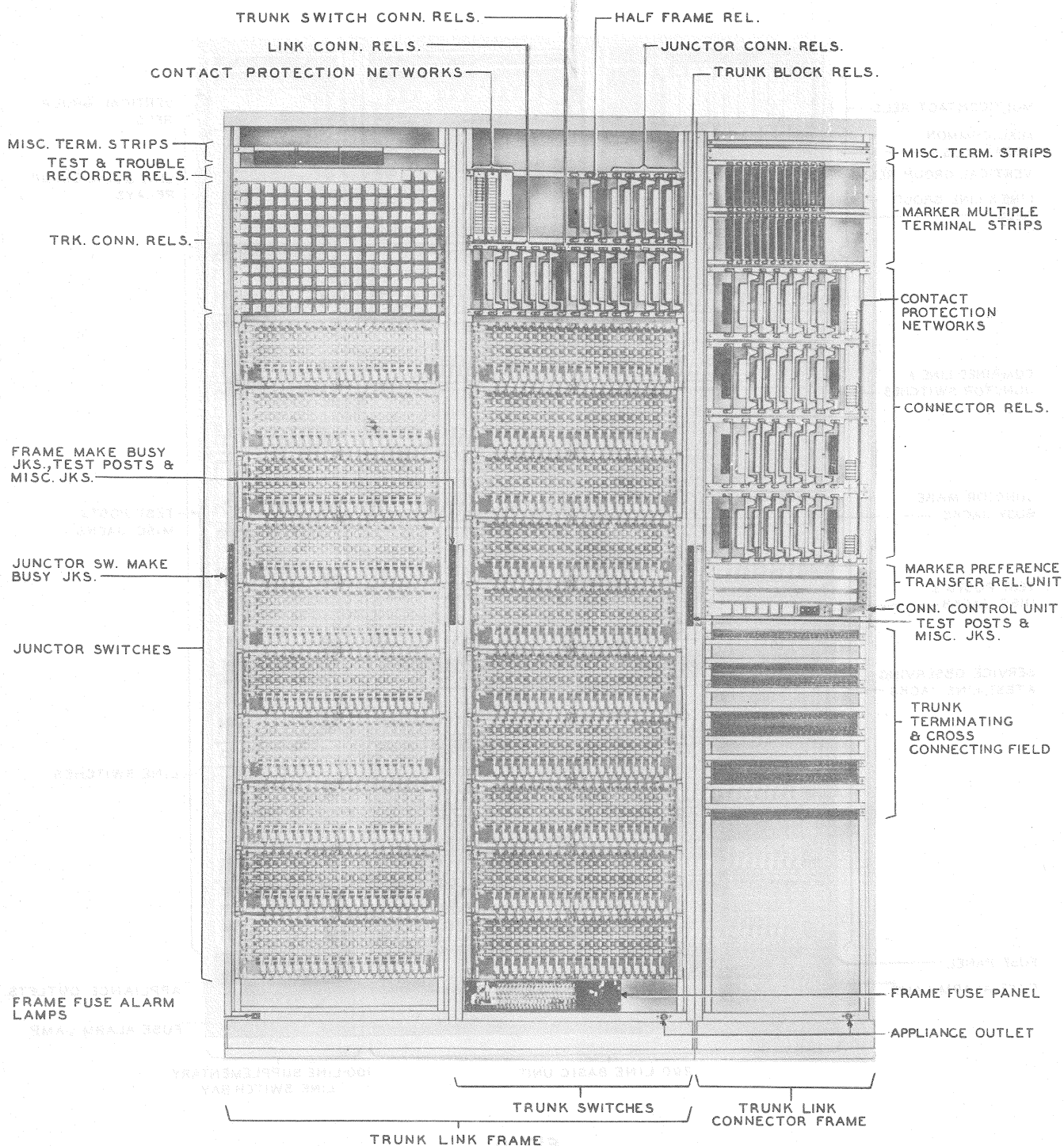
FIG. 12 TRUNK LINK FRAME AND TRUNK LINK CONNECTOR FRAME
