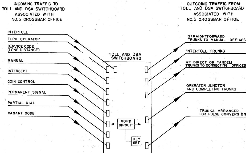
Fig. 46 - Traffic at a Combined Toll and DSA Switchboard Associated With a No. 5 Crossbar Office
