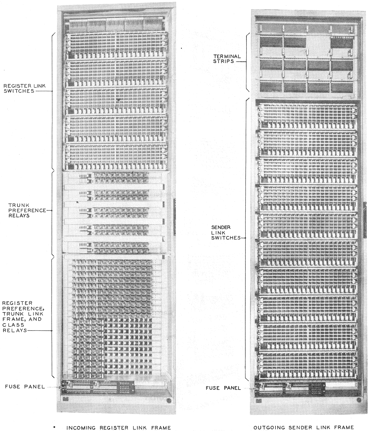
FIG. 24 REGISTER AND SENDER LINK FRAMES
