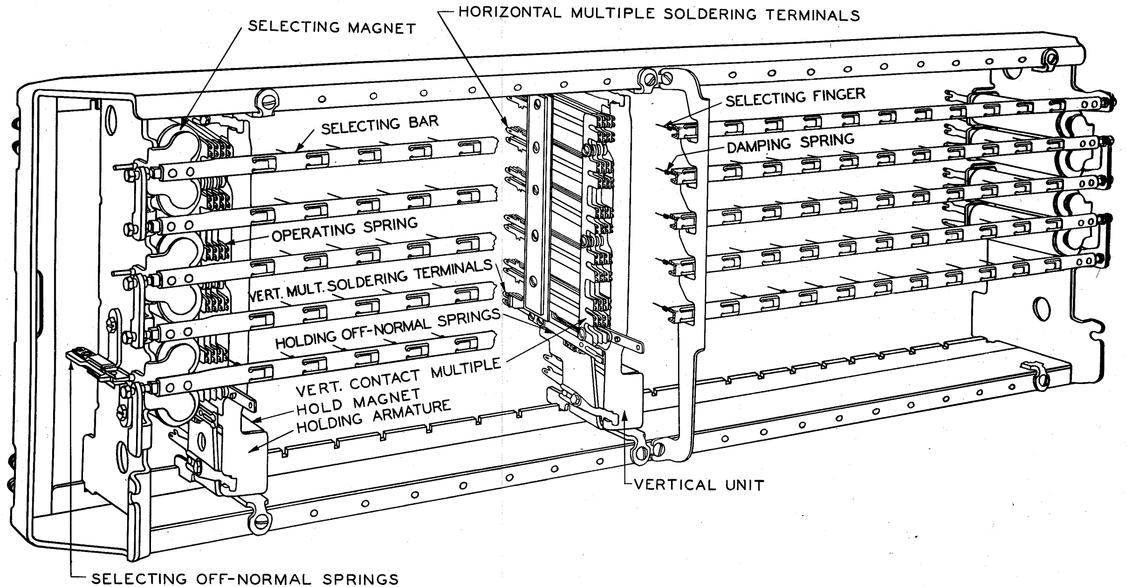
FIG. 1 PARTIAL PERSPECTIVE VIEW OF 20-VERTICAL UNIT CROSSBAR SWITCH (200 POINT)
