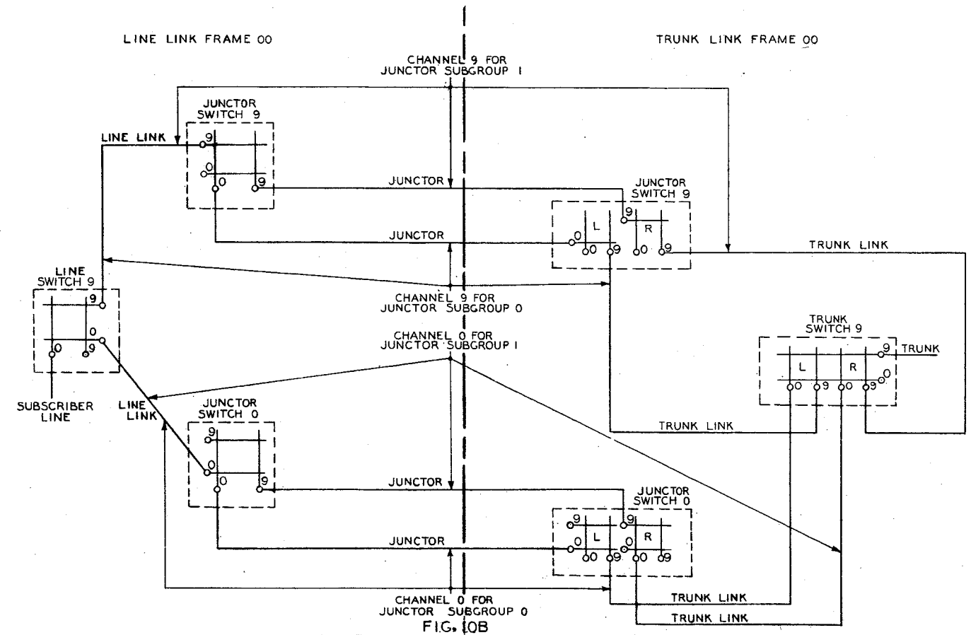
FIG. 10B CHANNELS FOR 10 LINE LINK-5 TRUNK LINK FRAMES
