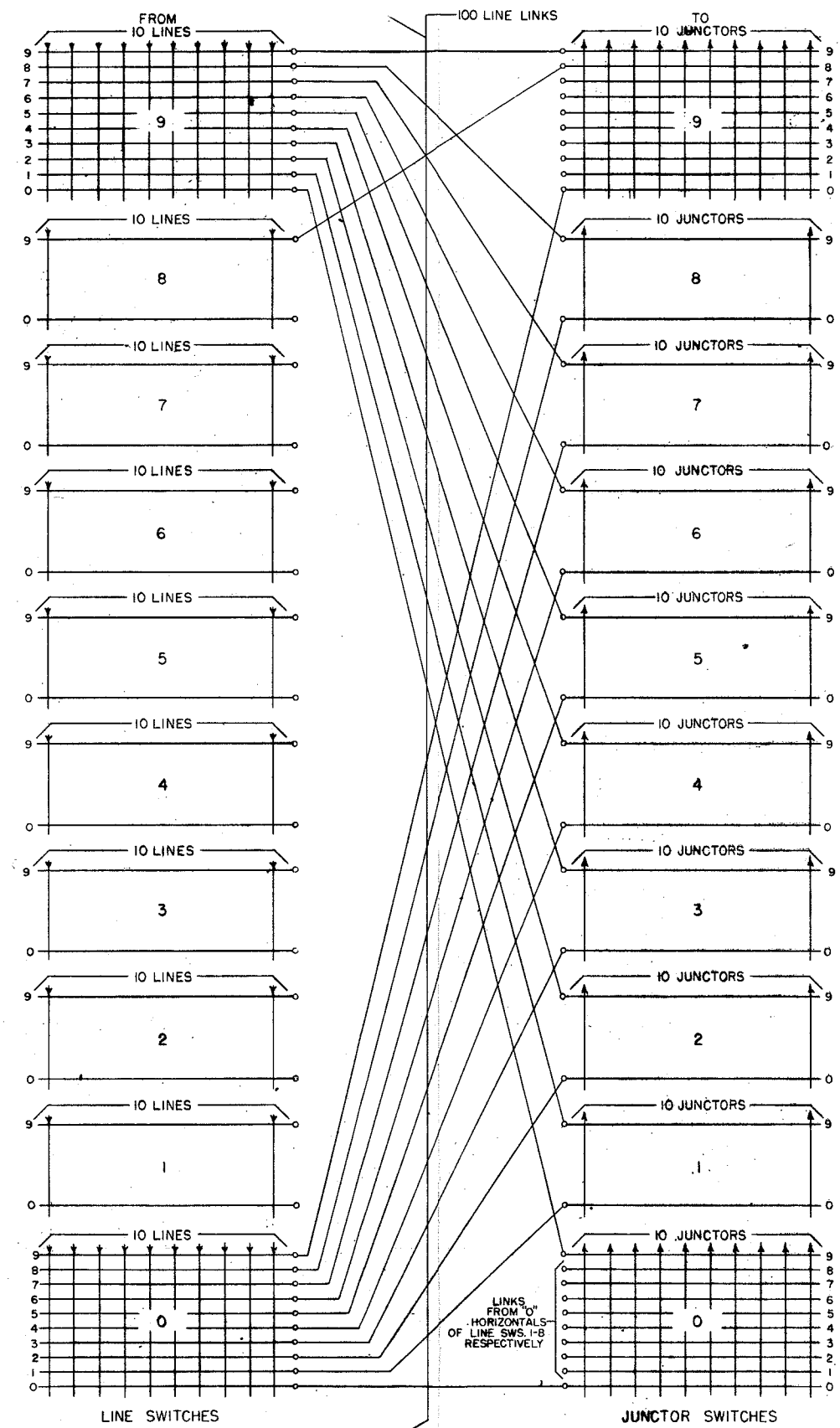
FIG. 4 LINE LINK DISTRIBUTION
