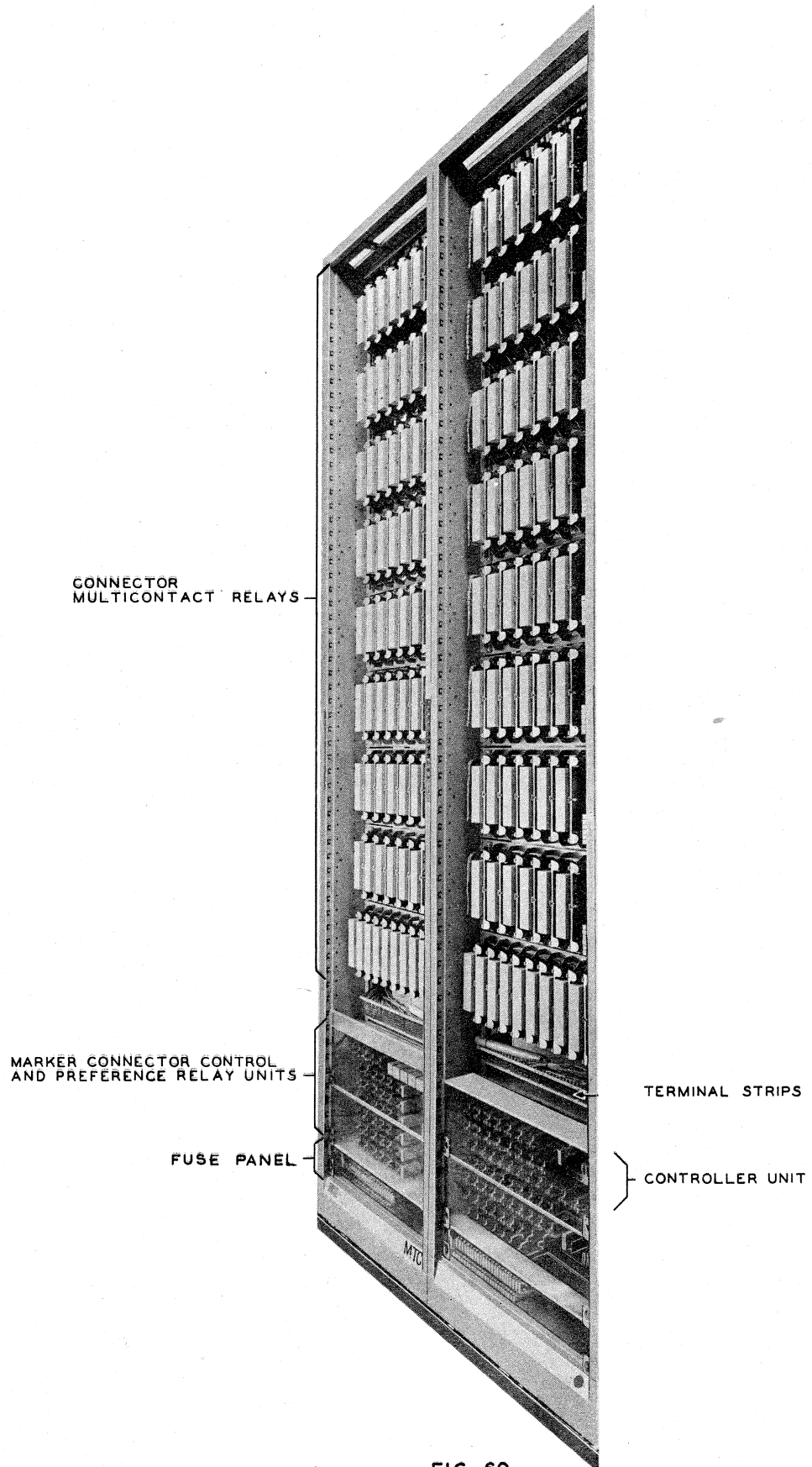
FIG. 60 MASTER TEST CONNECTOR FRAME
