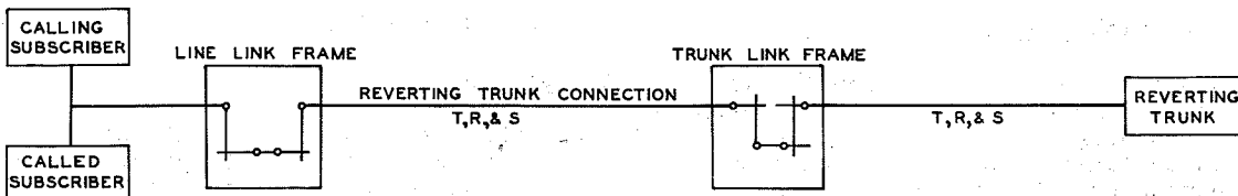
Fig. 34 - Reverting Trunk Connection
