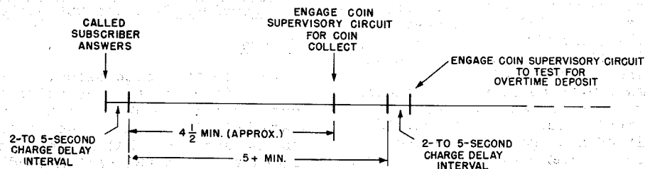
Fig. 45 - Intervals for Coin Operation With Overtime
