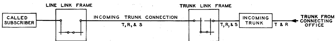
Fig. 36 - Incoming Trunk Connection
