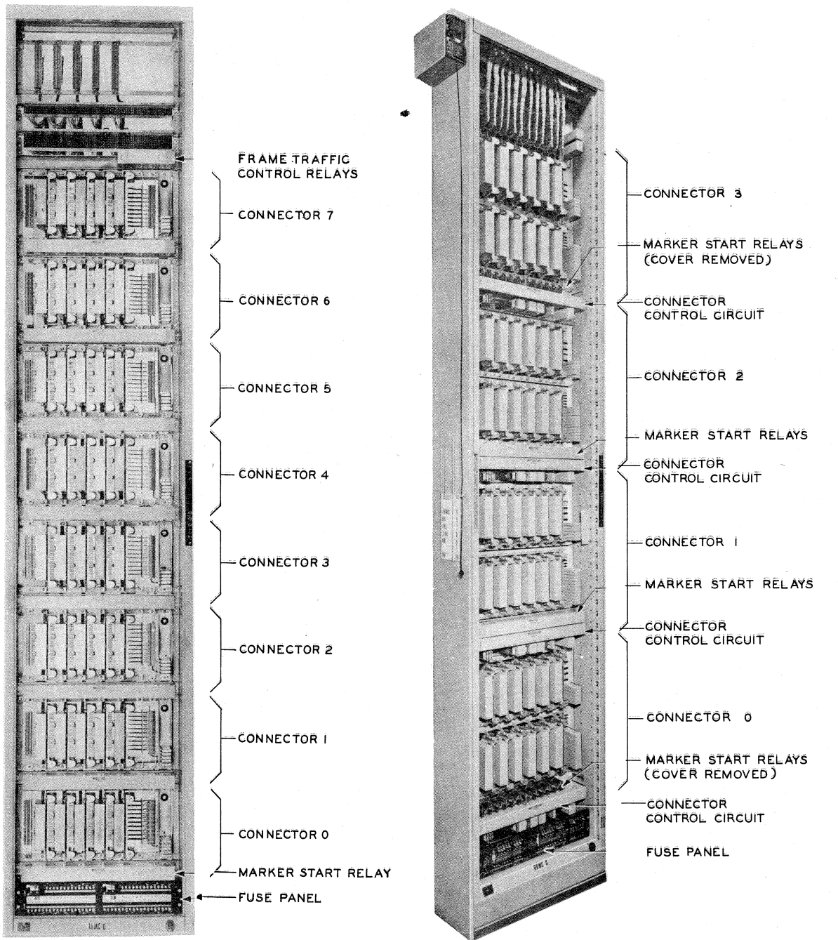
LINE LINK MARKER CONNECTOR
