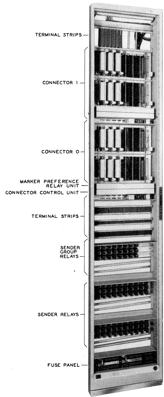
OUTGOING SENDER CONNECTOR
