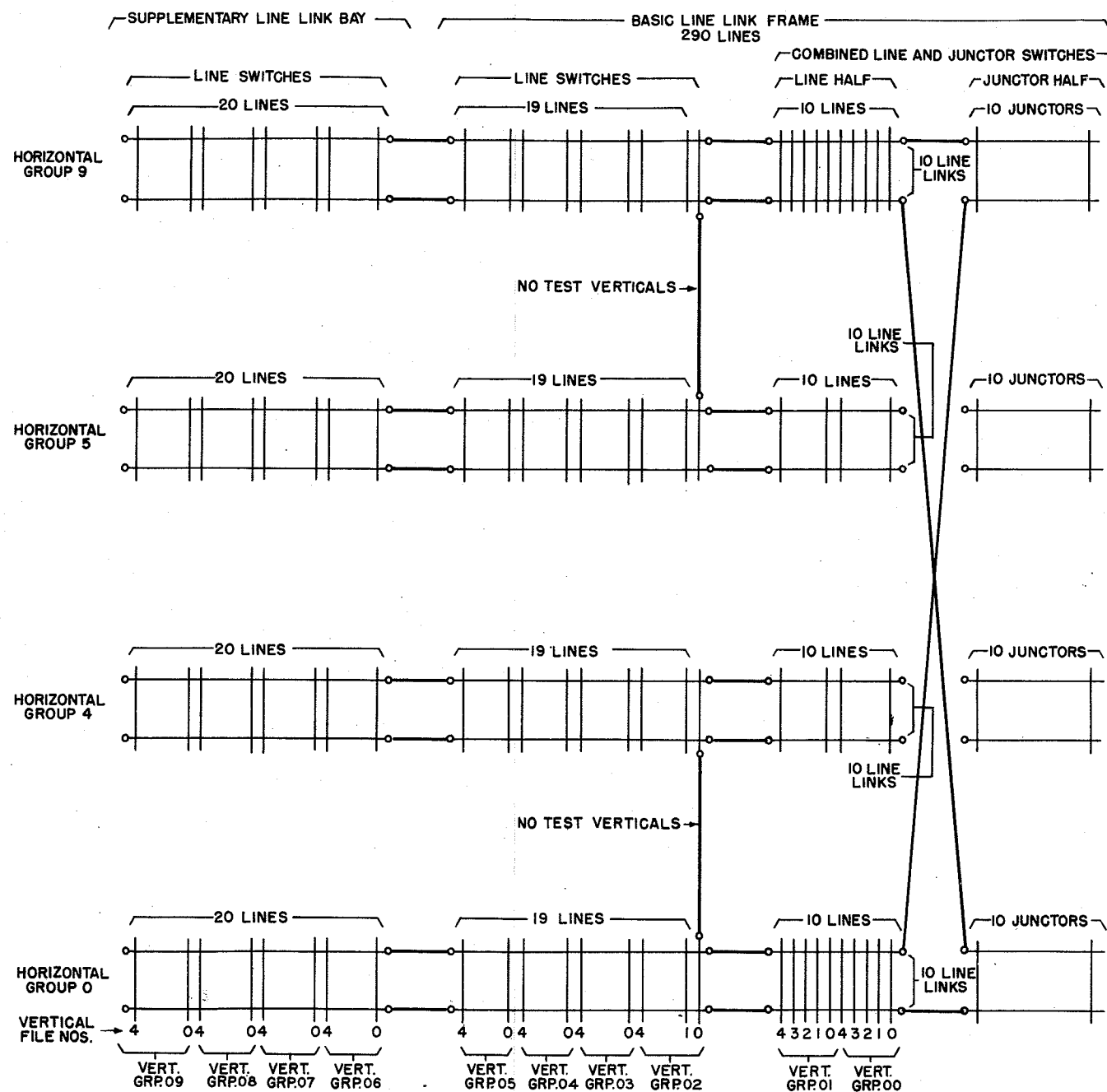
FIG. 38 LINE LINK FRAME SCHEMATIC (WIRING SIDE) FRAME ARRANGED FOR 490 LINES
