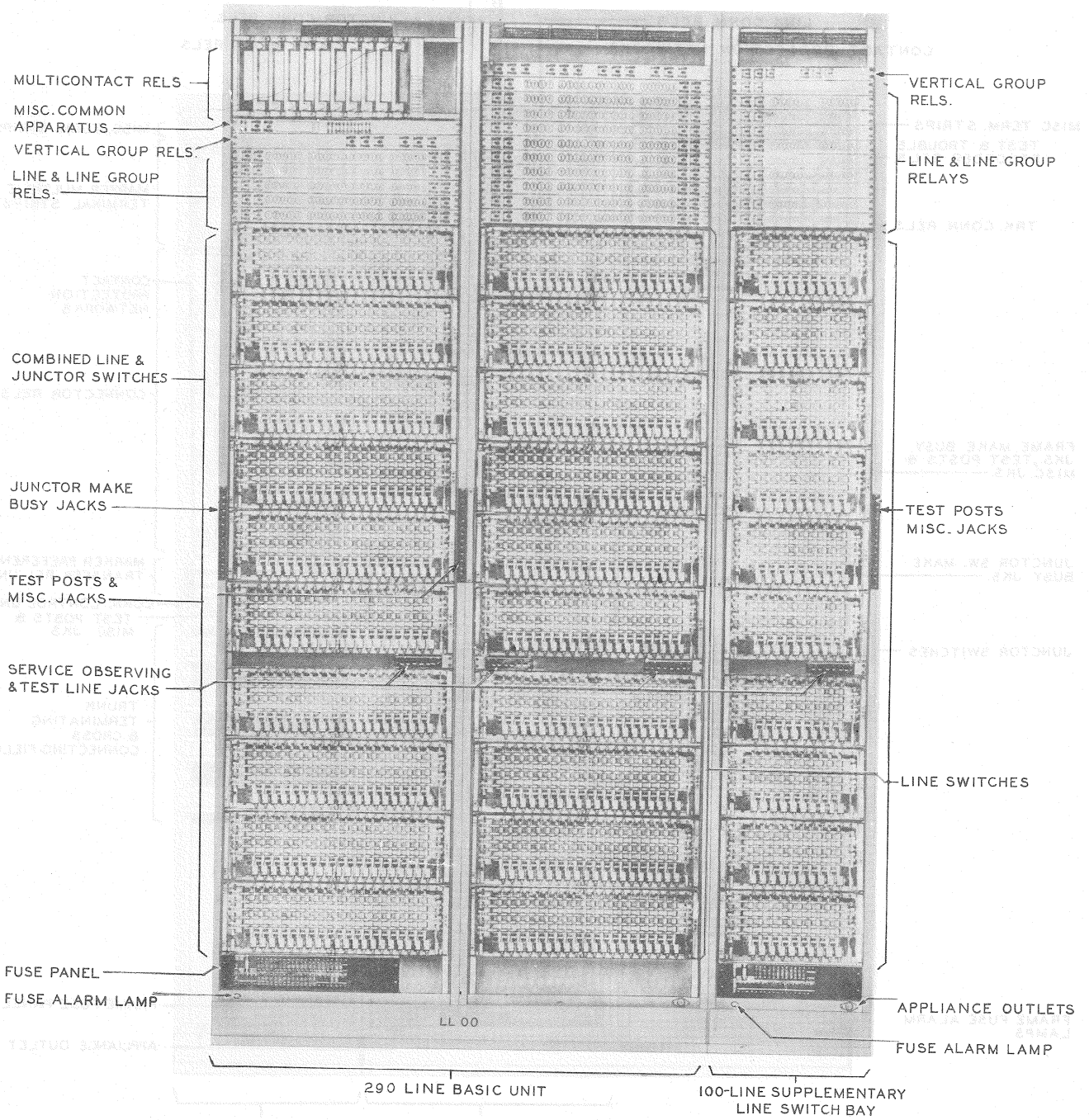
FIG. II LINE LINK FRAME AND SUPPLEMENTARY LINE SWITCH BAY
