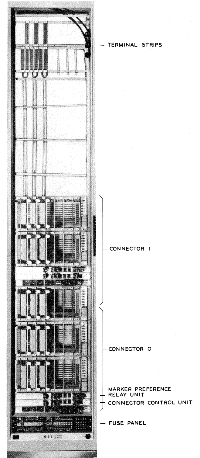
NUMBER GROUP CONNECTOR
