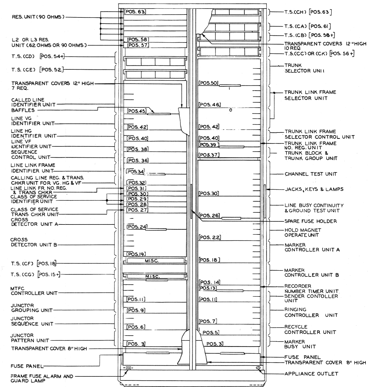
FIG. 14 MARKER FRAME COMMON EQUIPMENT FRAME
