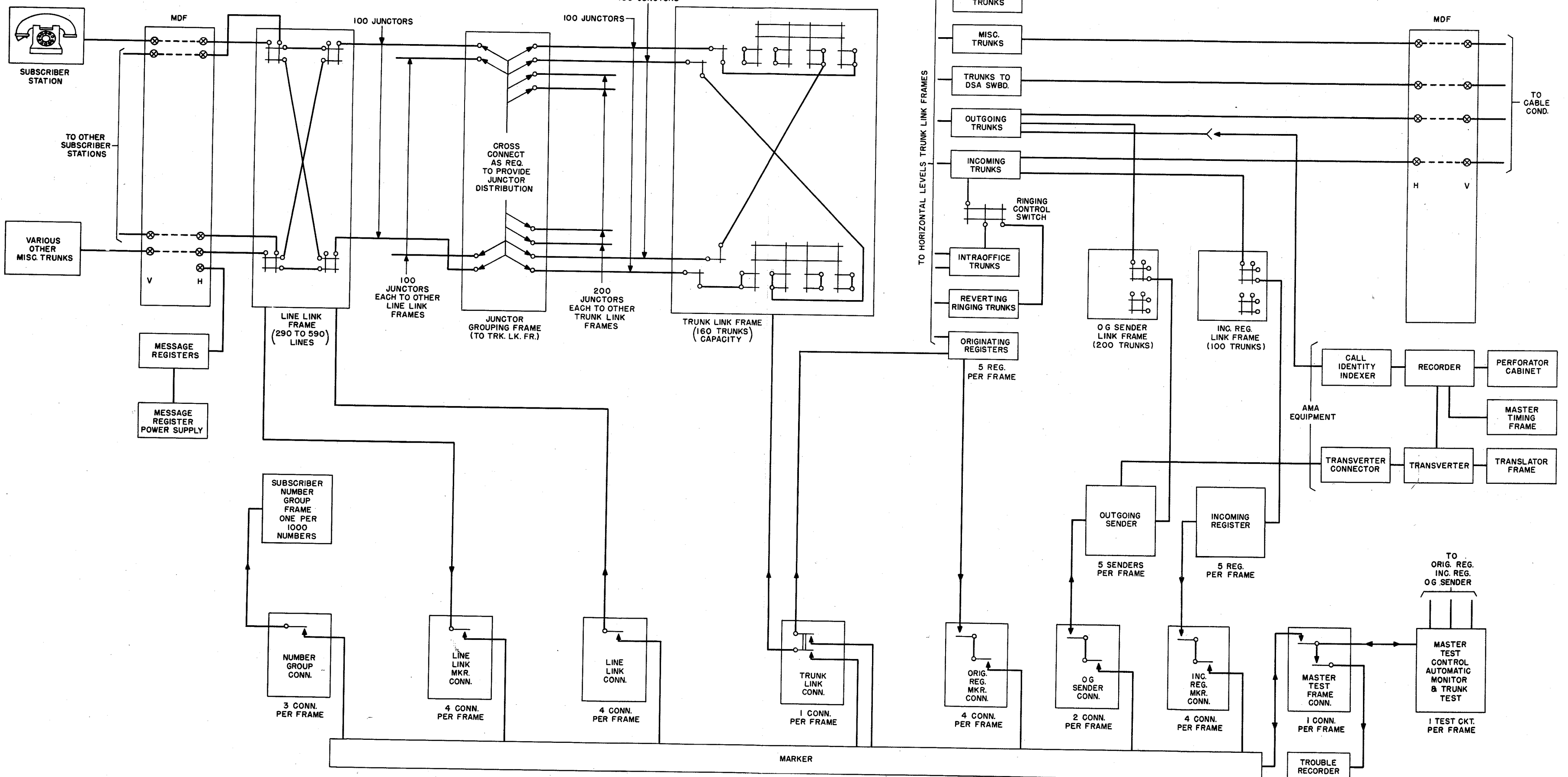
FIG. 2 EQUIPMENT SCHEMATIC OF A NO. 5 CROSSBAR OFFICE
