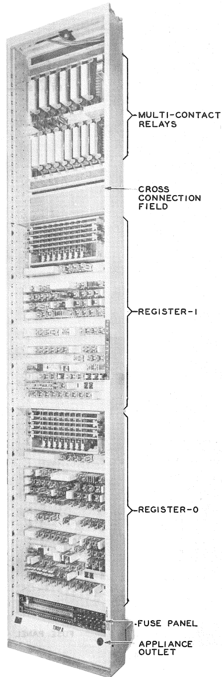
FIG. 25 - TANDEM REVERTIVE PULSE INCOMING REGISTER
