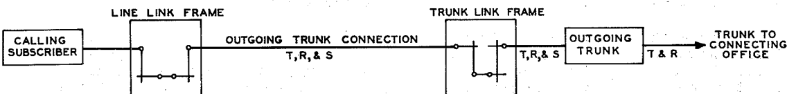
Fig. 35 - Outgoing Trunk Connection
