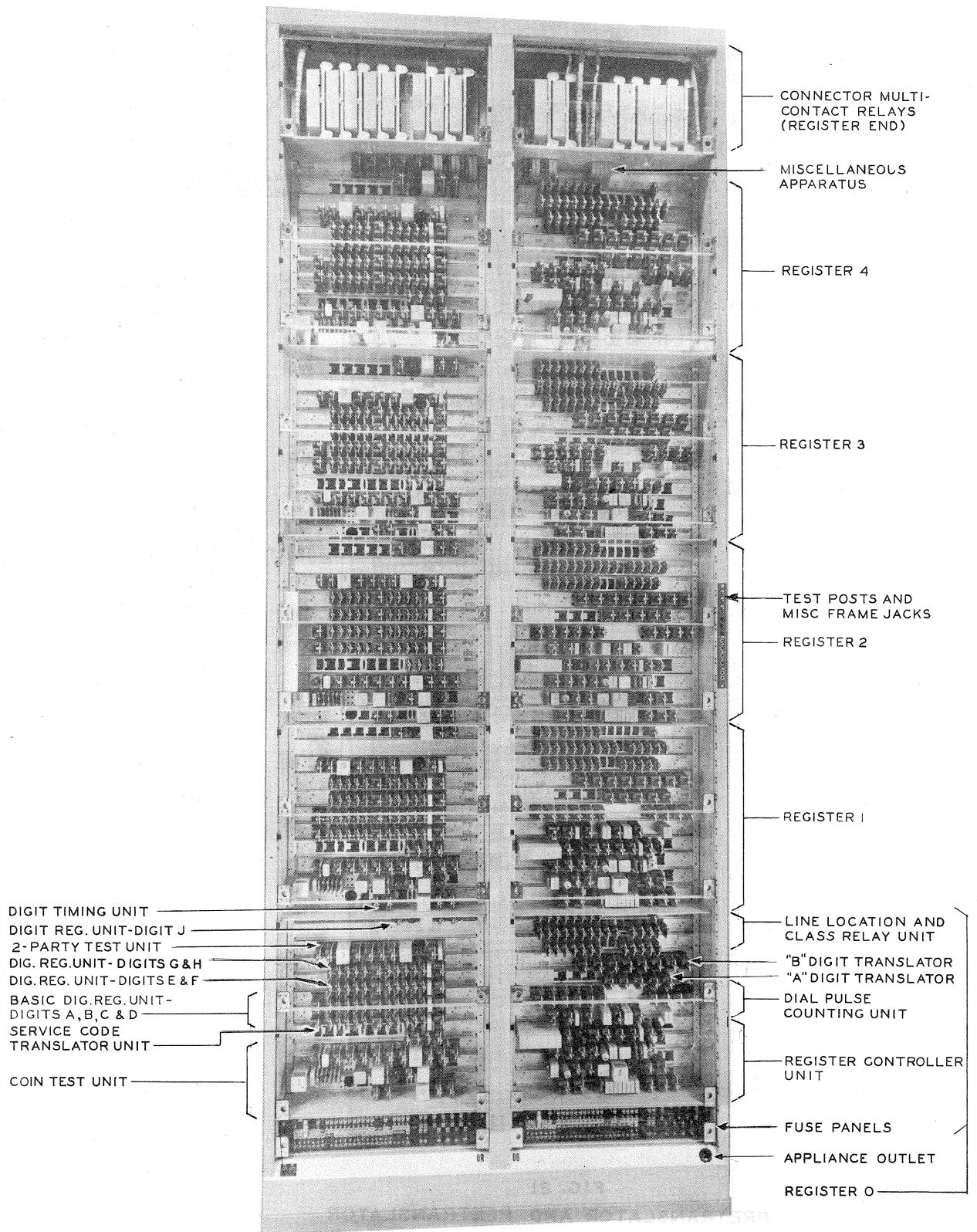
FIG. 20 ORIGINATING REGISTER FRAME
