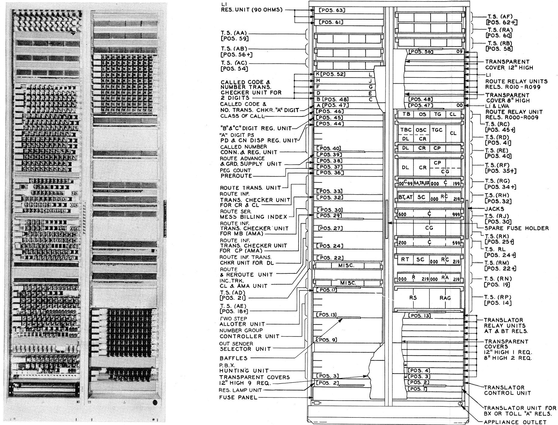
FIG. 15 MARKER FRAME TRANSLATOR AND ROUTE RELAY FRAME
