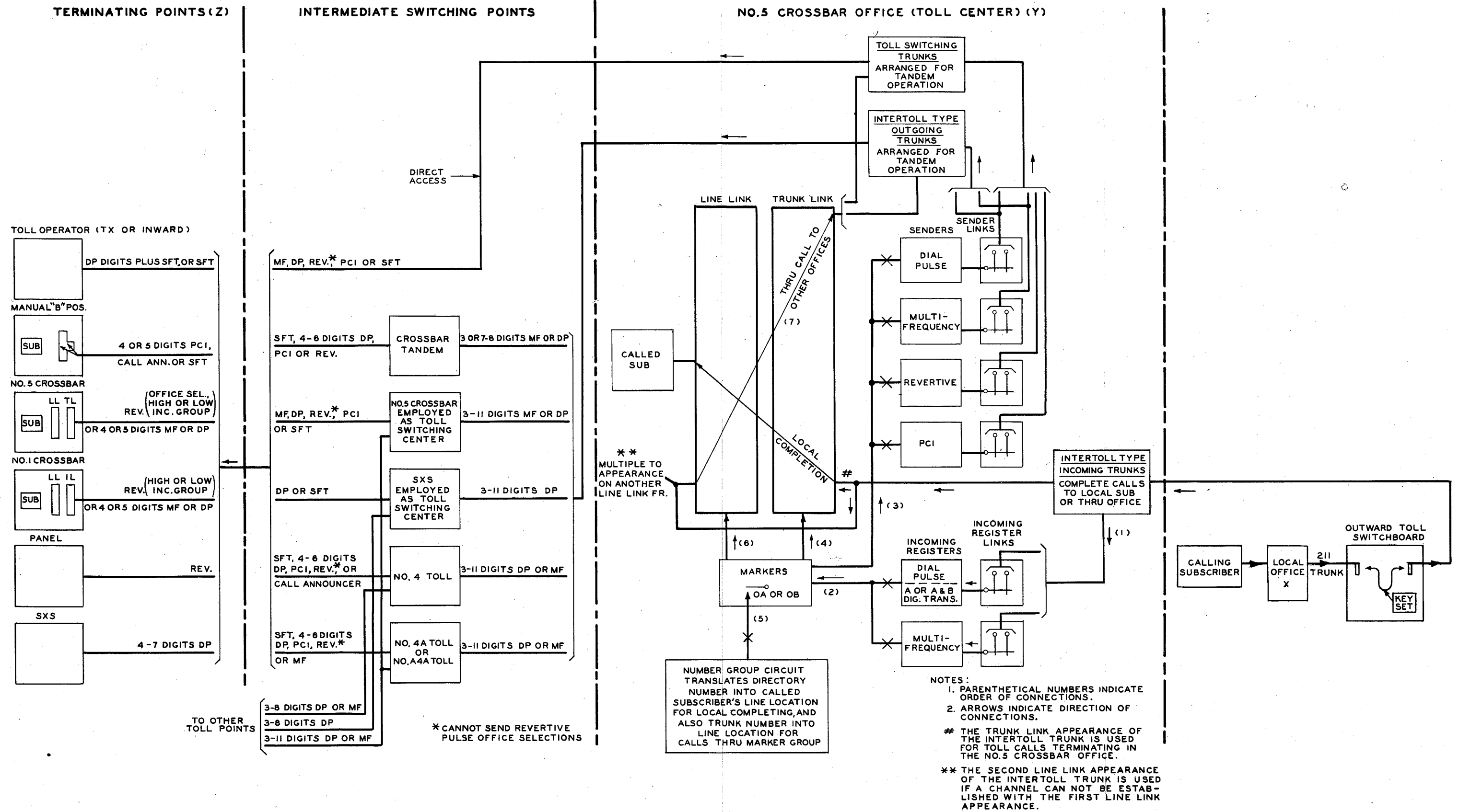
FIG. 51 - TOLL CENTER SWITCHING COMBINED WITH LOCAL COMPLETION TO SUBSCRIBERS IN THE SAME MARKER GROUP
