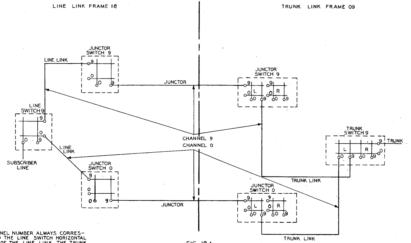
FIG. 10A CHANNELS FOR 20 LINE LINK-10 TRUNK LINK FRAMES
