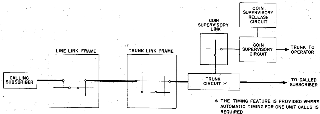
Fig. 44 - Association of Coin Trunk and Coin Supervisory Link
