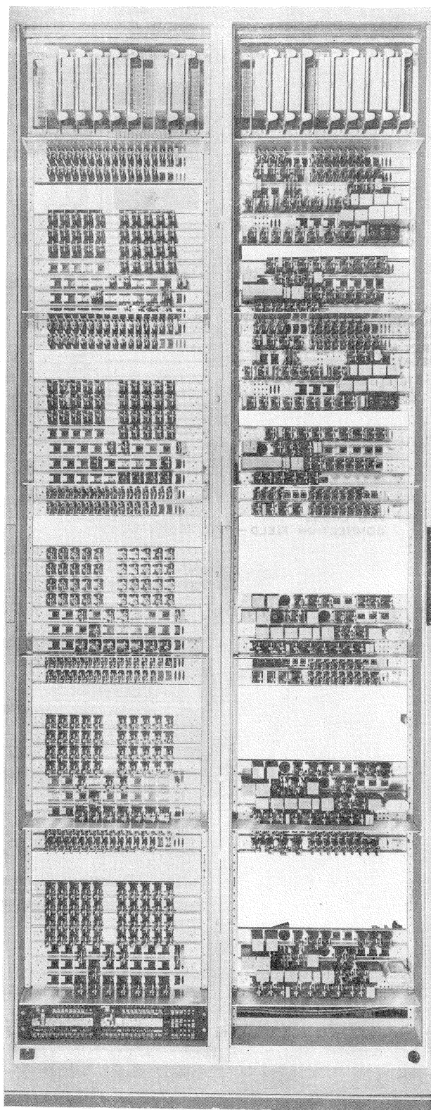
FIG. 23 OUTGOING SENDER FRAME
