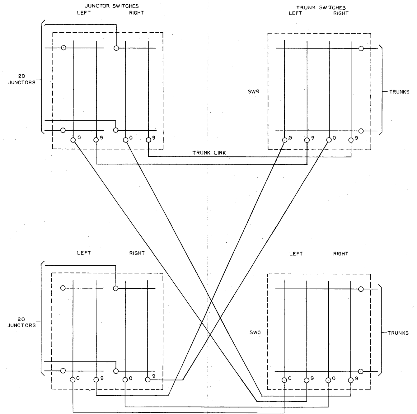
FIG. 8 TRUNK LINK DISTRIBUTION
