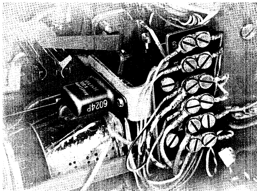
Fig. 5 - FW (4-Wire) Relay and Auxiliary Terminal Strip
