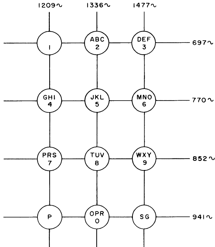
Fig. 3 - Dial Frequencies
