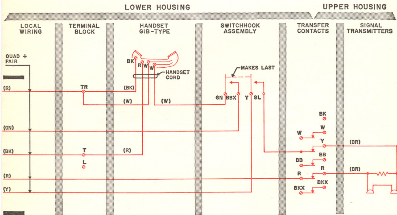
Fig. 1 — Circuit Diagram for Connecting 182CN, DN and 200C, D Coin Collectors When Used With a 685A Network-type Subscriber Set
